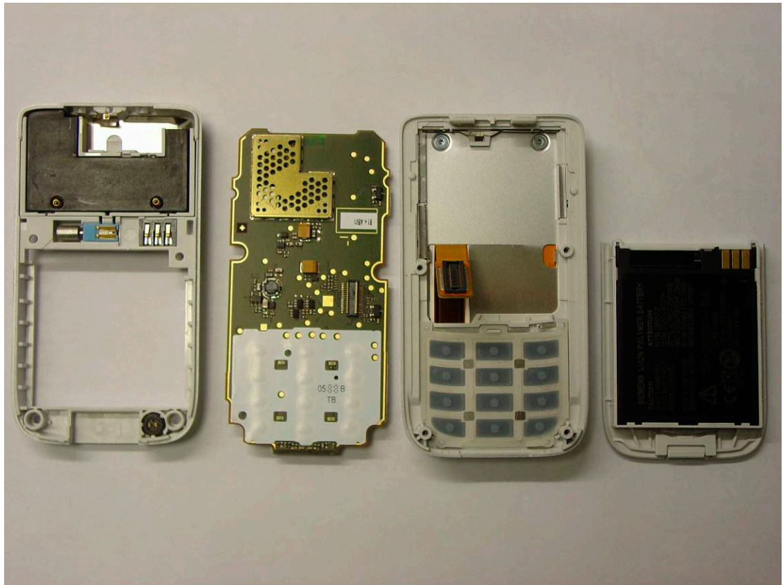
CF110 Disassembly Step 2
