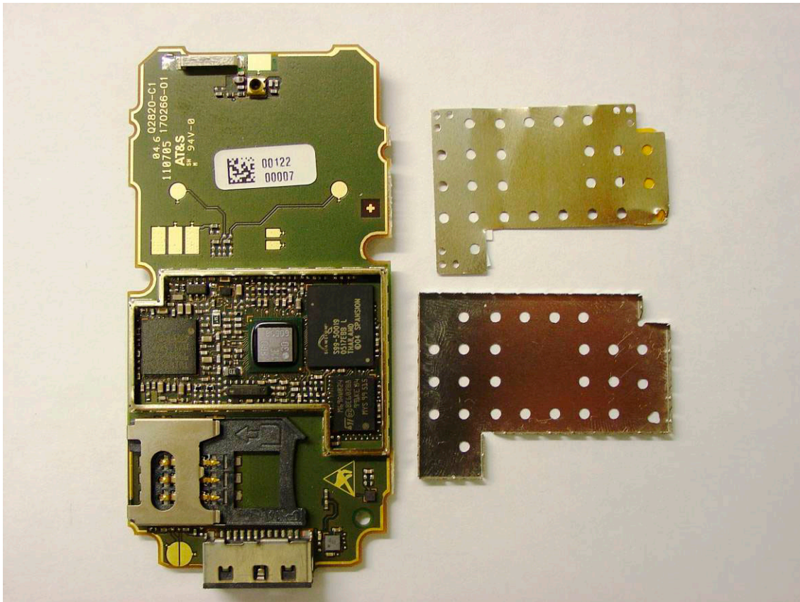
CF110 Back view BB (rep. Lid)
