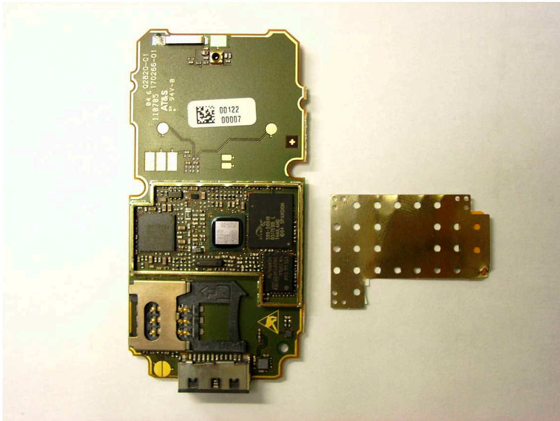
CF110 PCB Back View Shields Removed
