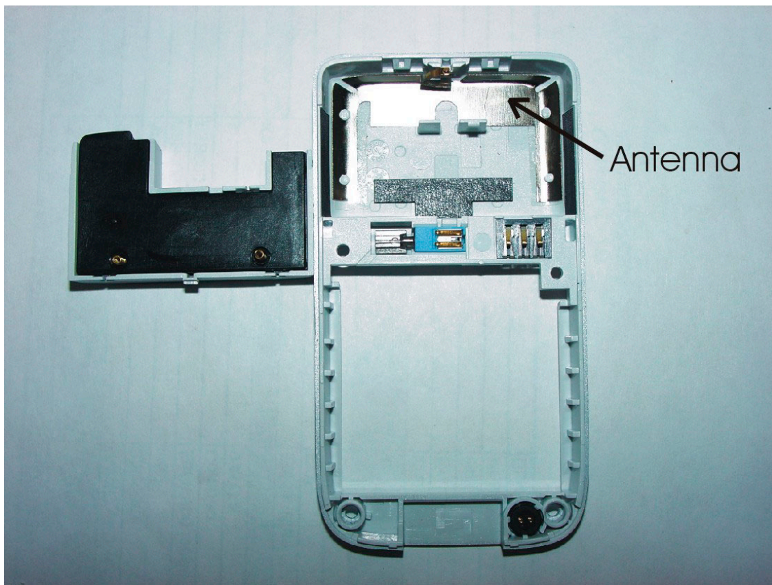
CF110 Antenna
