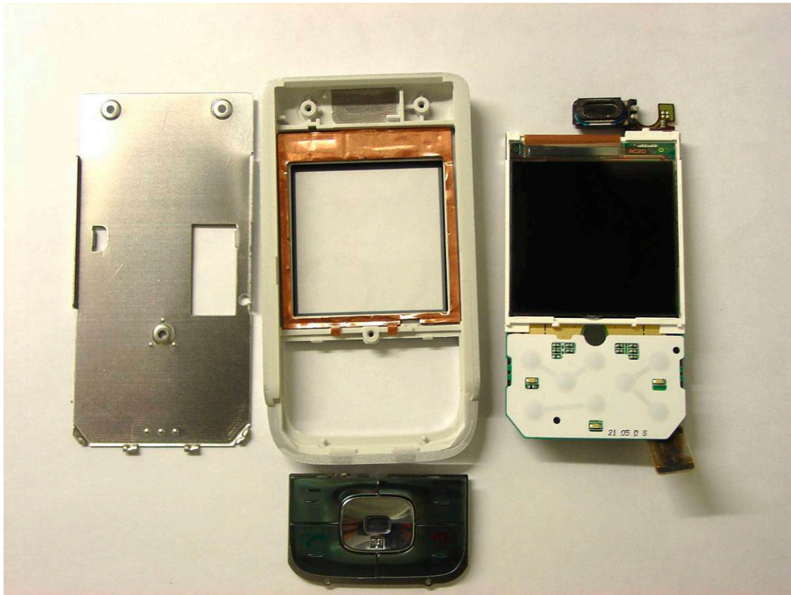
CF110 Disassembly Step 5
