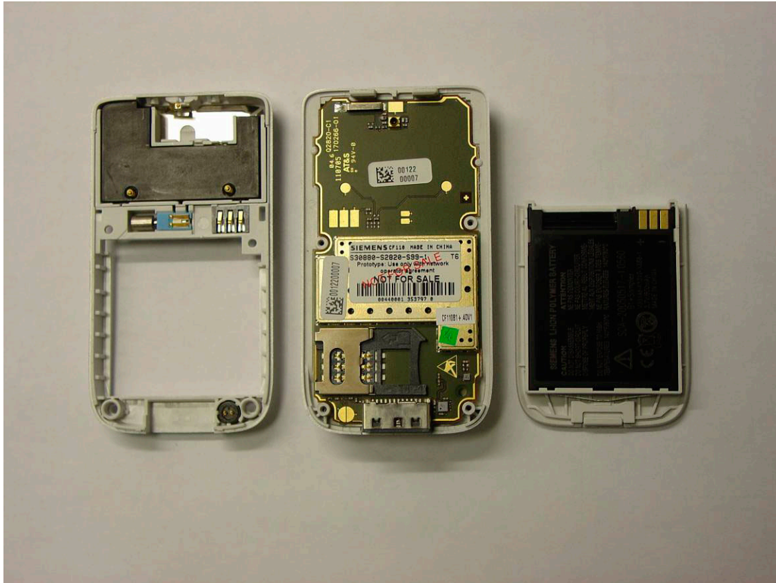
CF110 Disassembly Step 1
