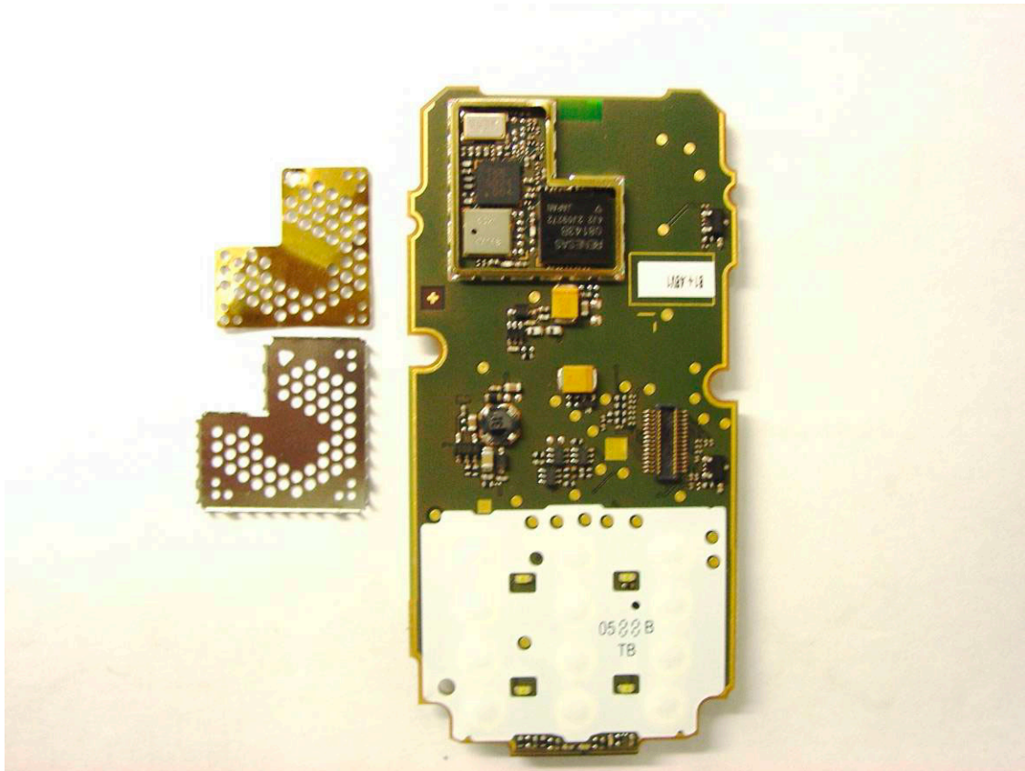
CF110 Front view RF
