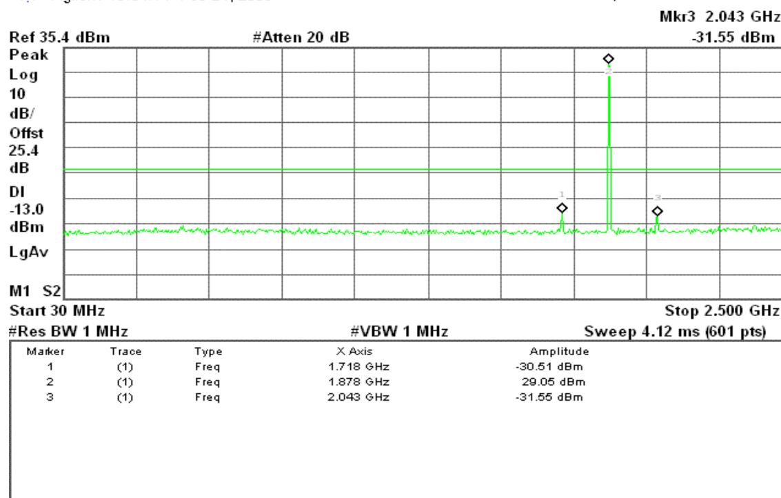
Figure 7-10: Out of Band emission at antenna terminals –GPRS CH Mid
