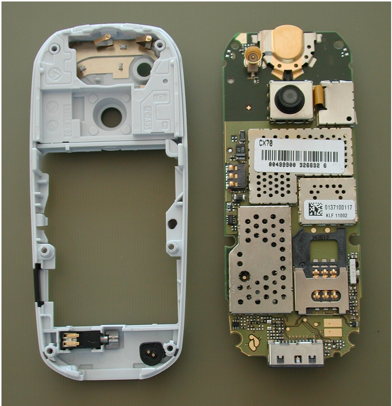
CX70 Disassembly Step 2
