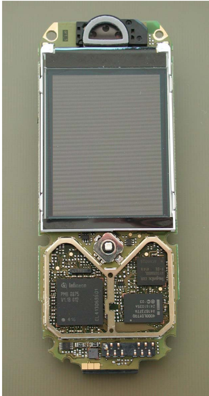
CX70 PCB Front View Shields Removed
