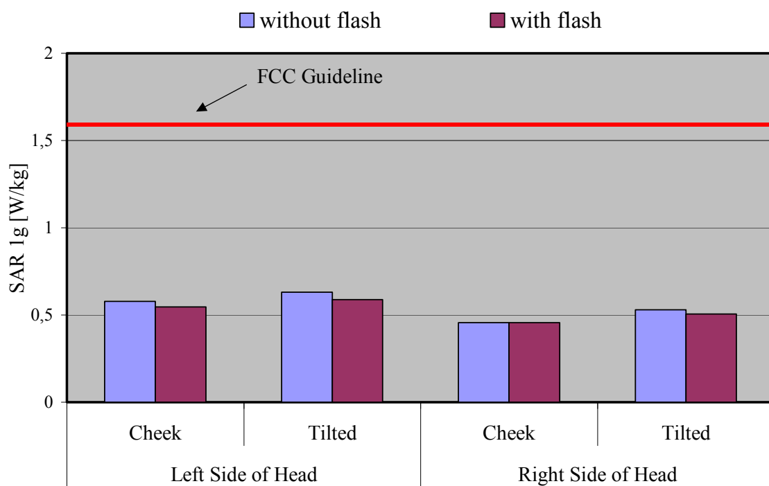
Fig. 8: The measured head phantom SAR values for the Siemens CX70 Standard for PCS 1900 in comparison to the FCC exposure limit.
