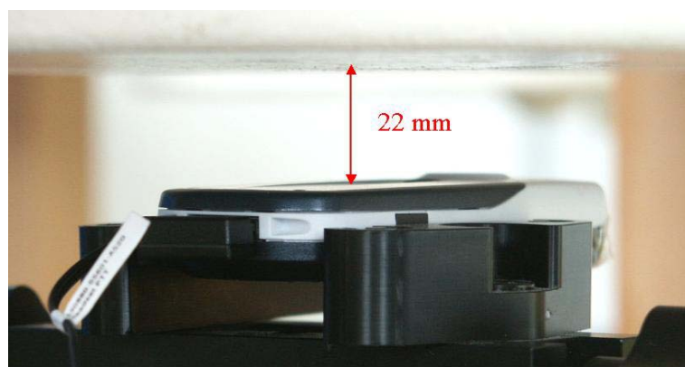
Fig. 46: Body worn configuration Standard, GSM mode with headset, antenna towards the phantom.
