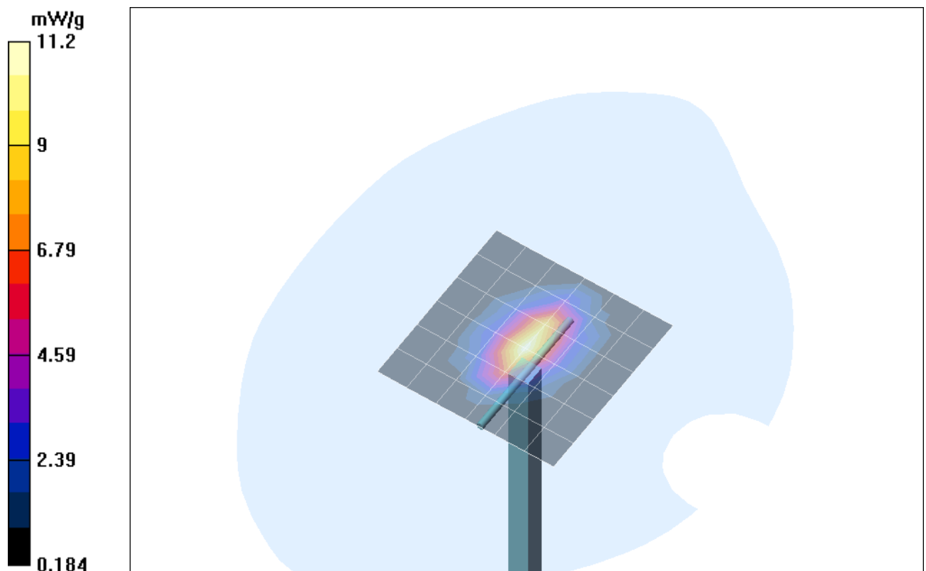
Fig. 12: Validation measurement 1900 MHz Head (October 21, 2004), coarse grid. Ambient Temperature: 22.0° C, Liquid Temperature: 20.8° C.
