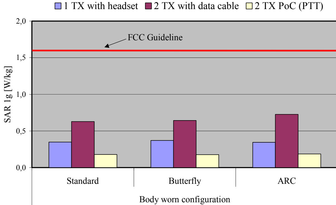
Fig. 11: The measured SAR values in body-worn configuration for the Siemens CX70 for PCS 1900 in comparison to the FCC exposure limit.
