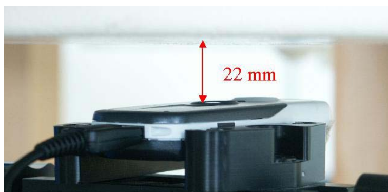
Fig. 50: Body worn configuration CX70 Butterfly, GPRS mode (Class 10) with data cable, antenna towards the phantom.
