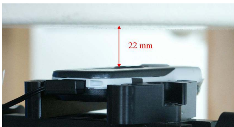
Fig. 47: Body worn configuration Butterfly, GSM mode with headset, antenna towards the phantom.
