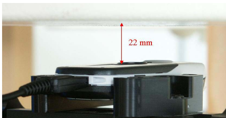
Fig. 51: Body worn configuration CX70 ARC, GPRS mode (Class 10) with data cable, antenna towards the phantom
