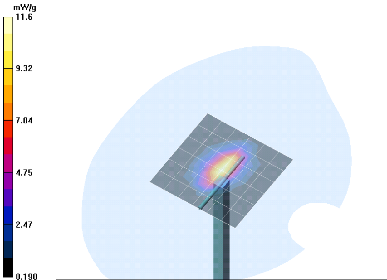
Fig. 13: Validation measurement 1900 MHz body (October 29, 2004), coarse grid. Ambient Temperature: 22.2° C, Liquid Temperature: 20.7° C.
