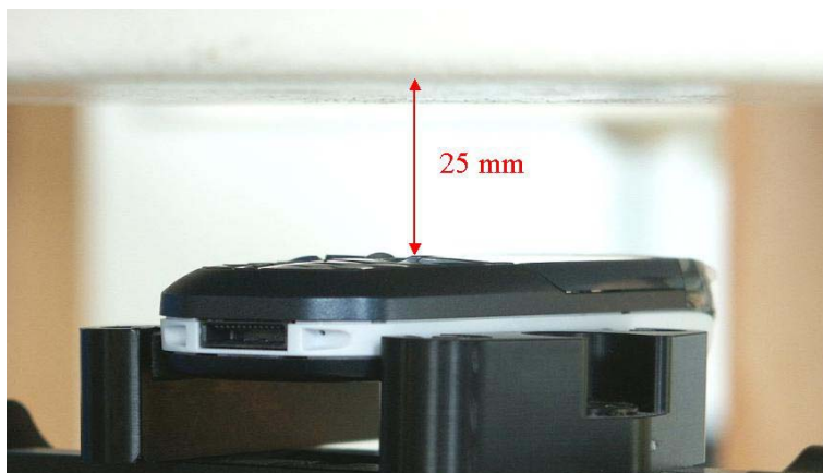
Fig. 52: Body worn configuration CX70 Standard, PTT GPRS mode (Class 10), display towards the phantom.
