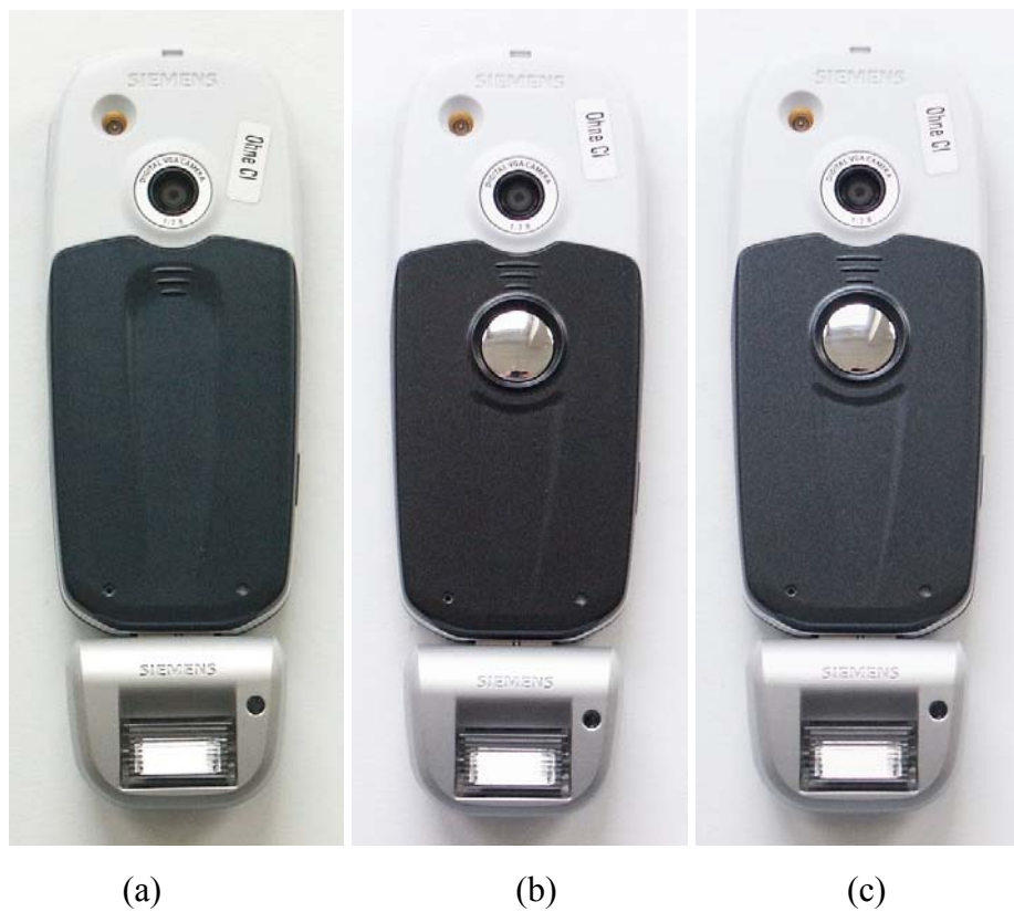
Fig. 19: Picture of the device under test, Backside (a Standard; b Butterfly; c ARC).
