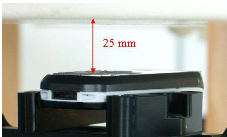
Fig. 54: Body worn configuration CX70 ARC, PTT GPRS mode (Class 10), display towards the phantom.
