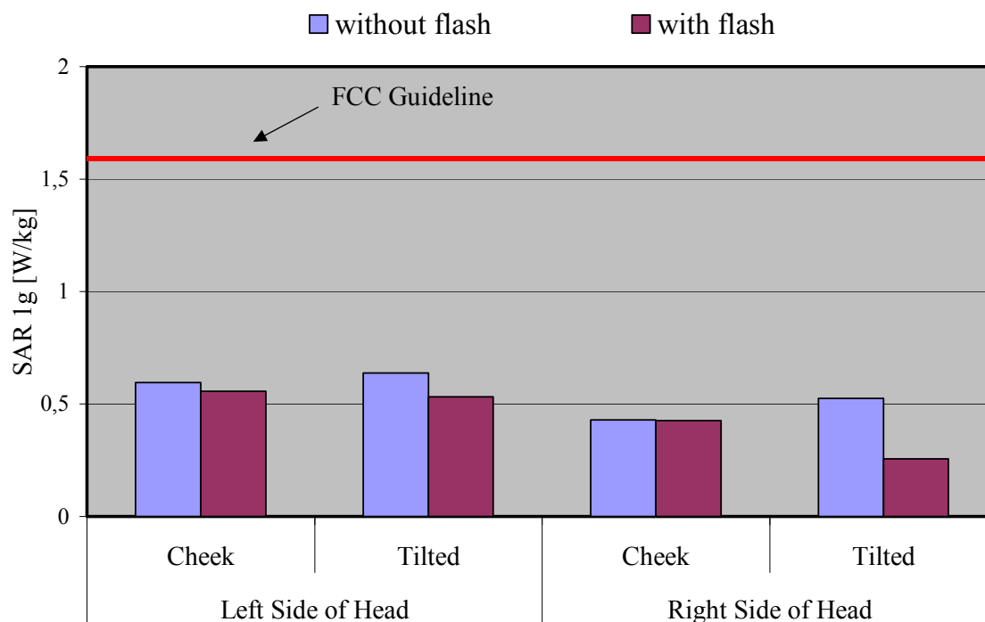
Fig. 9: The measured head phantom SAR values for the Siemens CX70 Butterfly for PCS 1900 in comparison to the FCC exposure limit.
