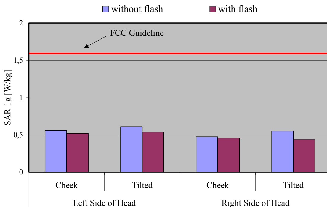
Fig. 10: The measured head phantom SAR values for the Siemens CX70 ARC for PCS 1900 in comparison to the FCC exposure limit.
