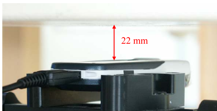
Fig. 49: Body worn configuration CX70 Standard, GPRS mode (Class 10) with data cable, antenna towards the phantom.
