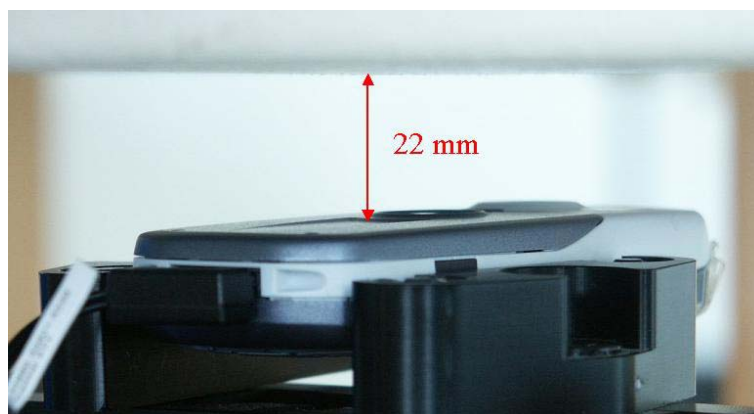
Fig. 48: Body worn configuration ARC, GSM mode with headset, antenna towards the phantom.
