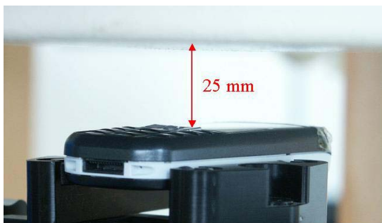
Fig. 53: Body worn configuration CX70 Butterfly, PTT GPRS mode (Class 10), display towards the phantom.
