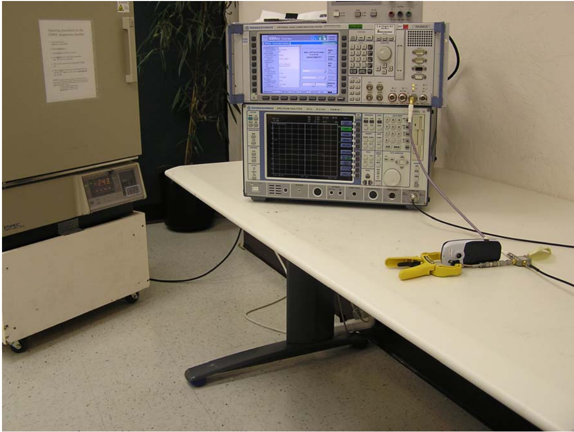
Test setup – RF conducted measurements
