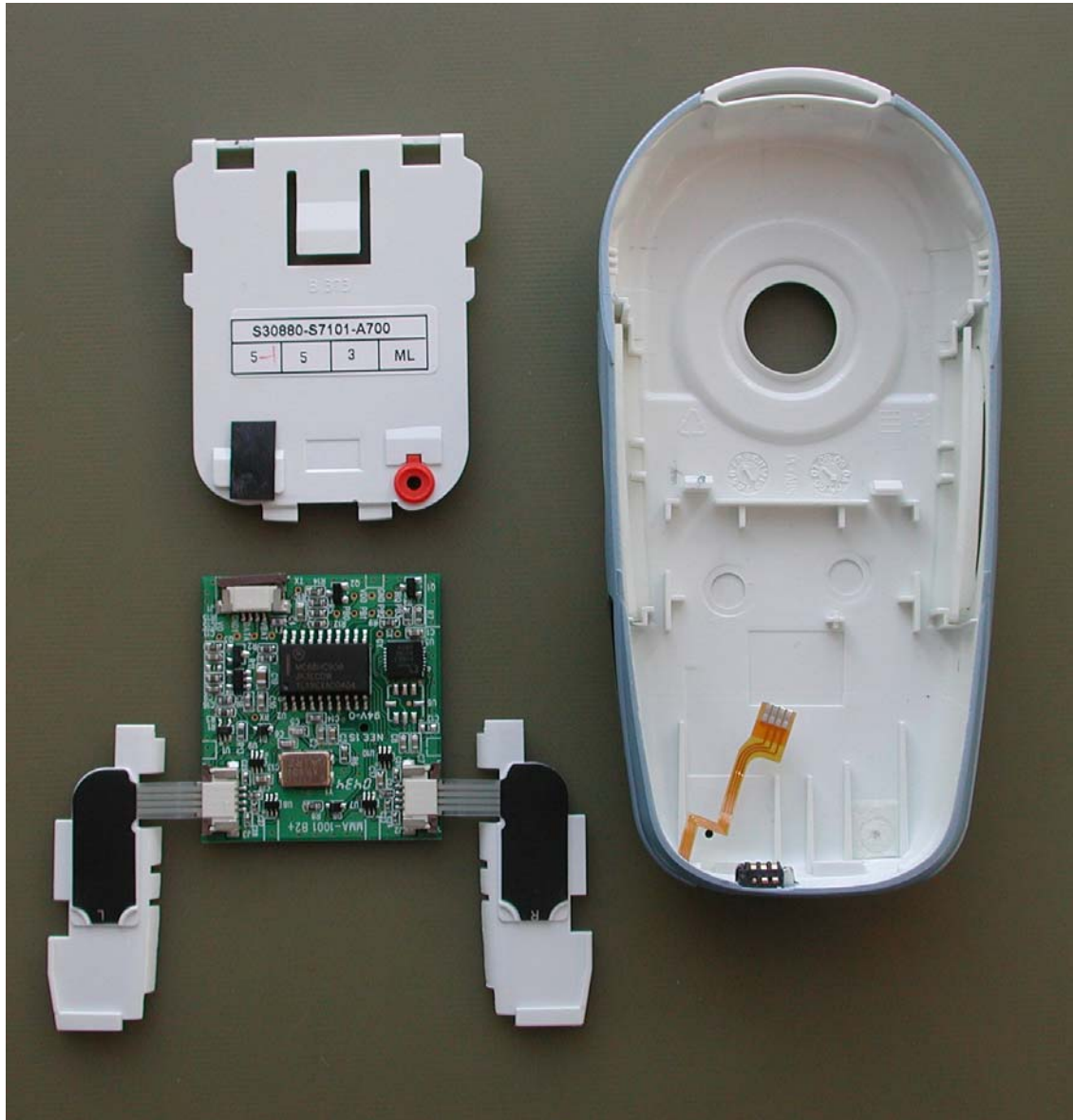
CX70E Disassembly Step 3
