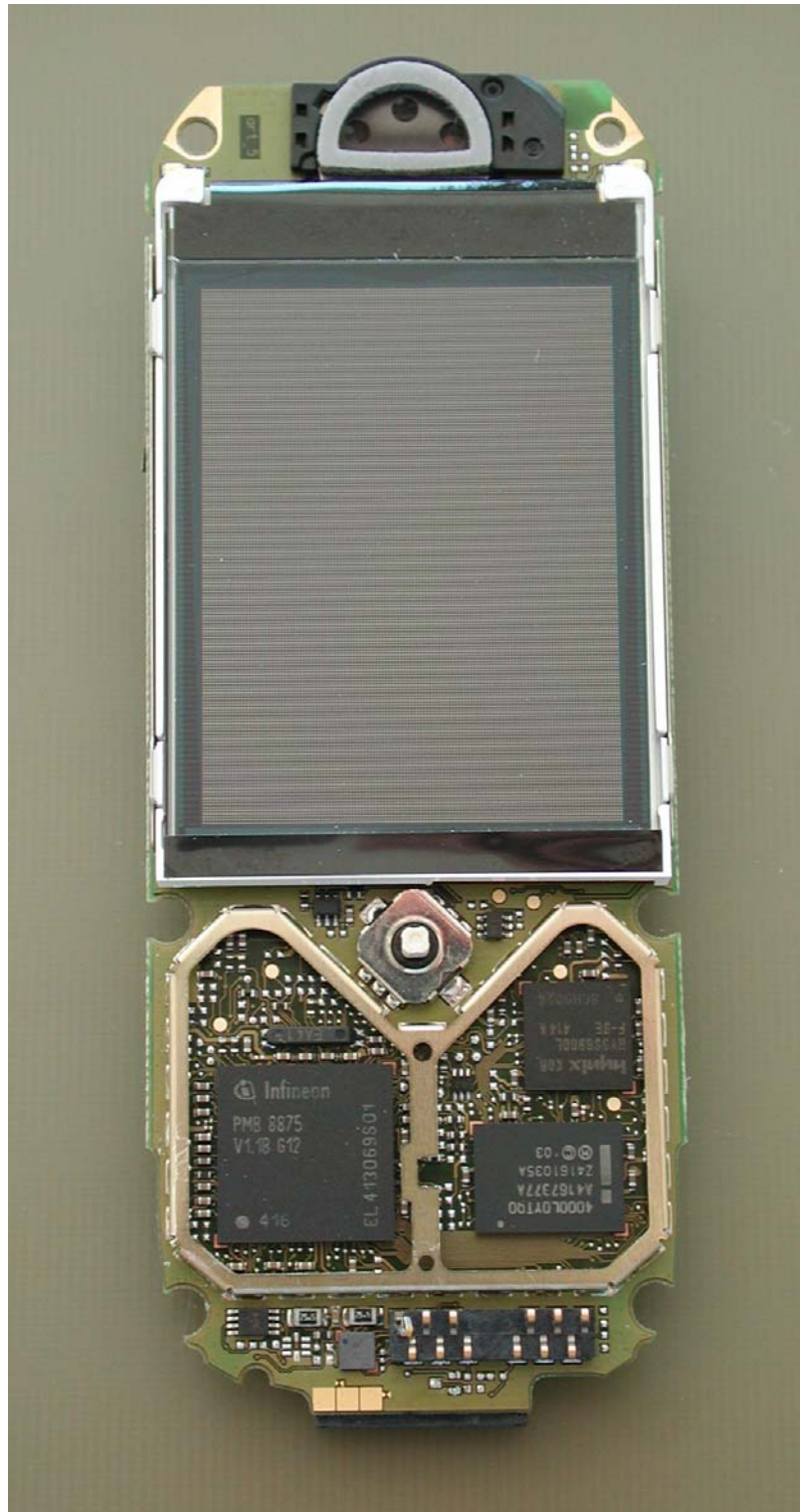
CX70E PCB Front View Shields Removed
