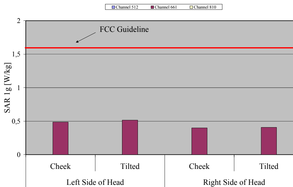
Fig. 11: The measured head phantom SAR values for the Siemens CX70E Active with Flash for PCS 1900 in comparison to the FCC exposure limit.
