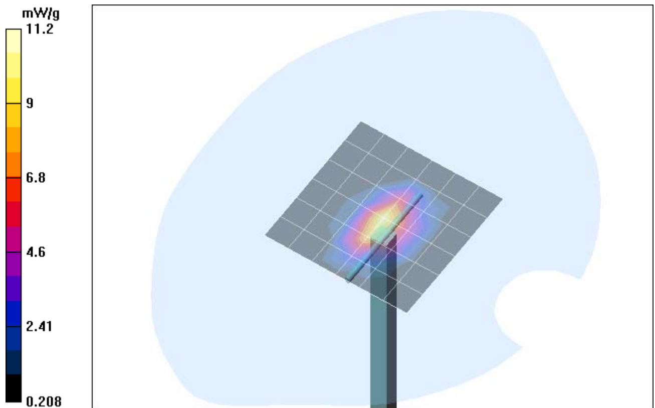
Fig. 14: Validation measurement 1900 MHz Head (September 16, 2004), coarse grid. Ambient Temperature: 20.6° C, Liquid Temperature: 19.9° C.
