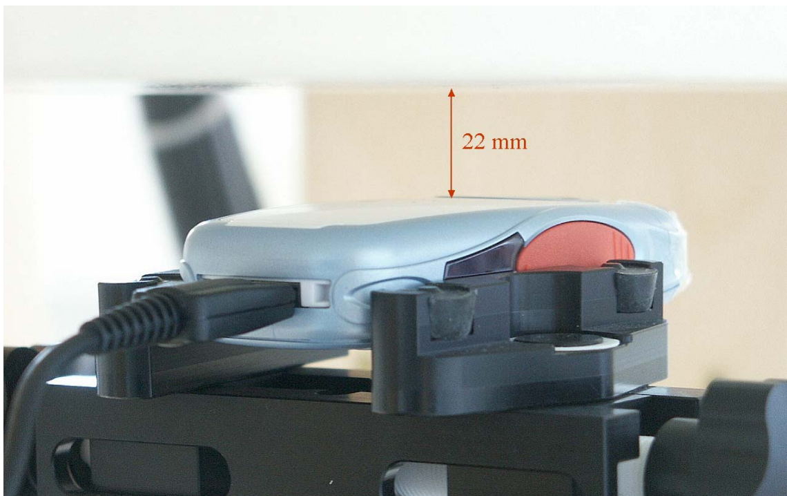
Fig. 42: Body worn configuration CX70E Active, GPRS mode (2 TX slots) with data cable, antenna towards the phantom.
