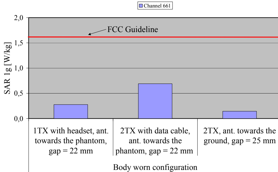
Fig. 12: The measured SAR values in body-worn configuration for the Siemens CX70E ARC for PCS 1900 in comparison to the FCC exposure limit.
