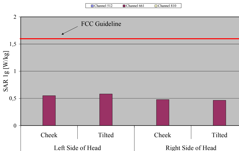
Fig. 9: The measured head phantom SAR values for the Siemens CX70E Active for PCS 1900 in comparison to the FCC exposure limit.
