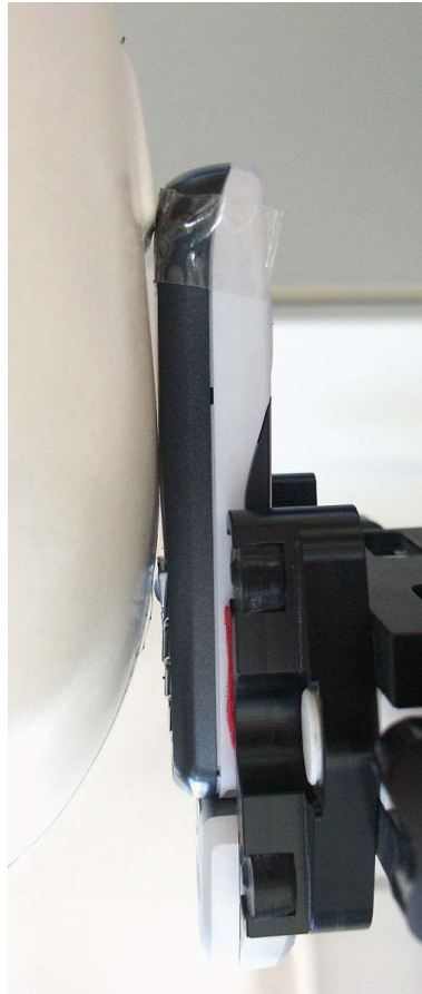
Fig. 31: Cheek position, left side, ARC.
