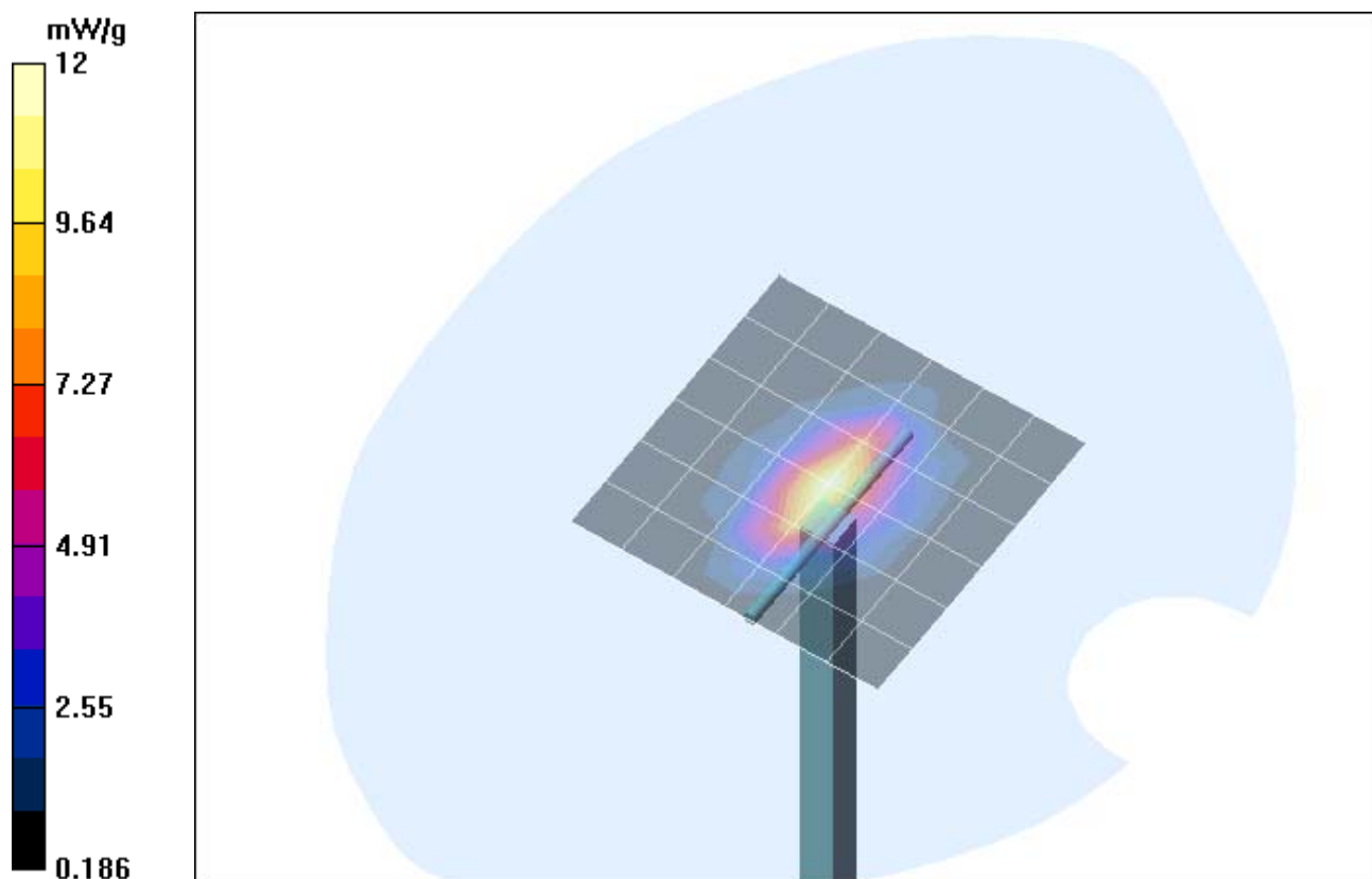
Fig. 15: Validation measurement 1900 MHz body (September 13, 2004), coarse grid. Ambient Temperature: 20.9° C, Liquid Temperature: 20.4° C.
