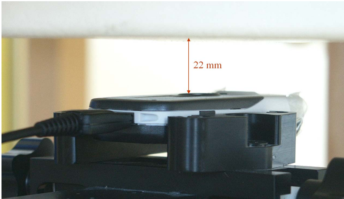
Fig. 41: Body worn configuration CX70E ARC, GPRS mode (2 TX slots) with data cable, antenna towards the phantom.
