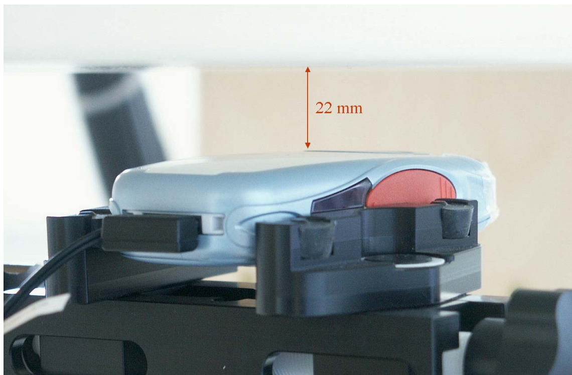
Fig. 40: Body worn configuration CX70E Active, GSM mode (1 TX slot) with headset, antenna towards the phantom.
