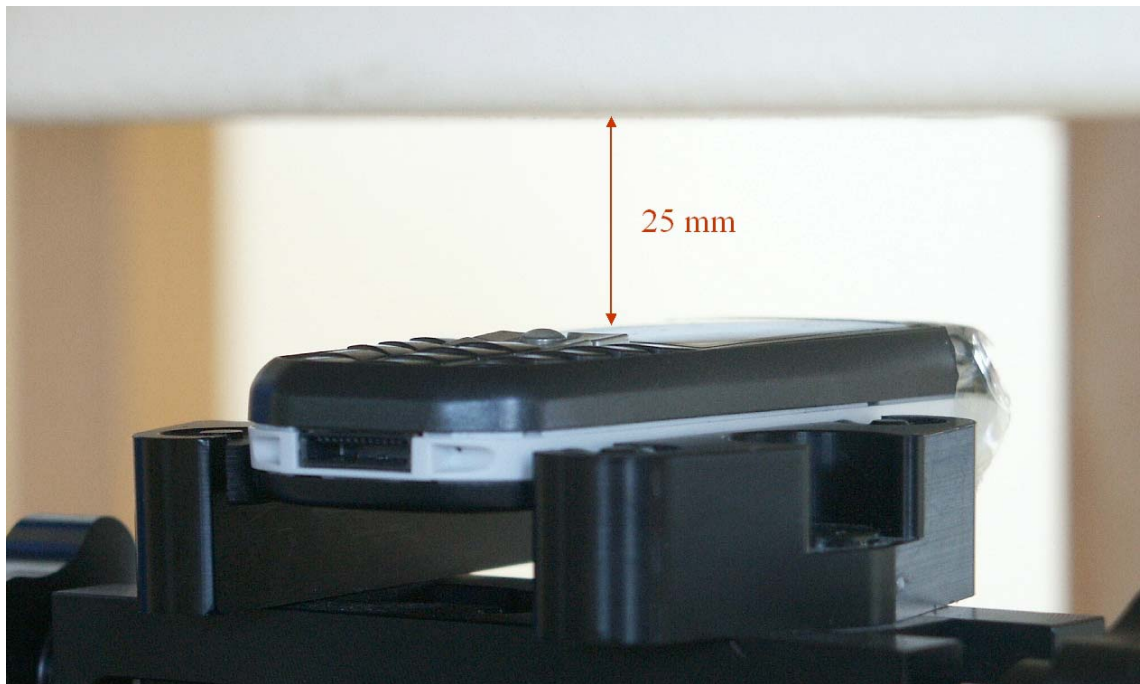
Fig. 43: Body worn configuration CX70E ARC, PTT GPRS mode (2 TX slots), antenna towards the ground.
