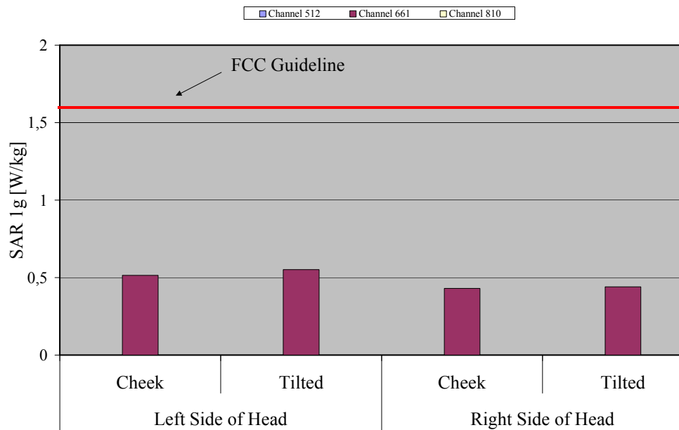
Fig. 10: The measured head phantom SAR values for the Siemens CX70E ARC with Flash for PCS 1900 in comparison to the FCC exposure limit.
