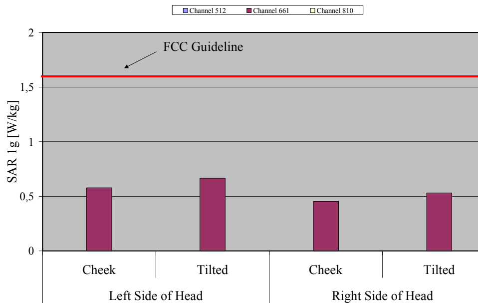
Fig. 8: The measured head phantom SAR values for the Siemens CX70E ARC for PCS 1900 in comparison to the FCC exposure limit.
