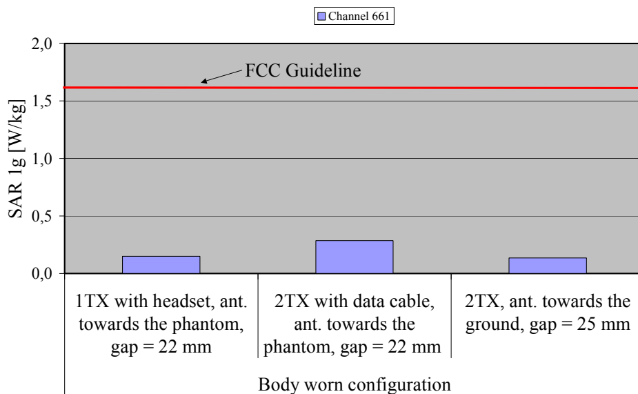
Fig. 13: The measured SAR values in body-worn configuration for the Siemens CX70E Active for PCS 1900 in comparison to the FCC exposure limit.
