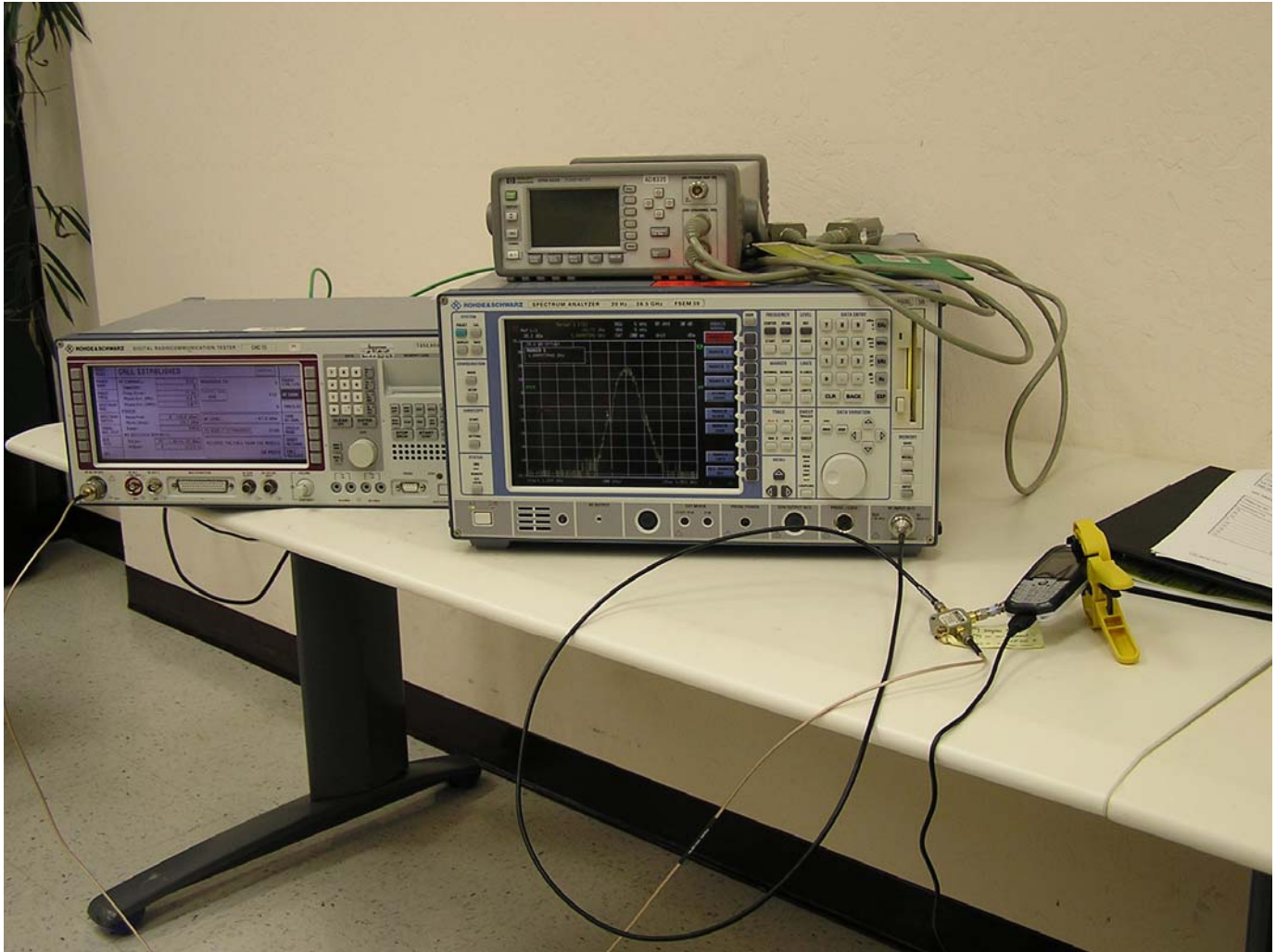
Test setup – RF conducted measurements (test sample is not in CX70E plastic housing)
