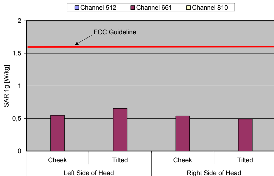
Fig. 9: The measured head phantom SAR values for the Siemens CX75 with flash for PCS 1900 in comparison to the FCC exposure limit.
