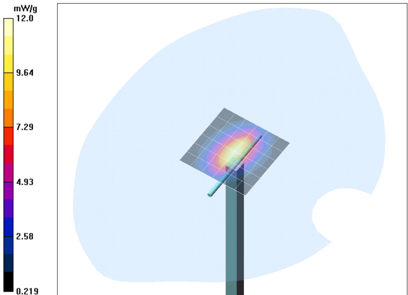
Fig. 11: Validation measurement 1900 MHz Head (April 15, 2005), coarse grid. Ambient Temperature: 22.4° C, Liquid Temperature: 21.2° C.
