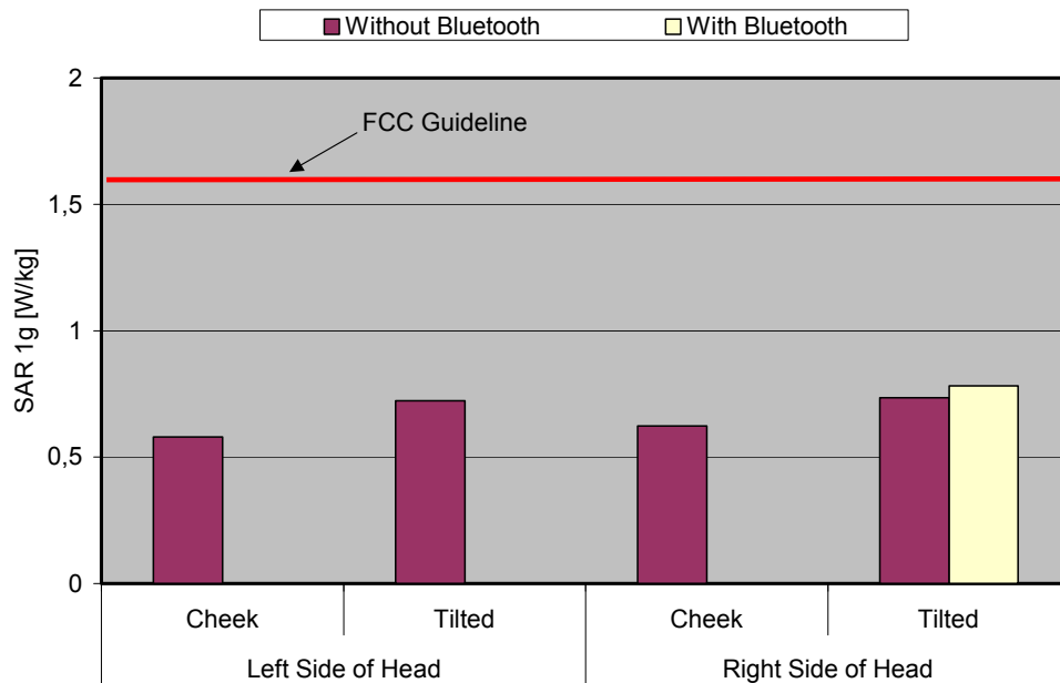
Fig. 8: The measured head phantom SAR values for the Siemens CX75 for PCS 1900 in comparison to the FCC exposure limit.
