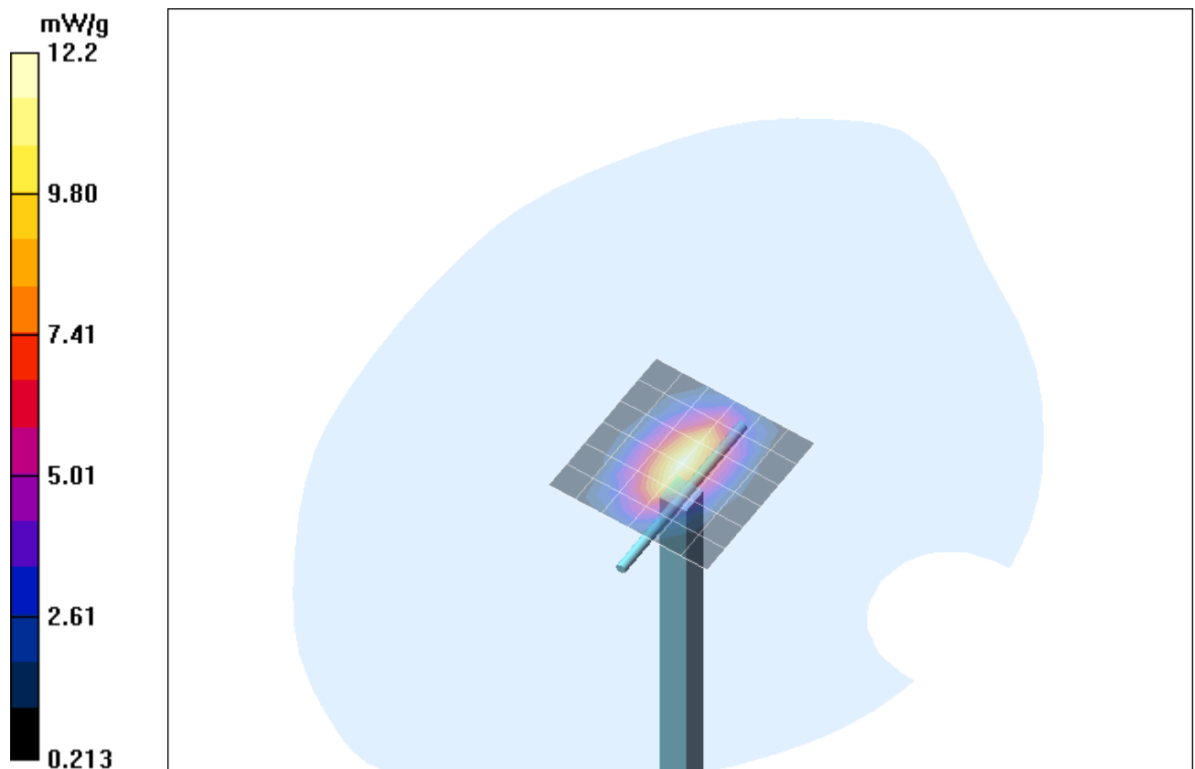
Fig. 12: Validation measurement 1900 MHz body (April 19, 2005), coarse grid. Ambient Temperature: 22.0° C, Liquid Temperature: 21.0° C.
