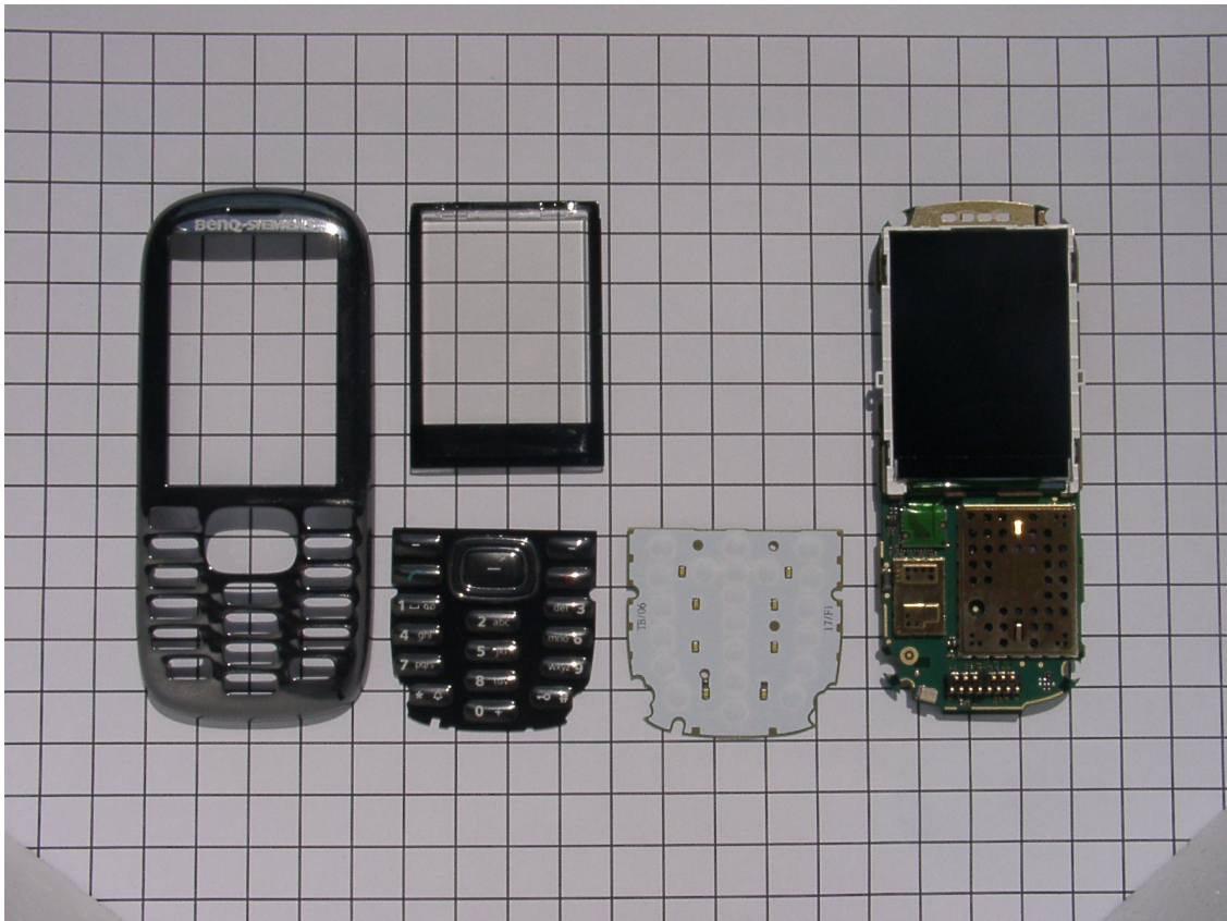
Device disassembled from top to bottom (1) 1 cm Grid
