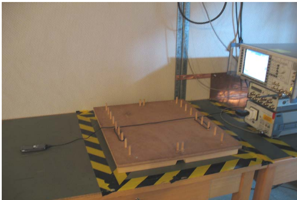
Photo 4 (Conducted Emissions): (Test Set-up No.2)
