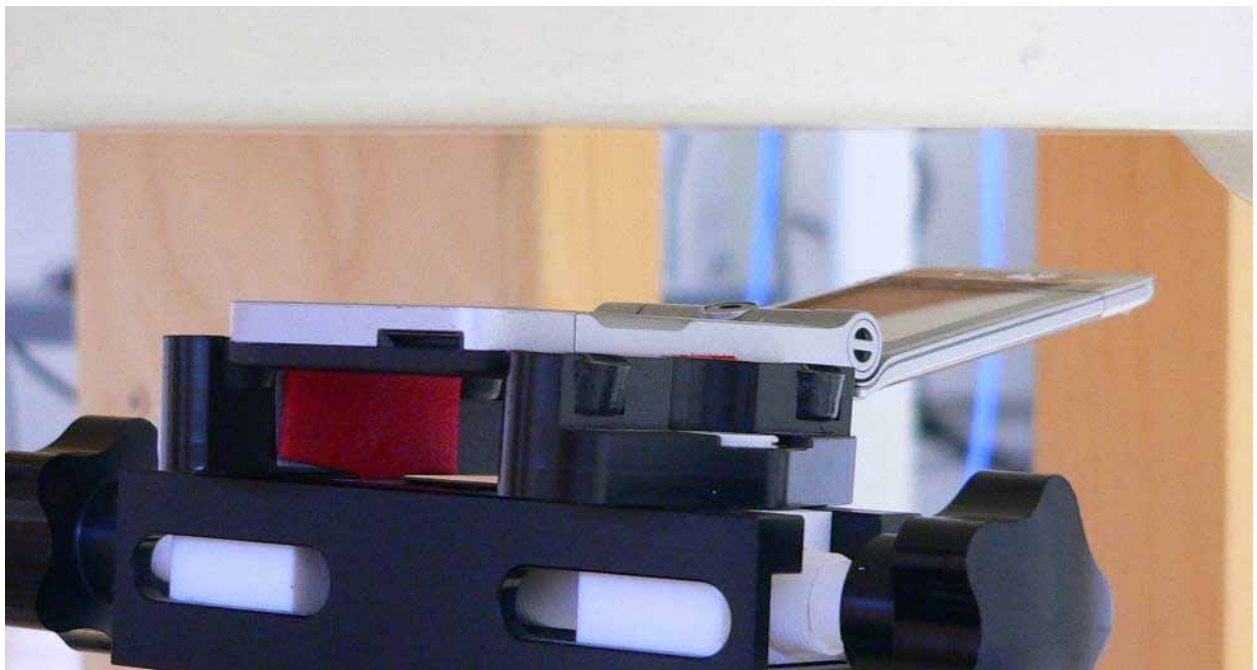
Fig. 27: Body worn configuration, PTT mode (Class 10), display towards the phantom.
