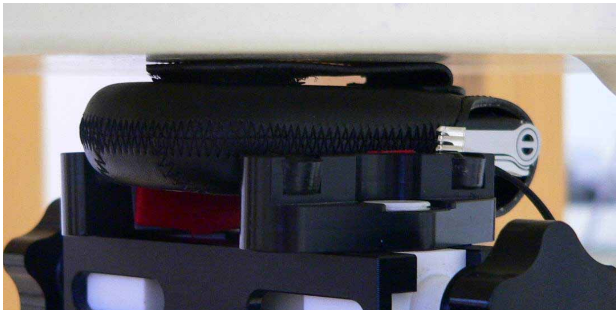
Fig. 24: Body worn configuration, GSM with headset and FCL 160 carry case, antenna towards the phantom.
