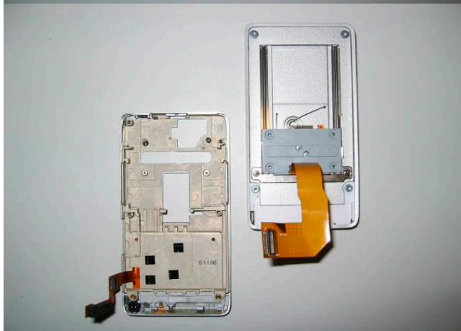
EL71 disassembled
