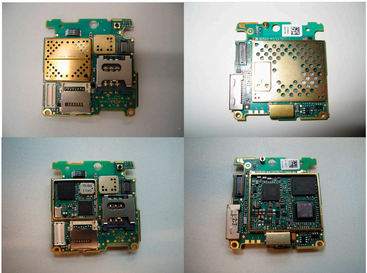
Main PCB
