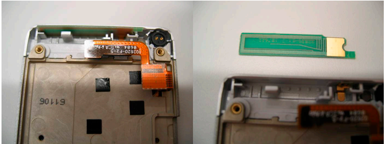
EL71 BT FPC-antenna & GSM PCB-antenna
