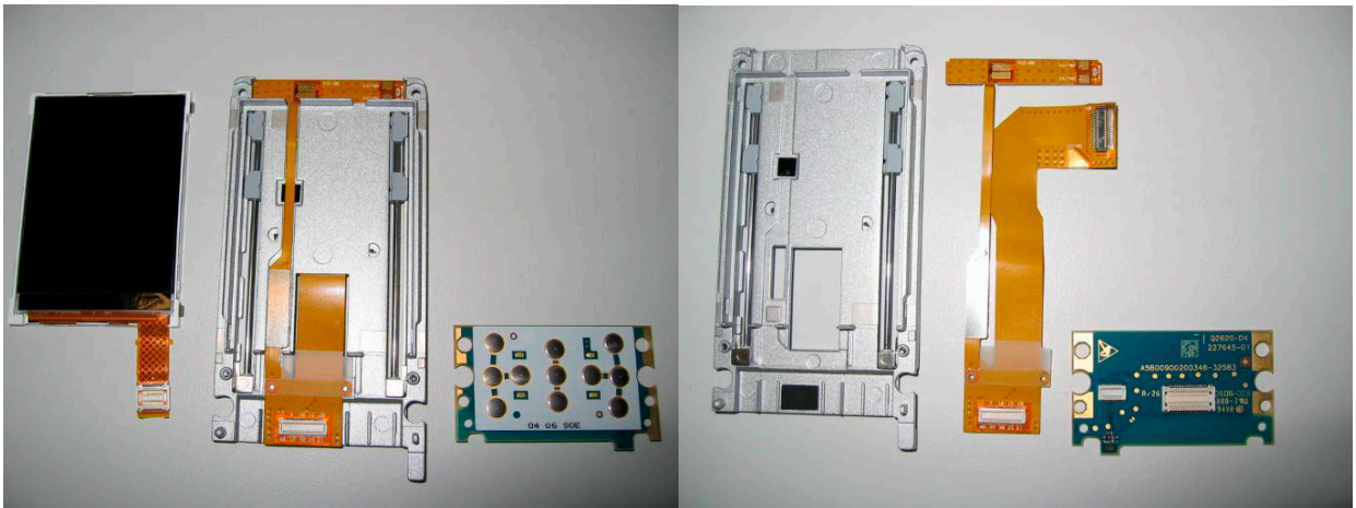
EL71 disassembled slider (step 2)
