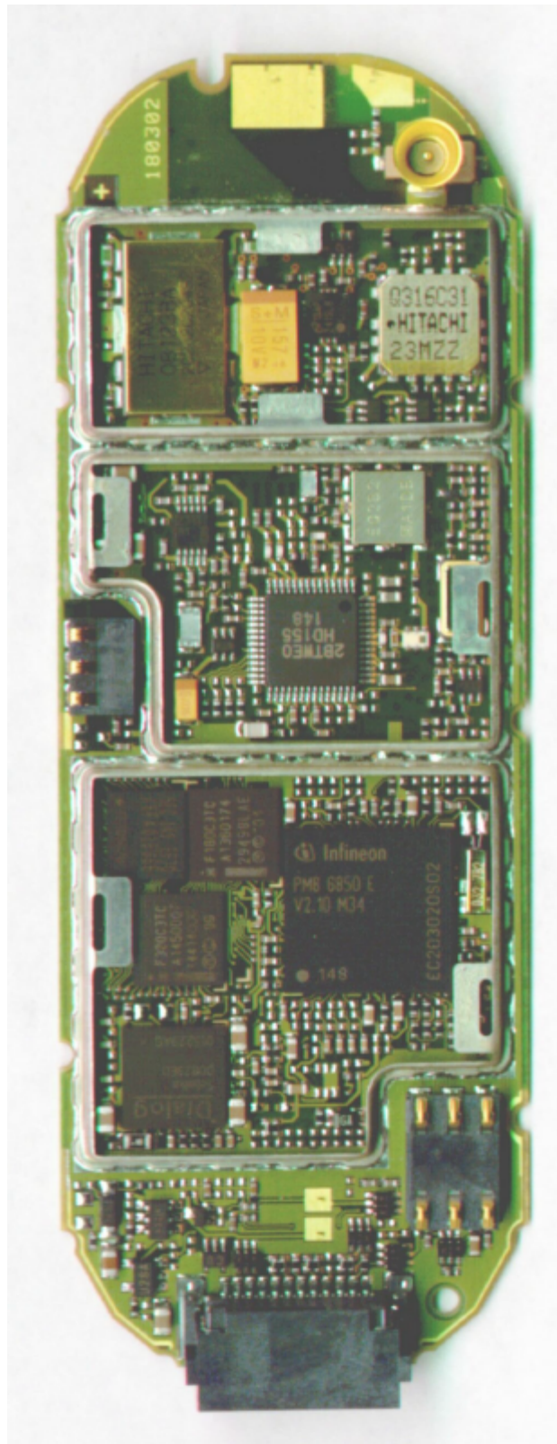
M46 – Main Board (side 2, without shielding)
