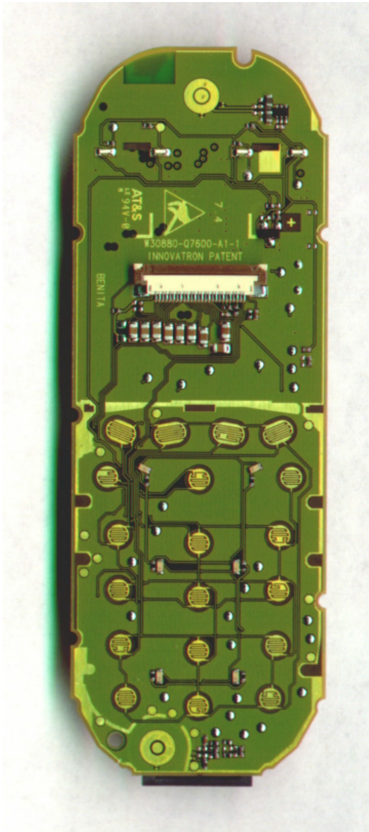
M46 – Main Board (side 1)
