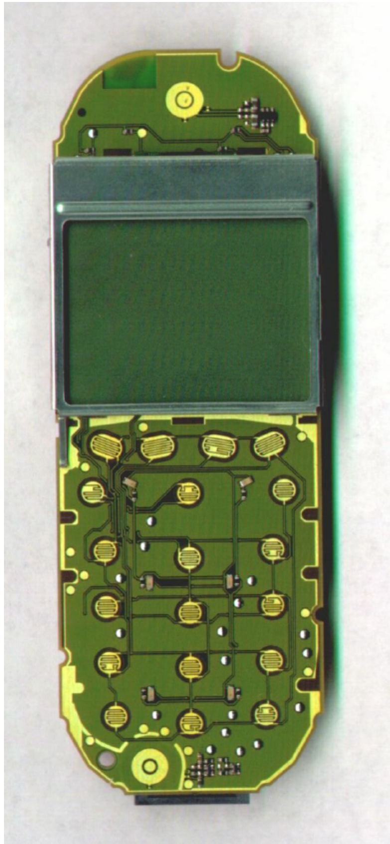
M46 – Main Board (side 1 with Display)
