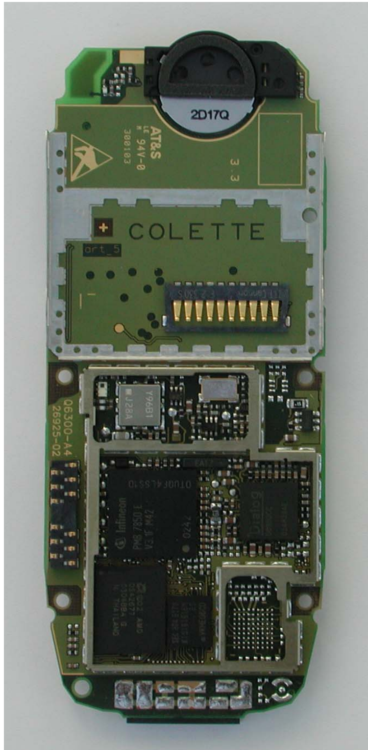
M55 Board without shielding and without display, side 1
