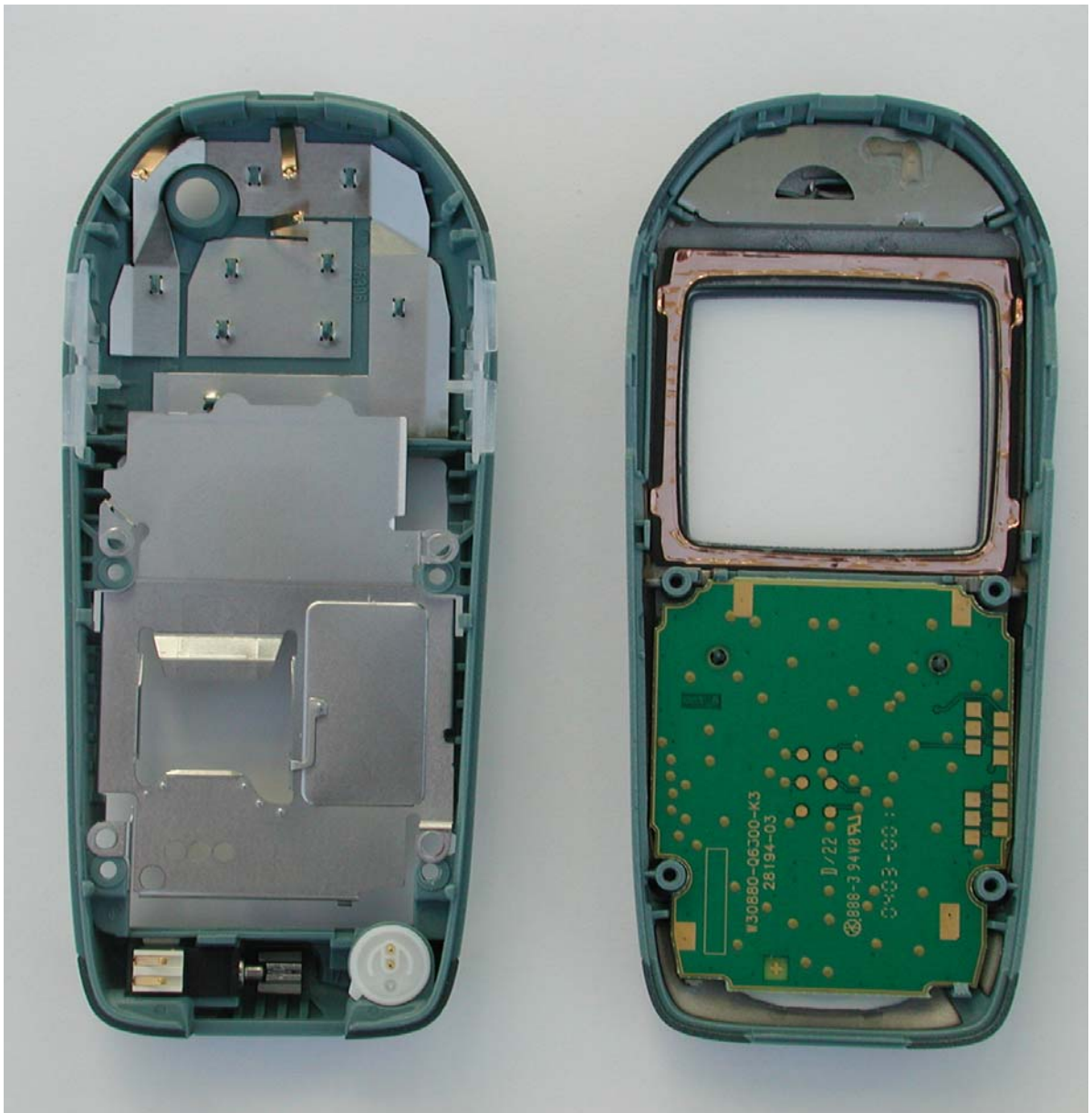
M55 Disassembly step 2
