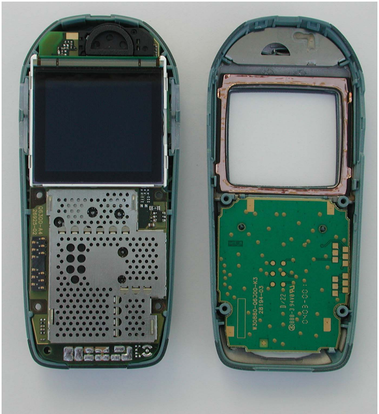
M55 Disassembly step 1
