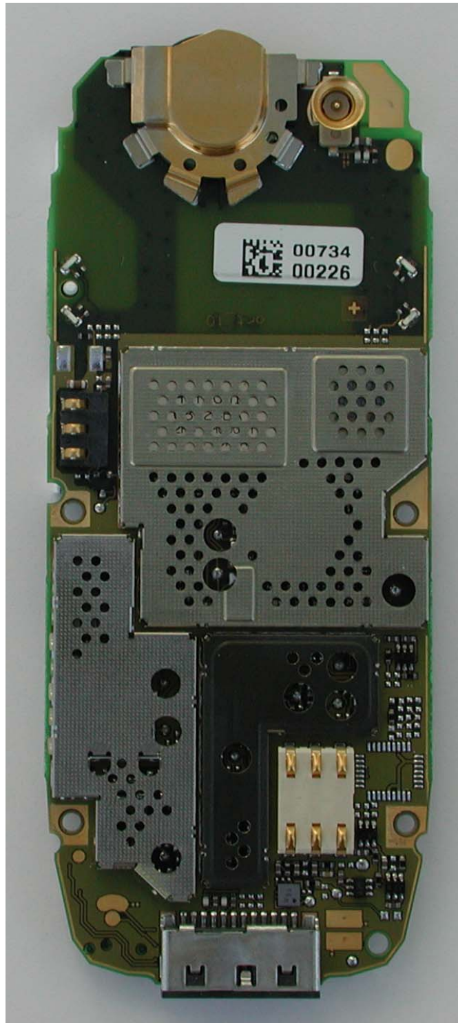
M55 Board with shielding, side 2
