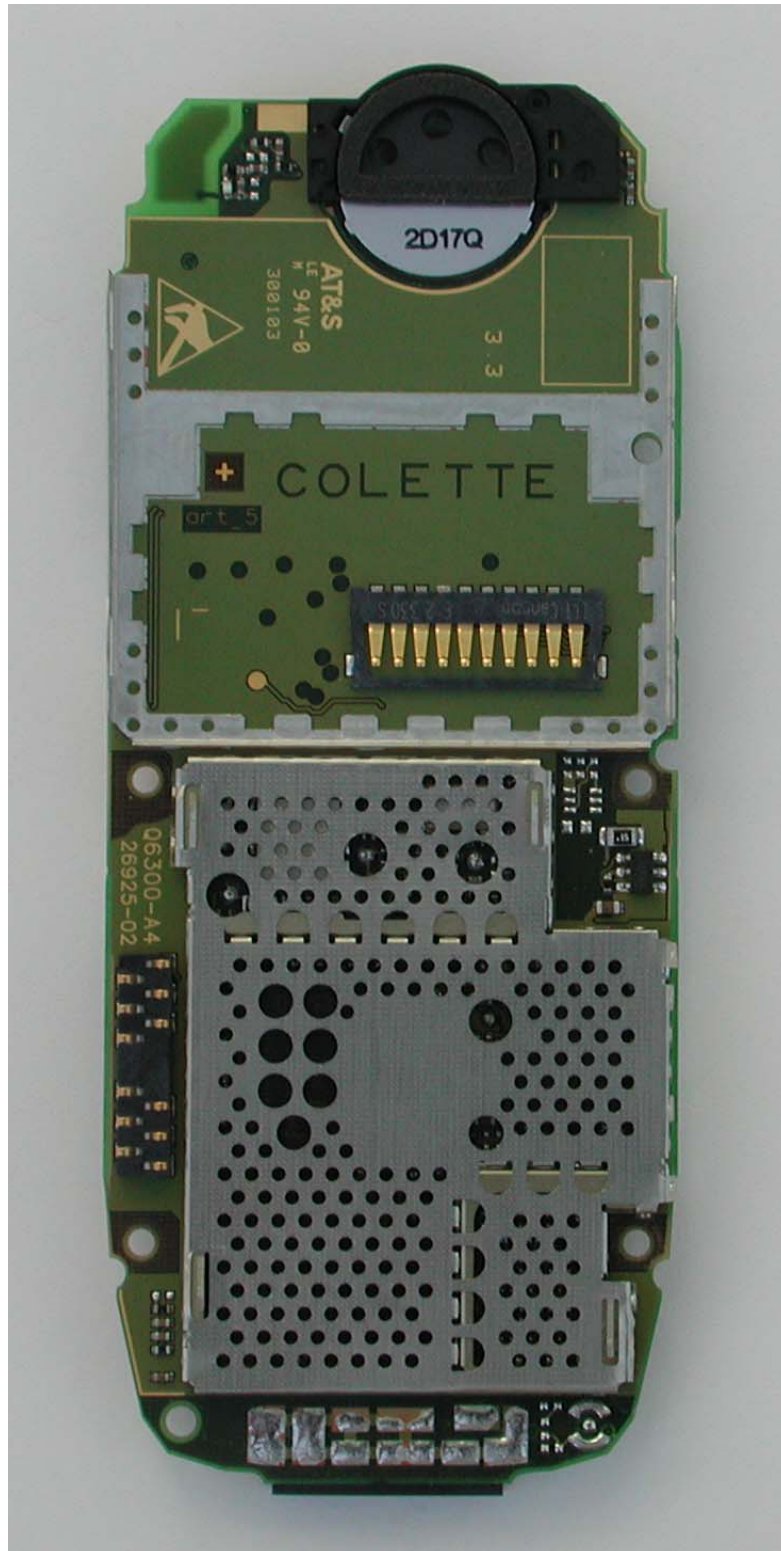
M55 Board with shielding, side 1
