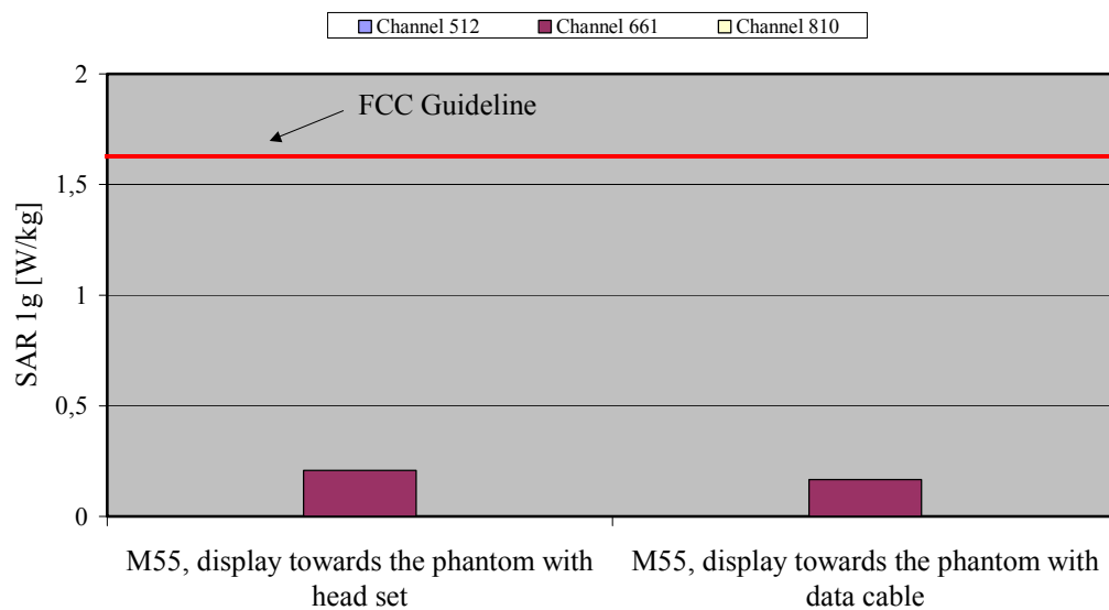
Fig. 11: The measured SAR values (1 TX) in body-worn configuration for the Siemens M55 (display towards the phantom) with leather case FCL-500 for PCS 1900 in comparison to the FCC exposure limit..
