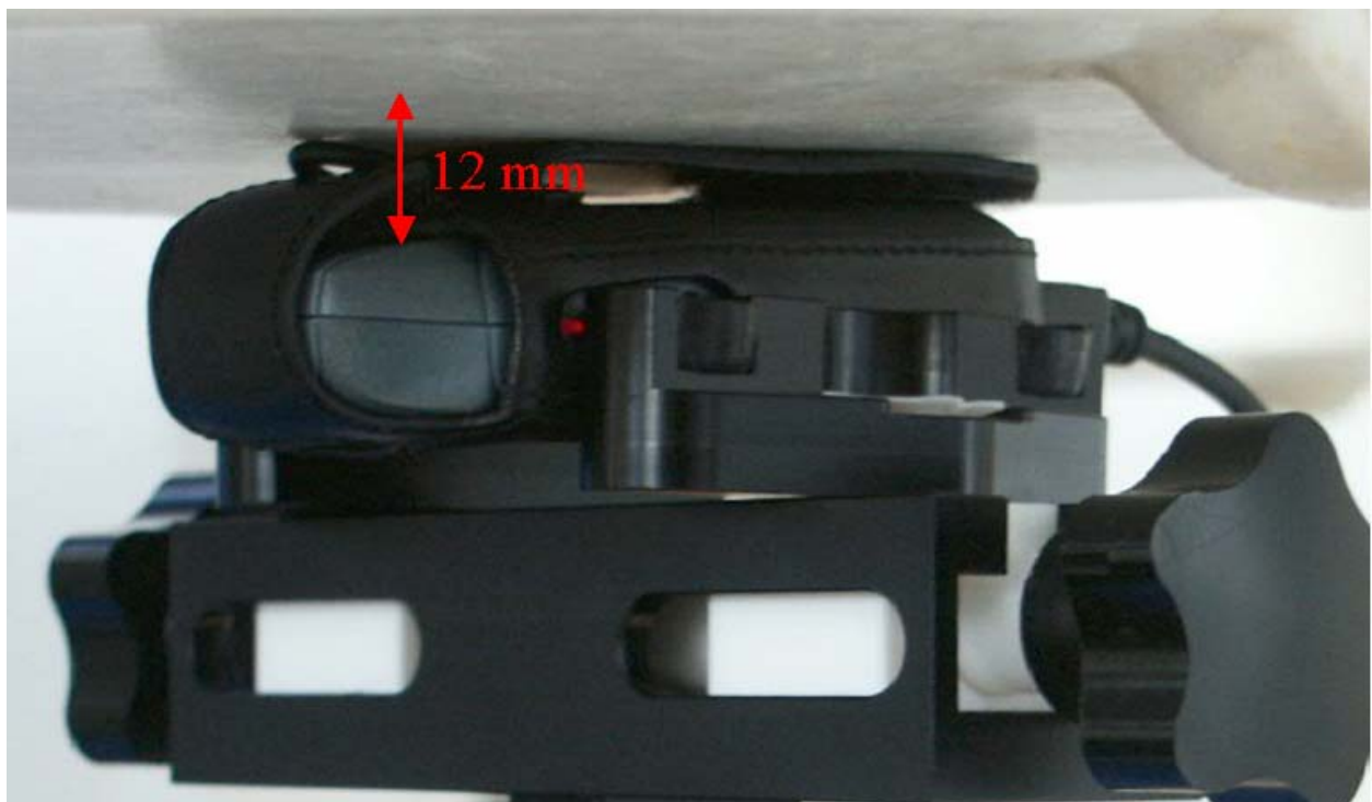
Fig. 33: Body worn configuration, with leather case FCL-500 and data cable, display towards the ground.
