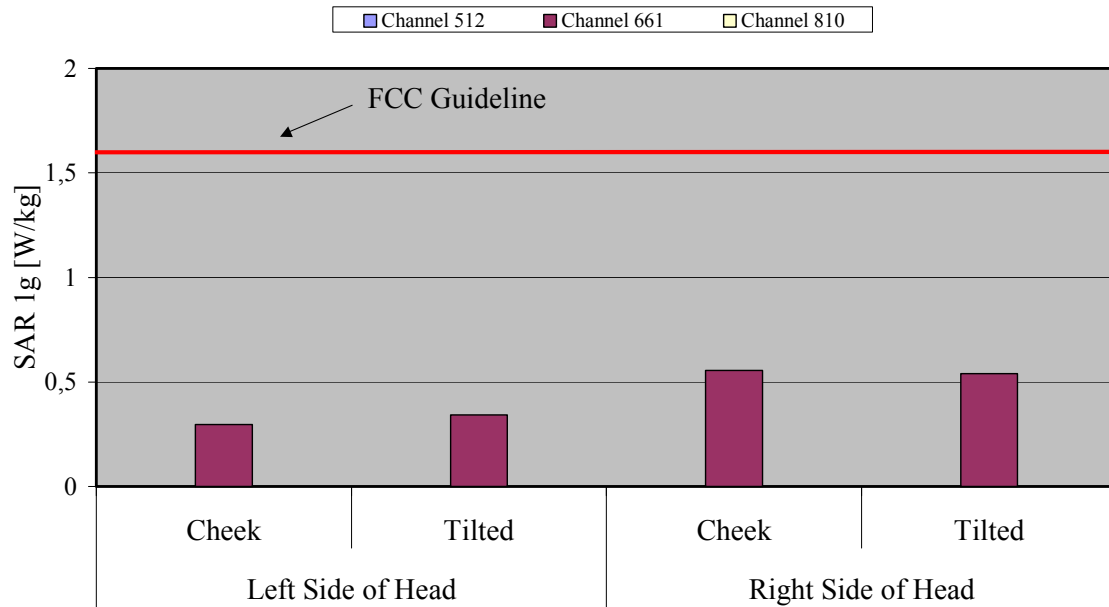
Fig. 8: The measured head phantom SAR values for the Siemens M55 (without camera) for PCS 1900 in comparison to the FCC exposure limit.
