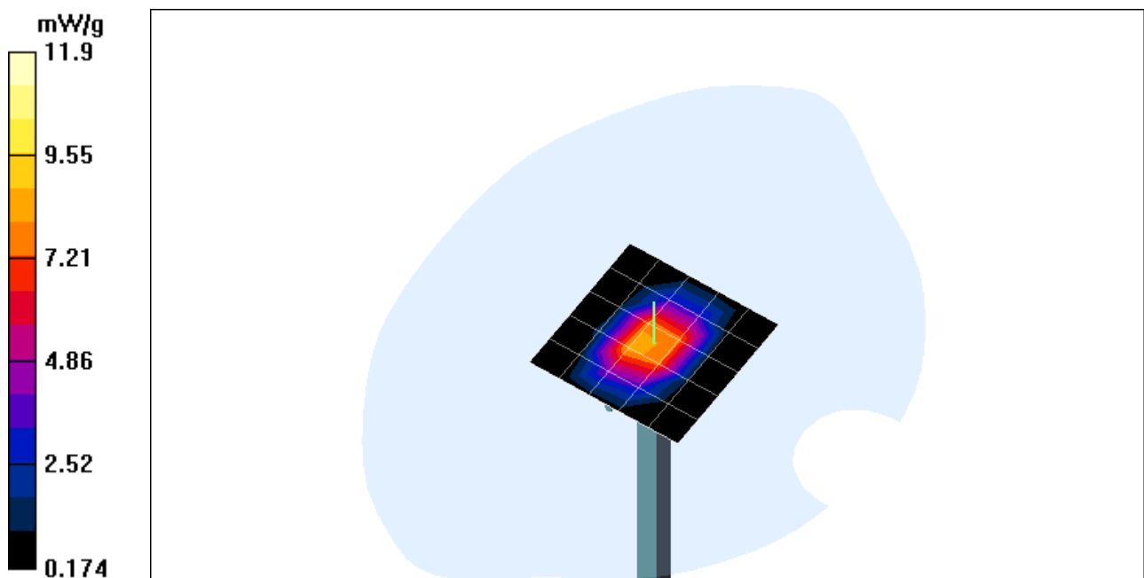
Fig. 12: Validation measurement 1900 MHz Head (09.04.2003), coarse grid. Ambient Temperature: 21.2° C, Liquid Temperature: 19.7° C.
