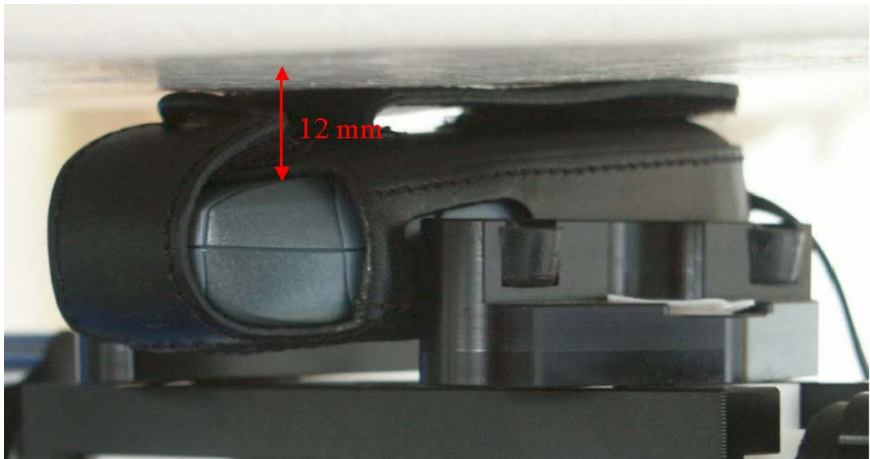
Fig. 32: Body worn configuration, with leather case FCL-500 and headset, display towards the ground.
