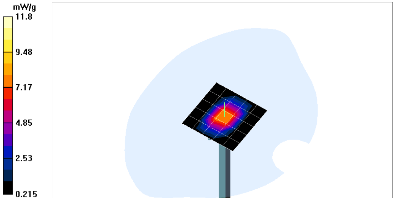
Fig. 13: Validation measurement 1900 MHz body (03.04.2003), coarse grid. Ambient Temperature: 21.0° C, Liquid Temperature: 19.9° C.
