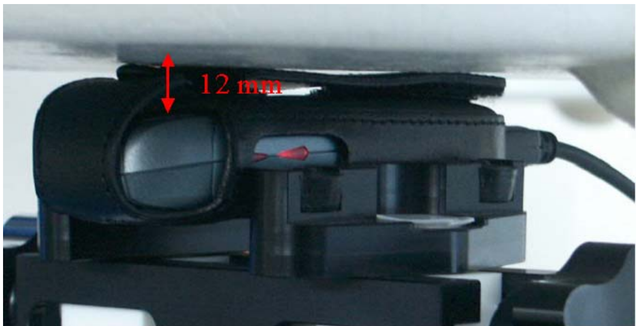
Fig. 35: Body worn configuration, with leather case FCL-500 and datacable, display towards the phantom.
