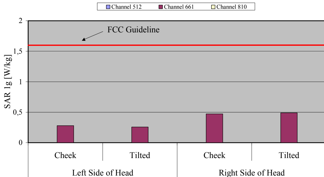
Fig. 9: The measured head phantom SAR values for the Siemens M55 (with camera) for PCS 1900 in comparison to the FCC exposure limit.
