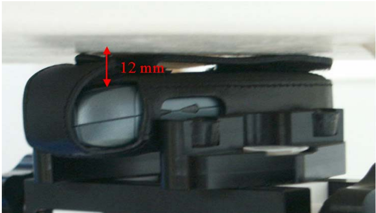
Fig. 34: Body worn configuration, with leather case FCL-500 and headset, display towards the phantom.
