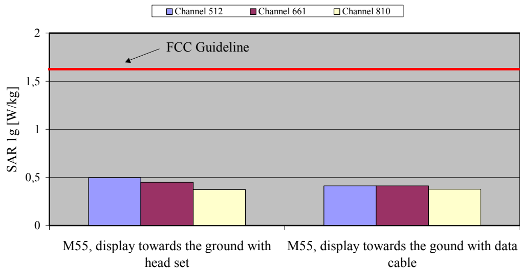
Fig. 10: The measured SAR values (1 TX) in body-worn configuration for the Siemens M55 (display towards the ground) with leather case FCL-500 for PCS 1900 in comparison to the FCC exposure limit.
