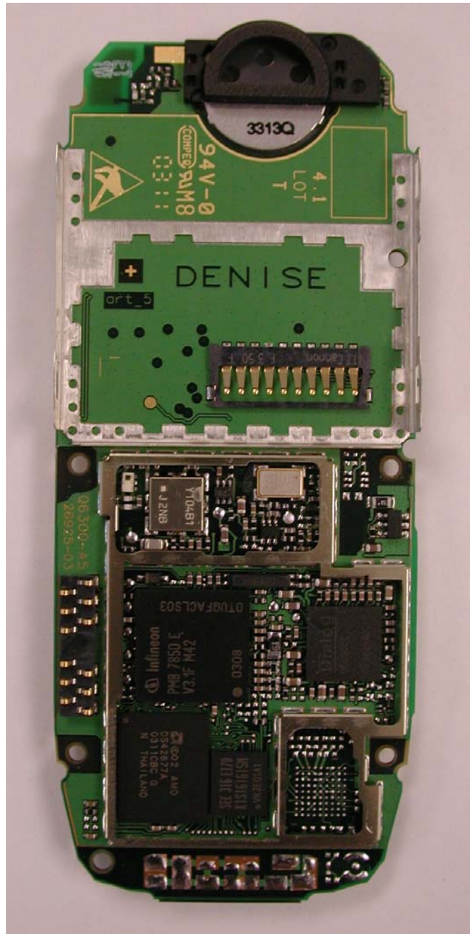
M56 Board without shielding and without display, side 1
