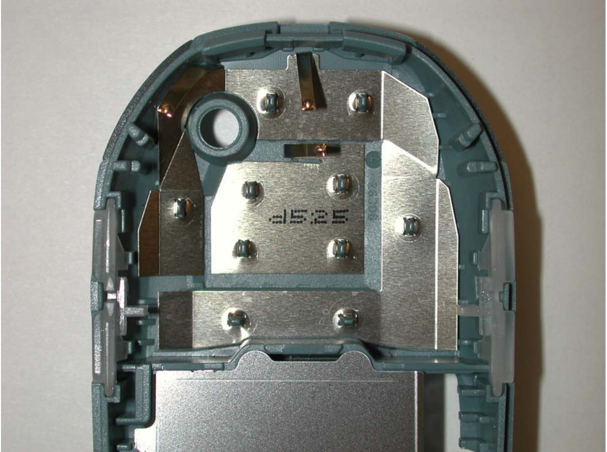
GSM Dual-band Antenna detail
