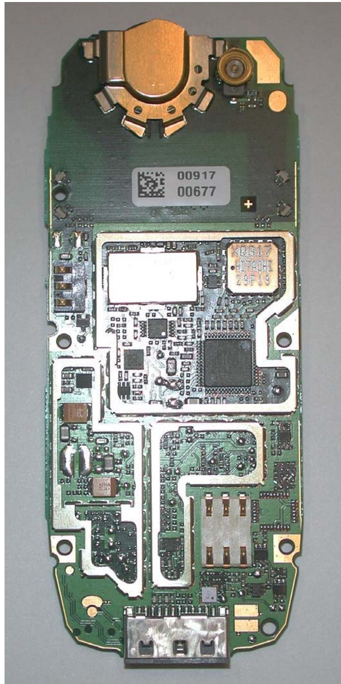
M56 Board without shielding, side 2
