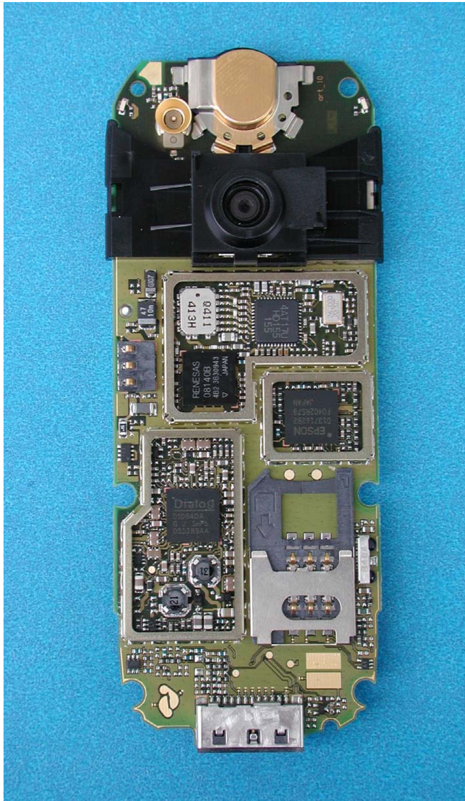
M65 board without shield (back)
