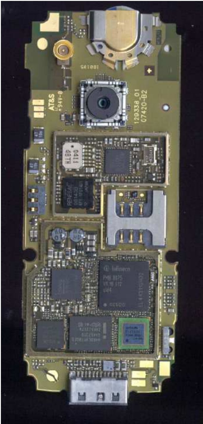
M75 PCB Back View Shields Removed
