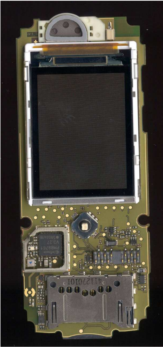
M75 PCB Front View Shields Removed
