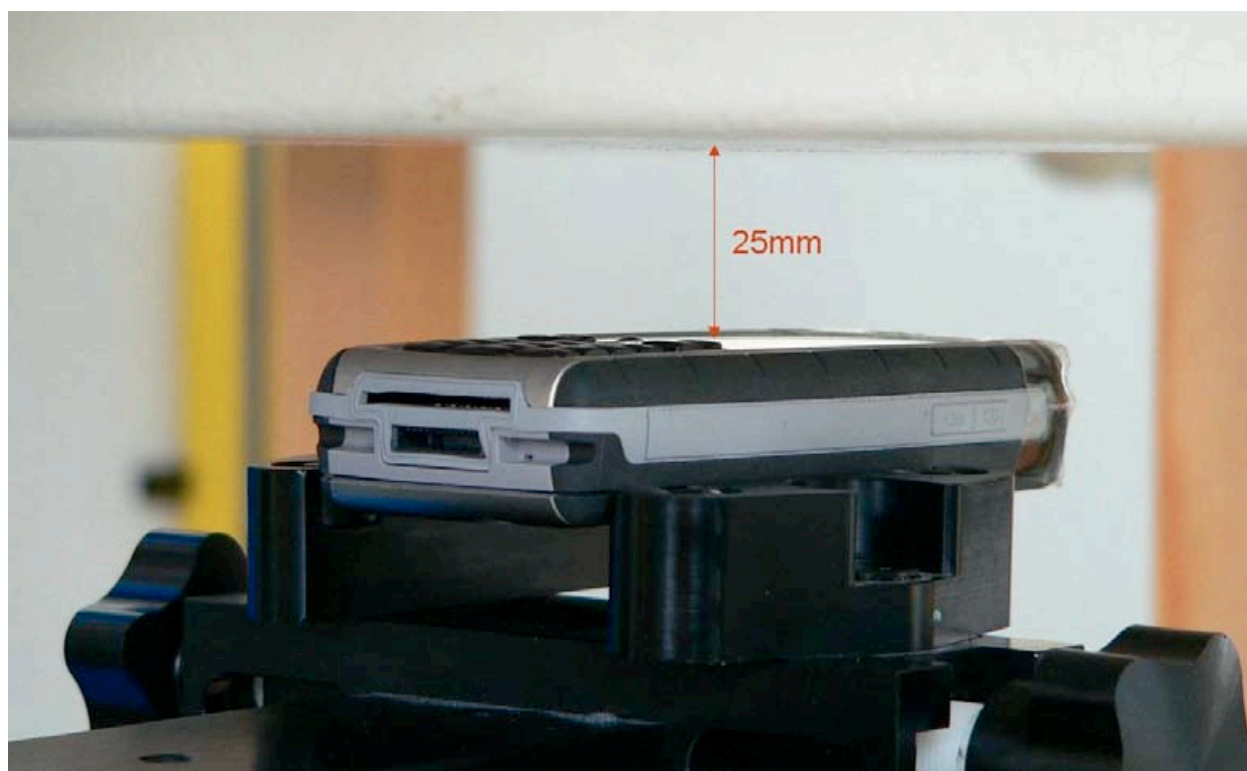
Fig. 27: Body worn configuration, PTT mode (Class 10), display towards the phantom.
