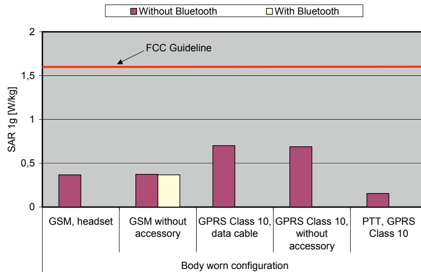
Fig. 10: The measured SAR values in body-worn configuration for the Siemens M75 for PCS 1900 with a distance of 15 mm (PTT = 25 mm) in comparison to the FCC exposure limit.
