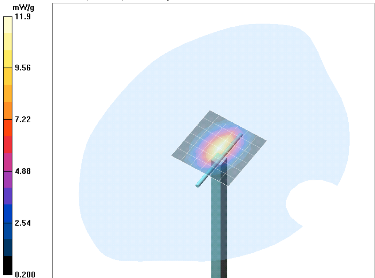
Fig. 11: Validation measurement 1900 MHz Head (May 11, 2005), coarse grid. Ambient Temperature: 21.2° C, Liquid Temperature: 20.1° C.
