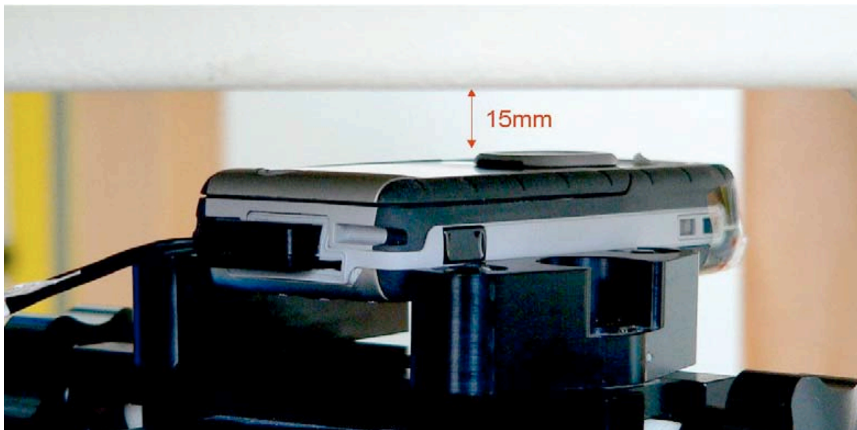
Fig. 24: Body worn configuration, GSM with headset, antenna towards the phantom.
