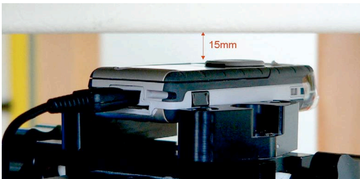
Fig. 25: Body worn configuration, GPRS Class 10 with data cable, antenna towards the phantom.
