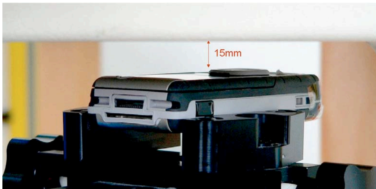
Fig. 26: Body worn configuration, GSM and GPRS Class 10, antenna towards the phantom.
