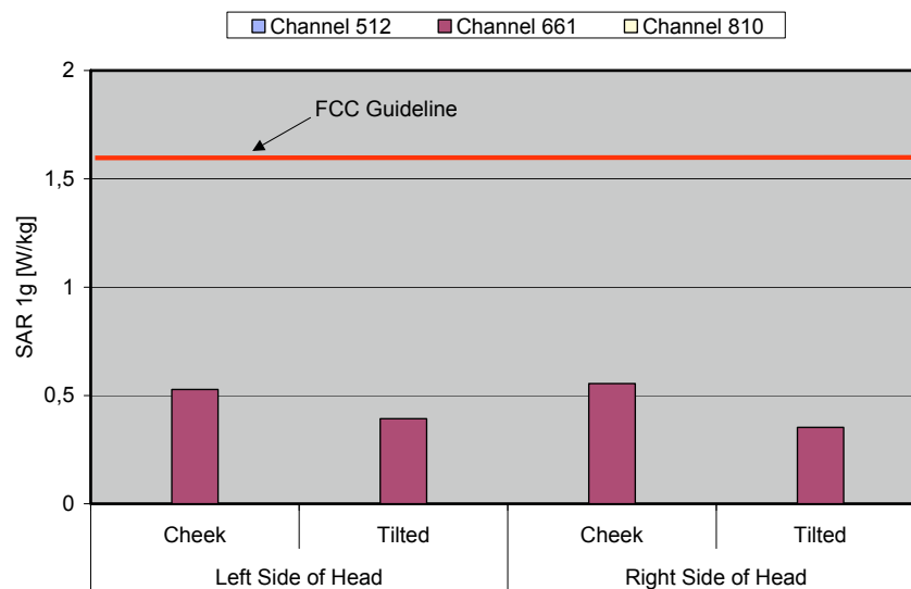
Fig. 9: The measured head phantom SAR values for the Siemens M75 with flash for PCS 1900 in comparison to the FCC exposure limit.
