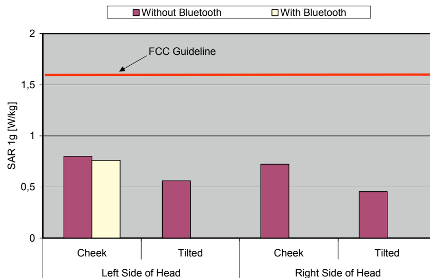
Fig. 8: The measured head phantom SAR values for the Siemens M75 for PCS 1900 in comparison to the FCC exposure limit.
