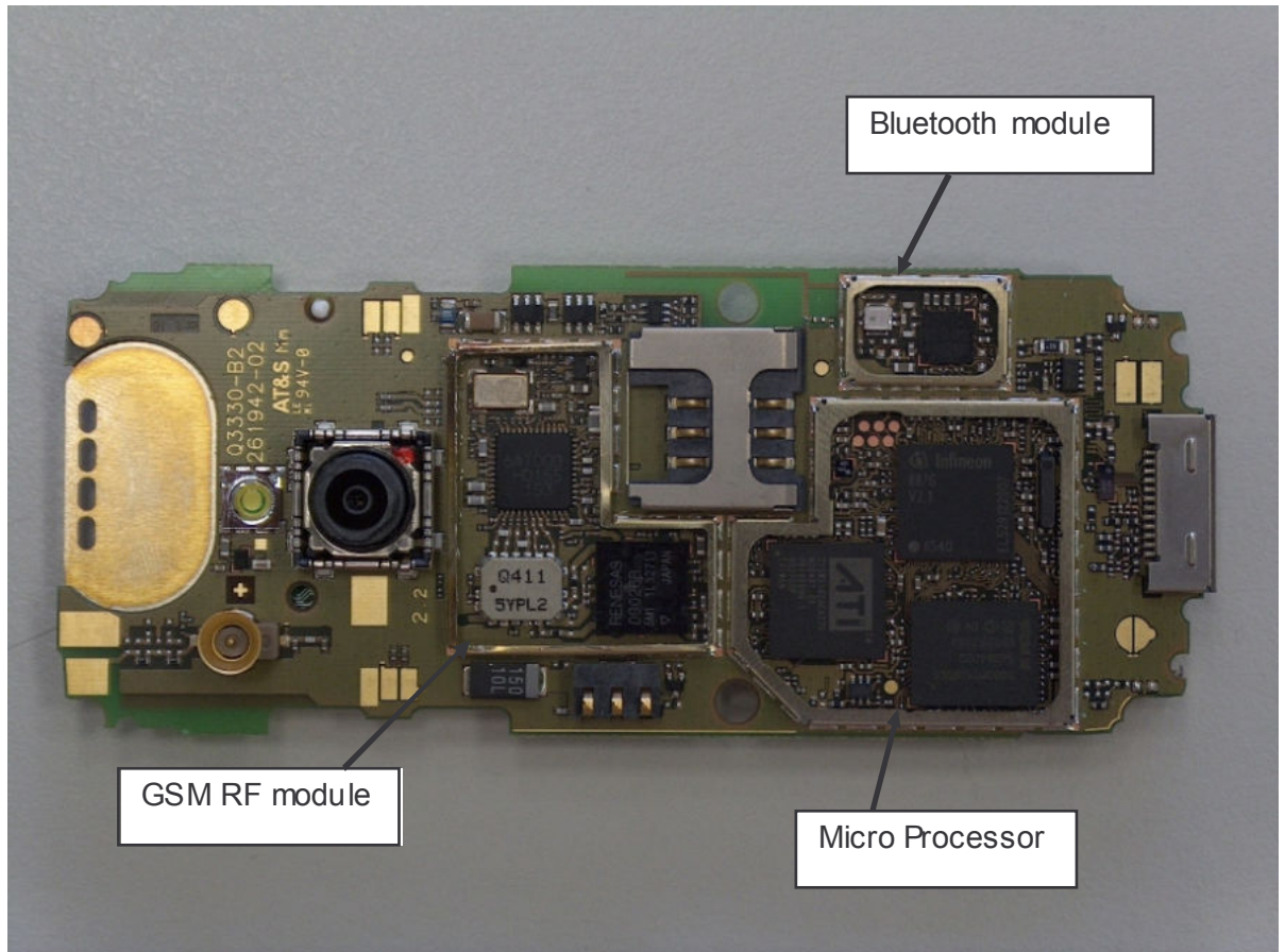
Disassemble Step 6: Back Side of main PCB
