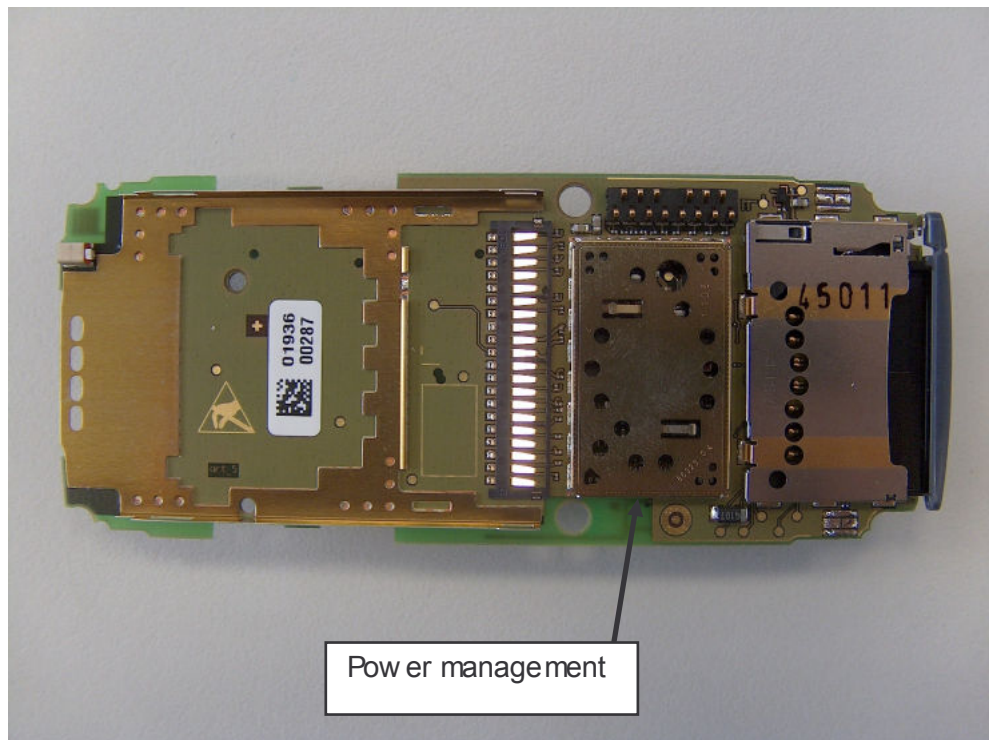
Disassemble Step 5: Front Side of main PCB
