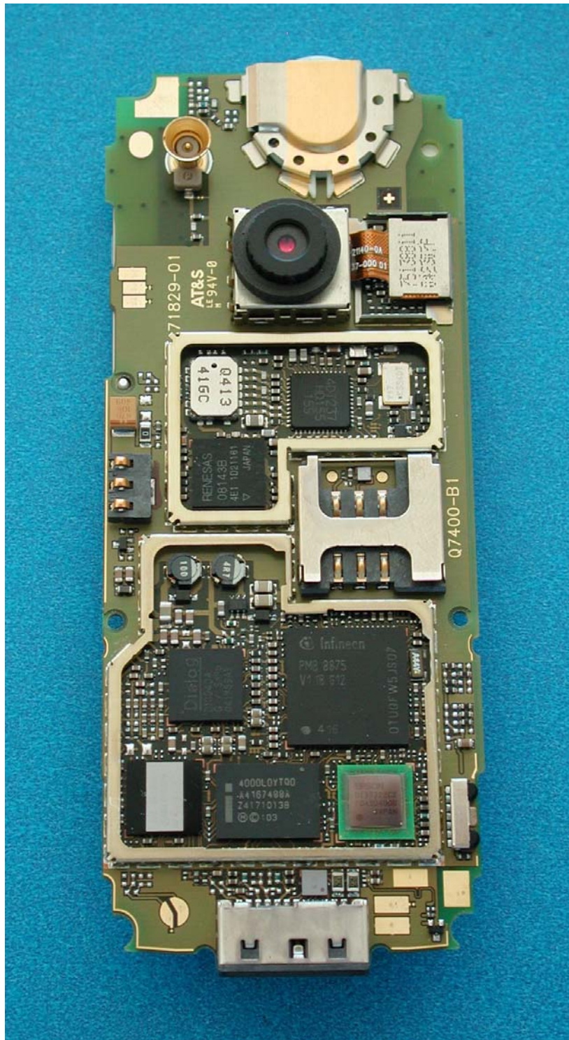
S66 PCB Back View Shields Removed
