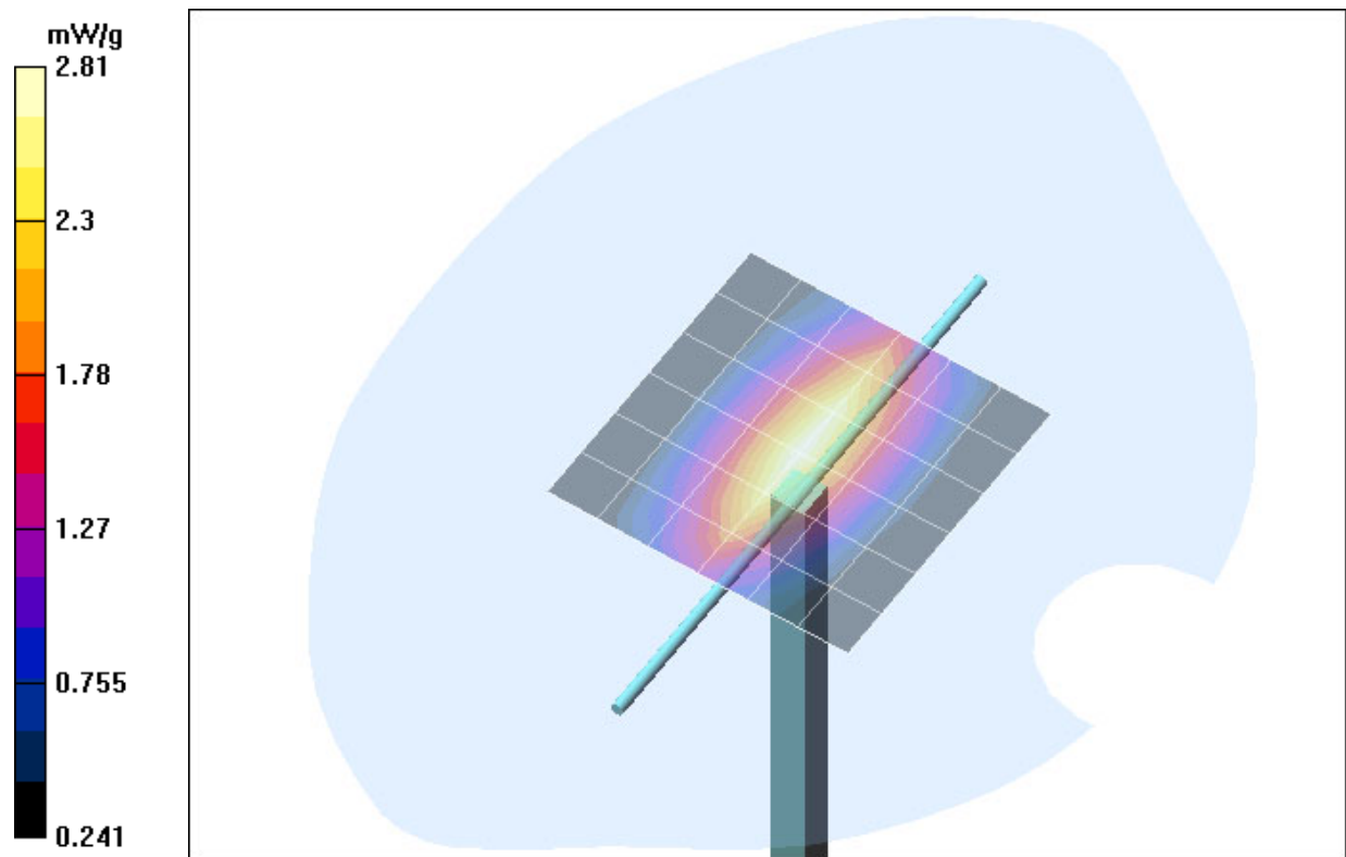
Fig. 15: Validation measurement 835 MHz body (August 24, 2004), coarse grid. Ambient Temperature: 22.0° C, Liquid Temperature: 21.0° C.
