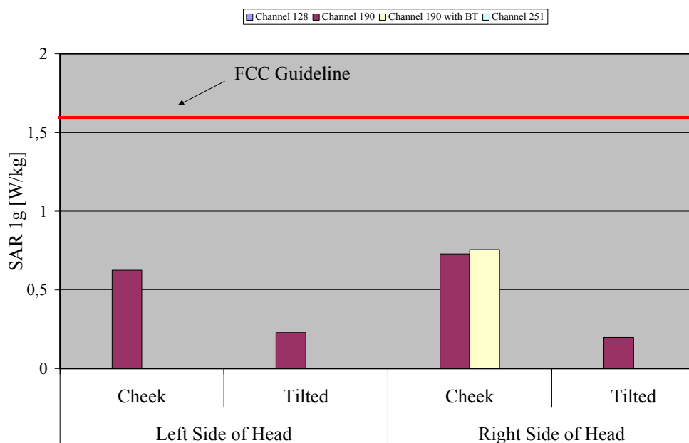
Fig. 9: The measured head phantom SAR values for the Siemens S66 with flash for GSM 850 in comparison to the FCC exposure limit.
