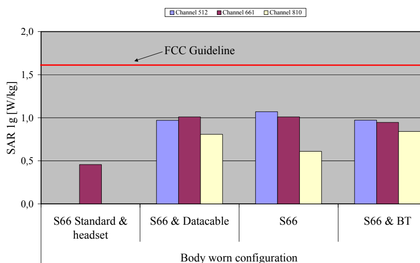
Fig. 13: The measured SAR values in body-worn configuration for the Siemens S66 for PCS 1900 (1 TX slot with headset, and 2 TX slots with and without data cable and Bluetooth, gap = 22 mm) in comparison to the FCC exposure limit.
