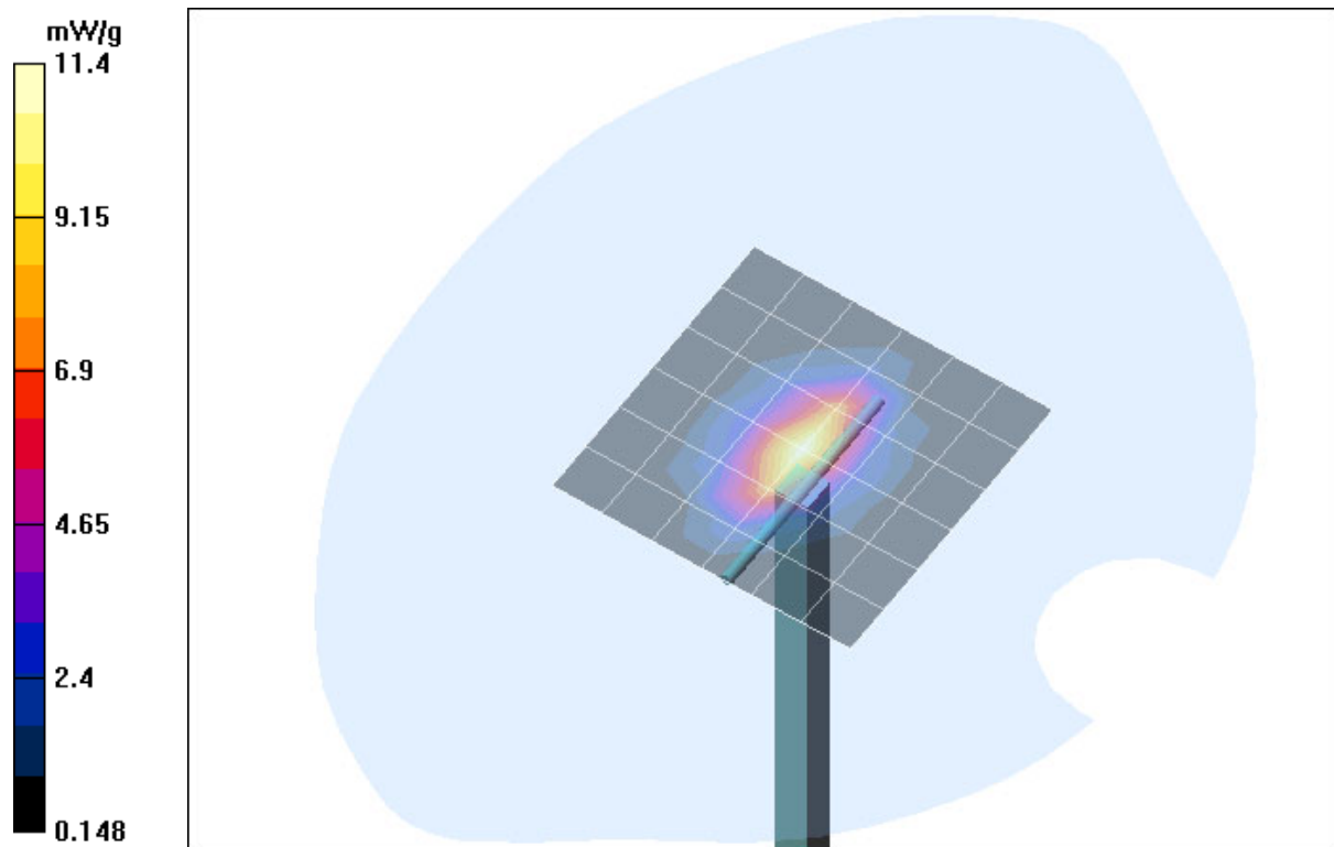
Fig. 17: Validation measurement 1900 MHz Head (August 19, 2004), coarse grid. Ambient Temperature: 21.6° C, Liquid Temperature: 21.1° C.
