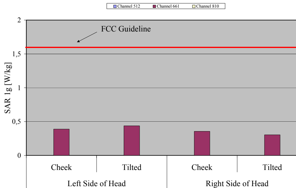
Fig. 11: The measured head phantom SAR values for the Siemens S66 with flash for PCS 1900 in comparison to the FCC exposure limit.
