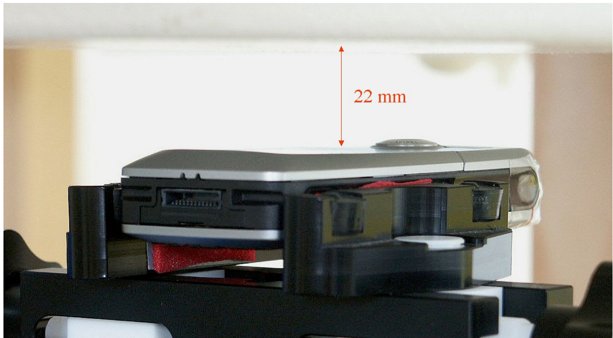
Fig. 31: Body worn configuration, GPRS mode (2 TX slot), antenna towards the phantom.
