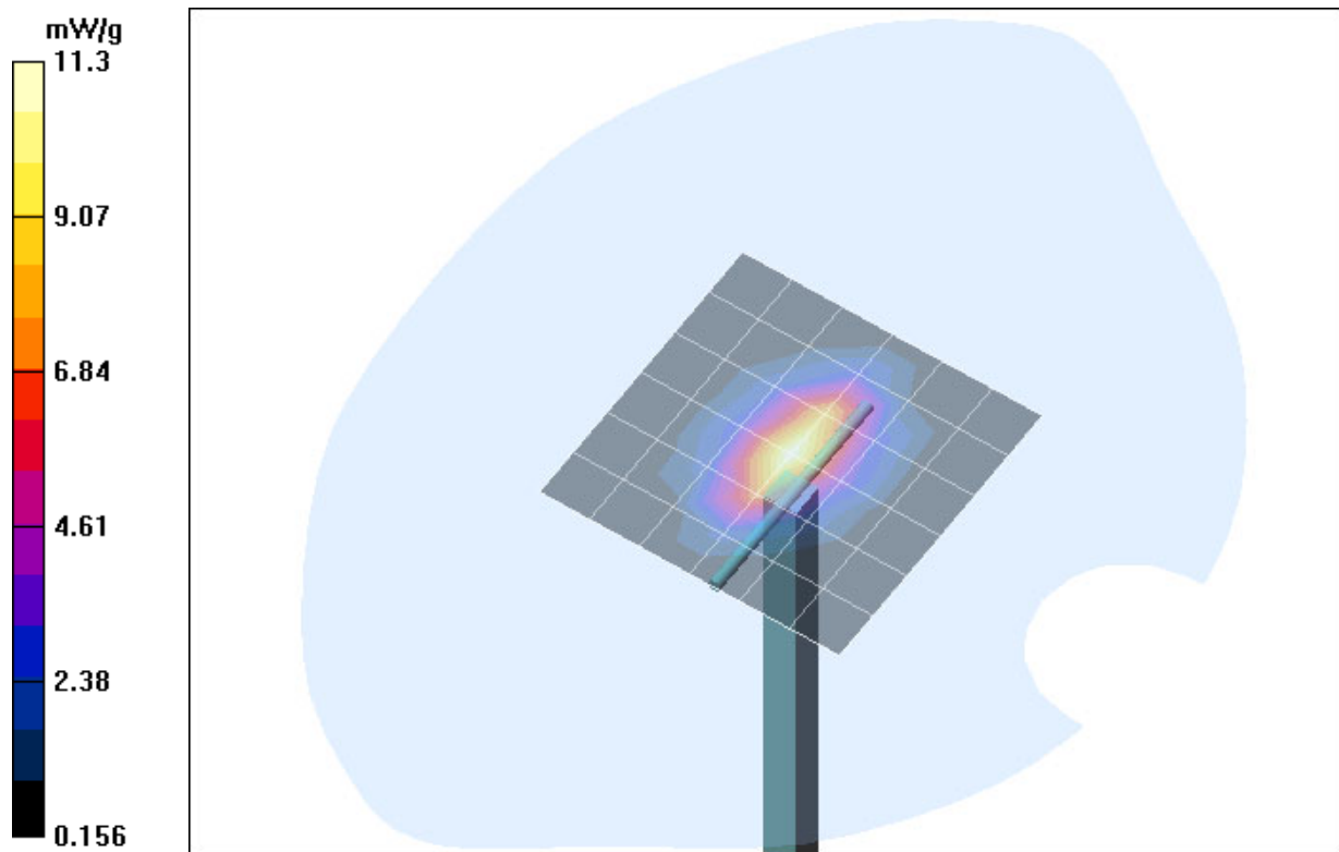
Fig. 16: Validation measurement 1900 MHz Head (August 23, 2004), coarse grid. Ambient Temperature: 20.6° C, Liquid Temperature: 20.0° C.
