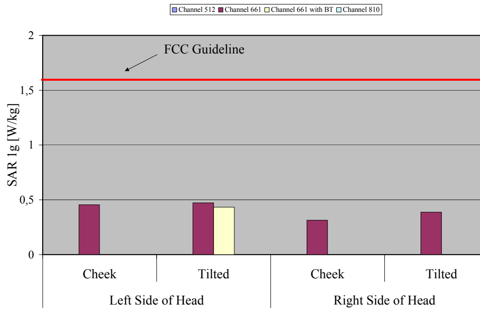
Fig. 10: The measured head phantom SAR values for the Siemens S66 without flash for PCS 1900 in comparison to the FCC exposure limit.
