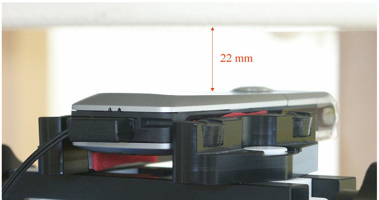
Fig. 32: Body worn configuration, GSM mode (1 TX ) with headset, antenna towards the phantom.
