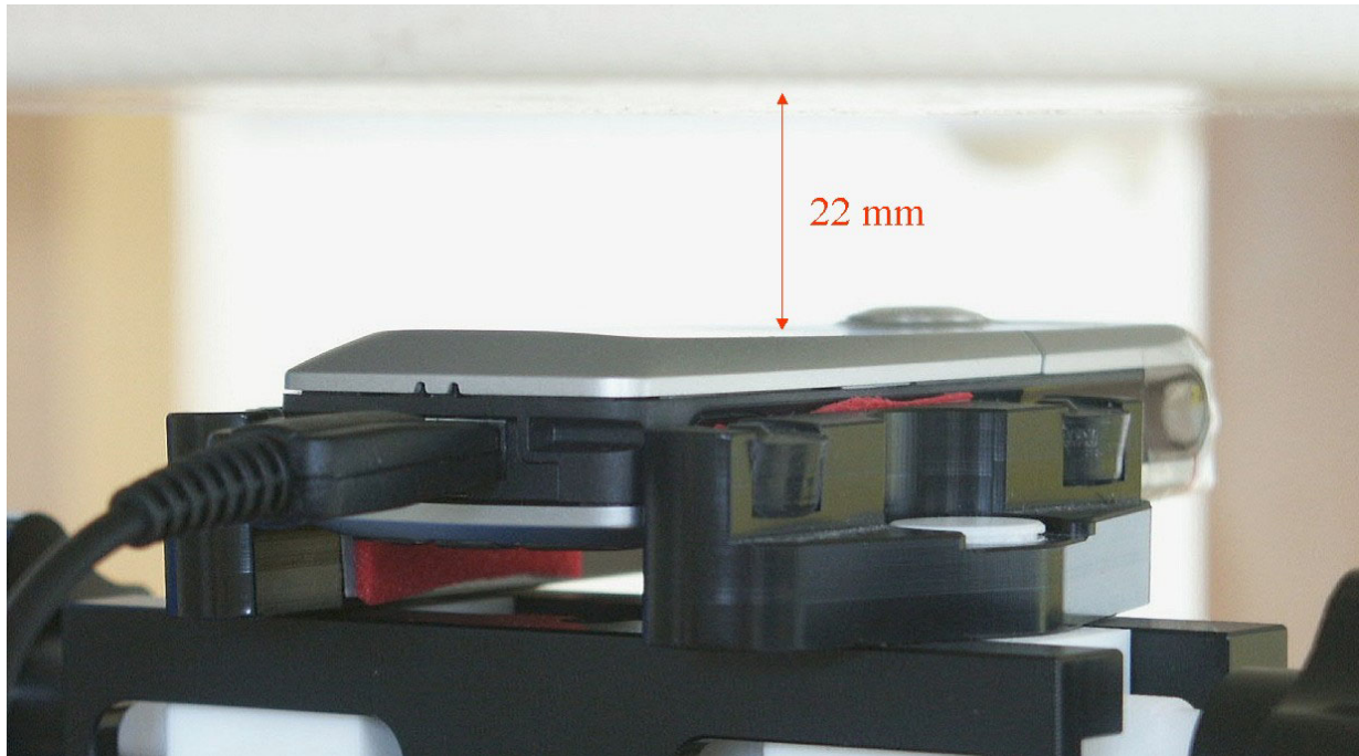
Fig. 33: Body worn configuration, GPRS mode (2 TX slot) with data cable, antenna towards the phantom.
