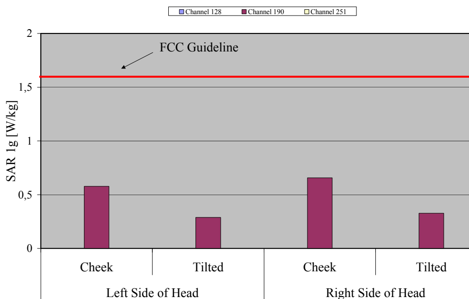
Fig. 8: The measured head phantom SAR values for the Siemens S66 without flash for GSM 850 in comparison to the FCC exposure limit.
