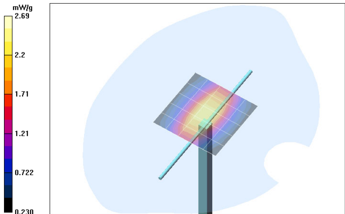
Fig. 14: Validation measurement 835MHz Head (August 18, 2004), coarse grid. Ambient Temperature: 21.9° C, Liquid Temperature: 21.3° C.
