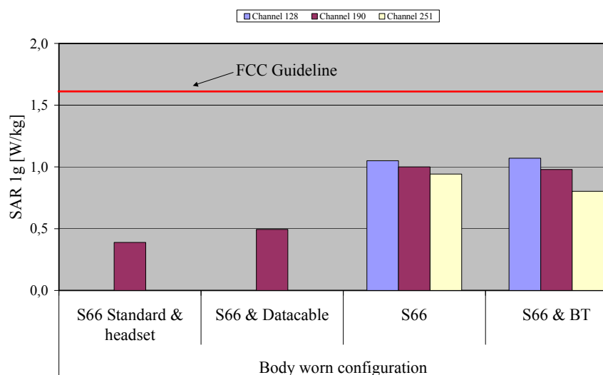
Fig. 12: The measured SAR values in body-worn configuration for the Siemens S66 for GSM 850 (1 TX slot with headset, and 2 TX slots with and without data cable and Bluetooth, gap = 22 mm) in comparison to the FCC exposure limit.
