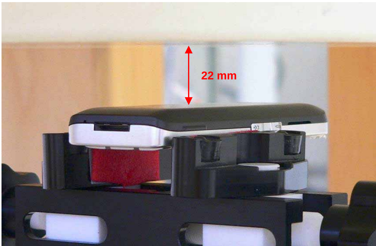
Fig. 27: Body worn configuration, GPRS (Class 10), BT activated, display towards the phantom.
