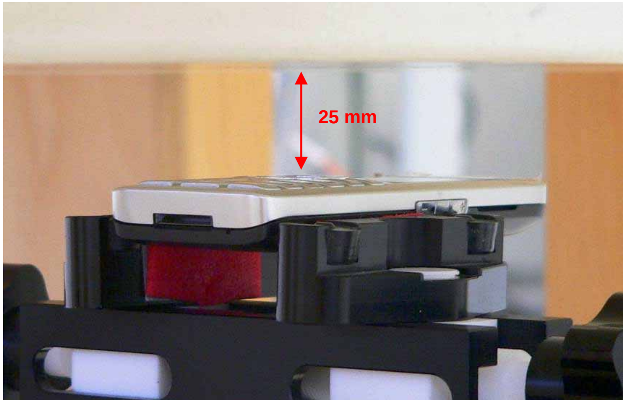
Fig. 28: Body worn configuration, PTT mode (Class 10), display towards the phantom.
