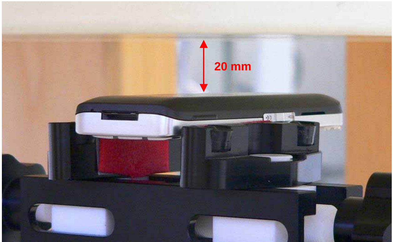
Fig. 24: Body worn configuration, GSM without accessory, antenna towards the phantom.
