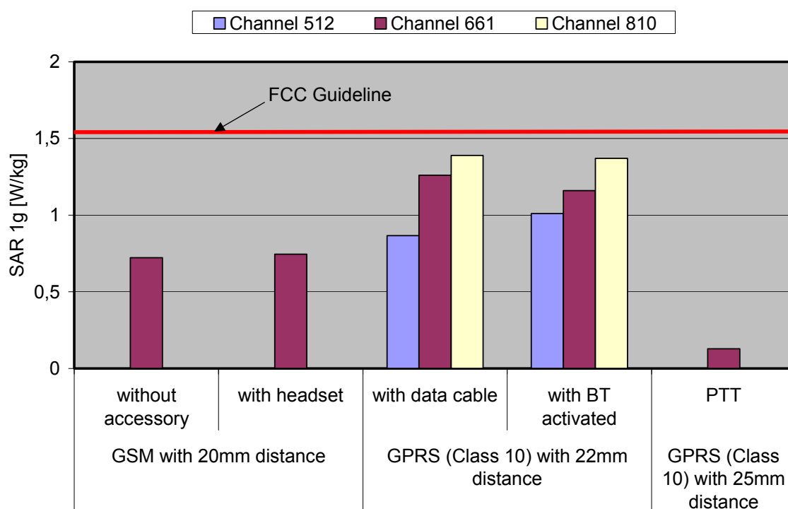
Fig. 9: The measured SAR values in body-worn configuration for the BenQ Siemens S68 for PCS 1900 in comparison to the FCC exposure limit.
