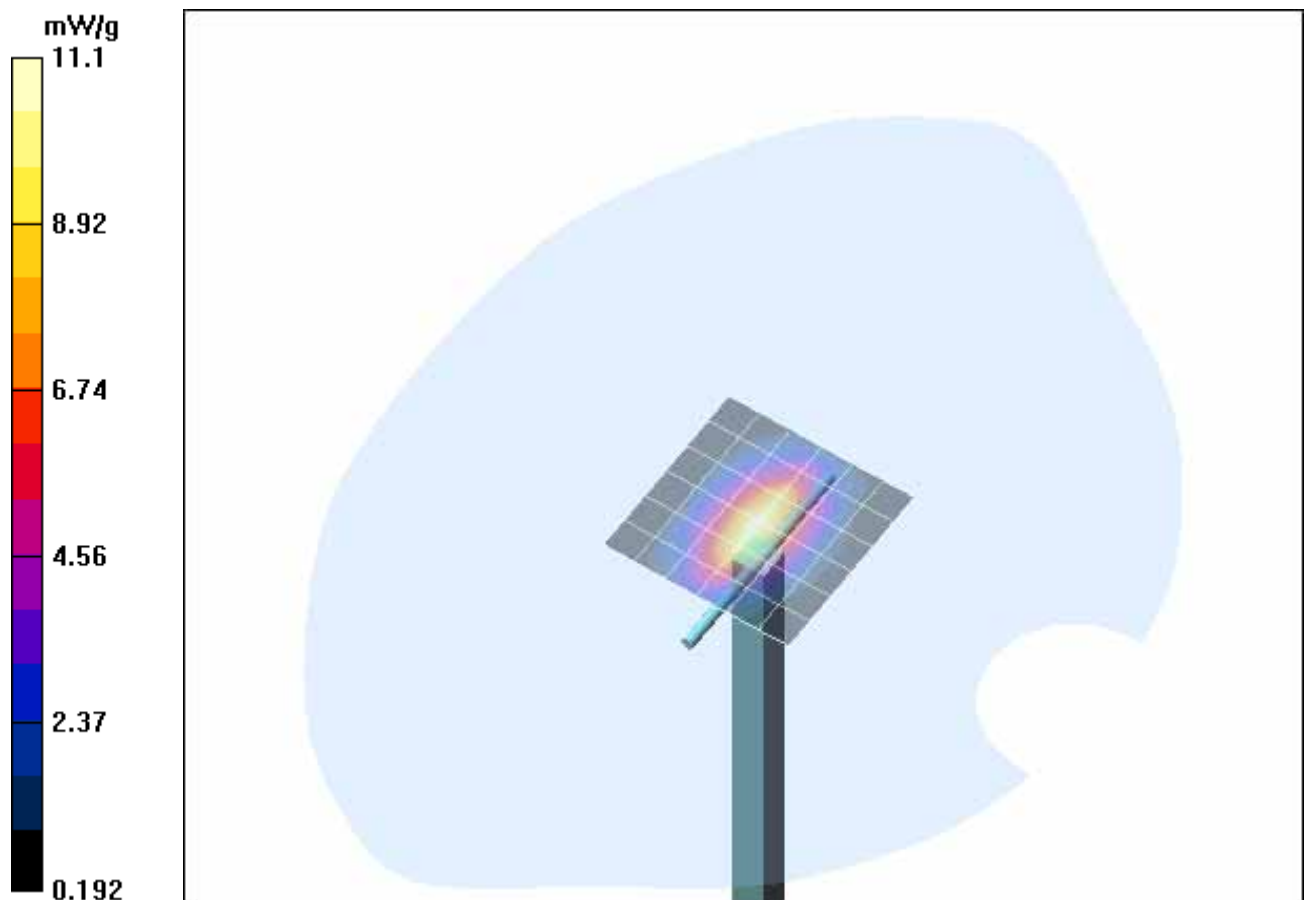
Fig. 11: Validation measurement 1900 MHz body (January 03, 2006), coarse grid. Ambient Temperature: 21.2° C, Liquid Temperature: 20.5° C.
