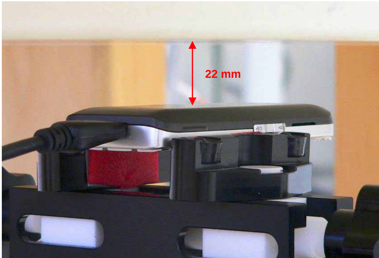
Fig. 26: Body worn configuration, GPRS (Class 10) with data cable, antenna towards the phantom.
