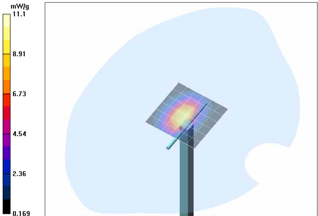
Fig. 10: Validation measurement 1900 MHz Head (December 30, 2005), coarse grid. Ambient Temperature: 20.9° C, Liquid Temperature: 20.1° C.
