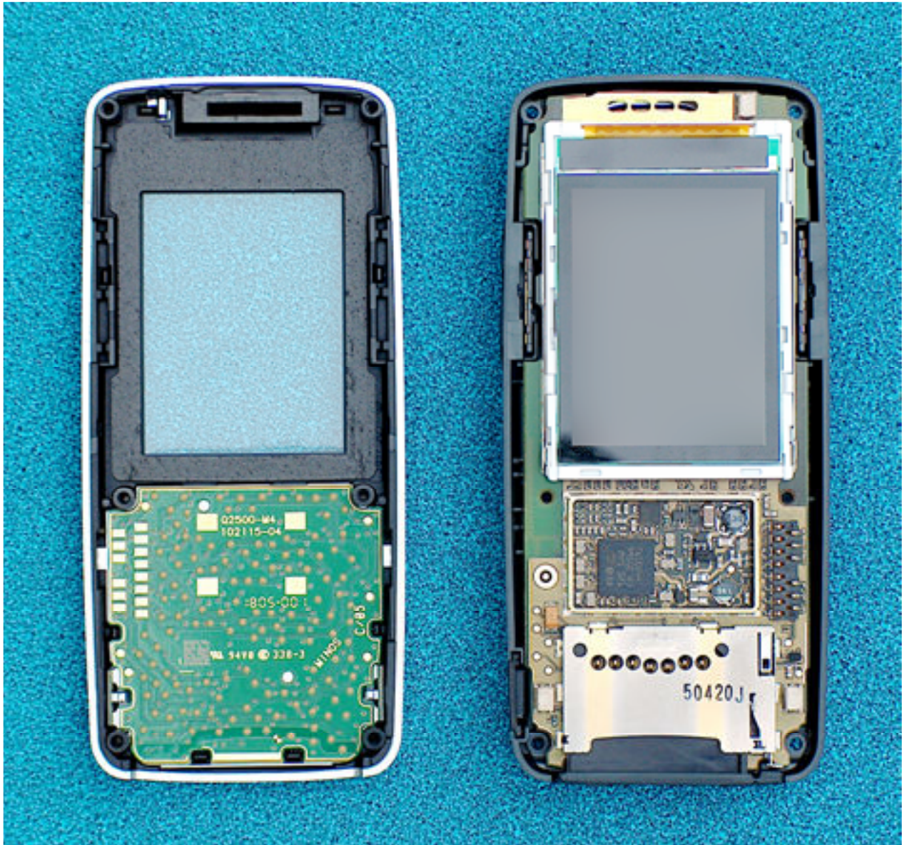
S75 Keypad & Front Cover Disassembly Step 2
