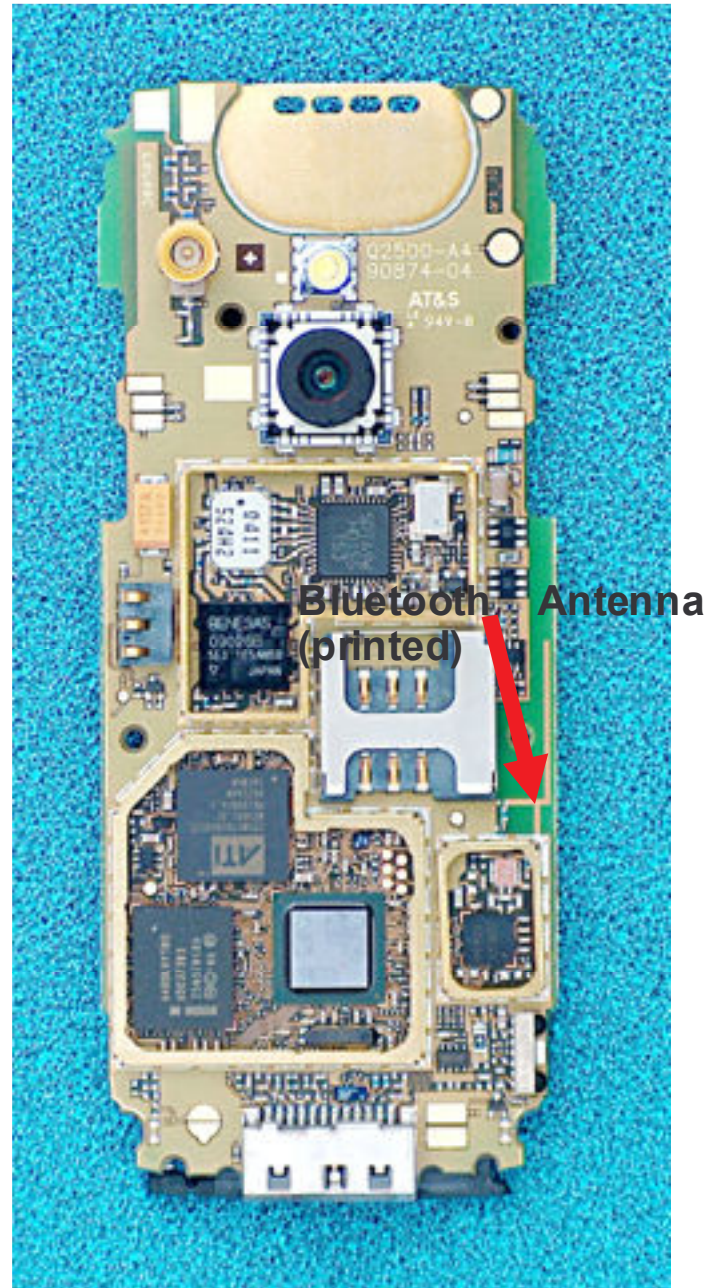
S75 PCB Front & Back Side Disassembly Step 4
