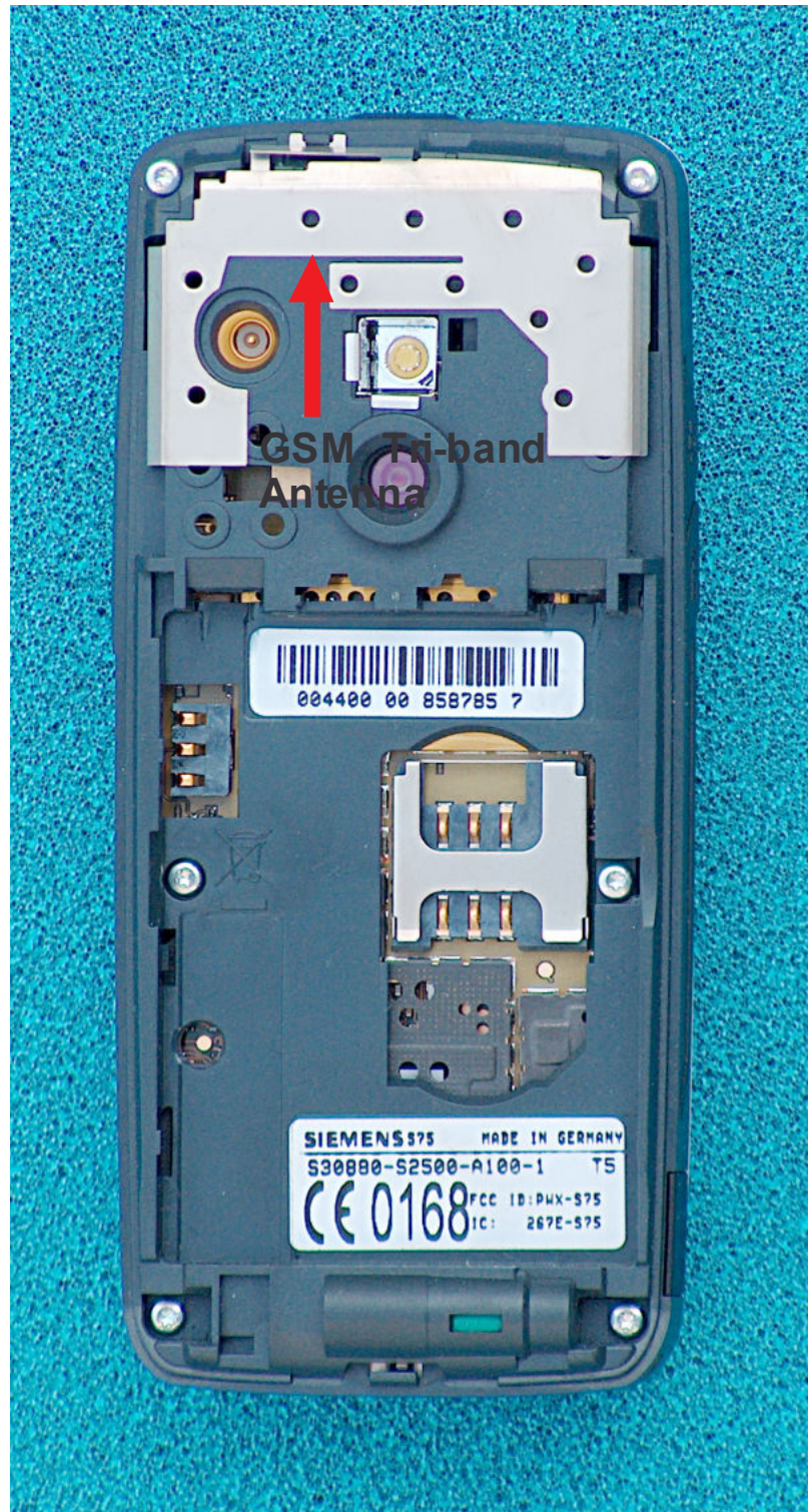
S75 Rear View incl. GSM Antenna
