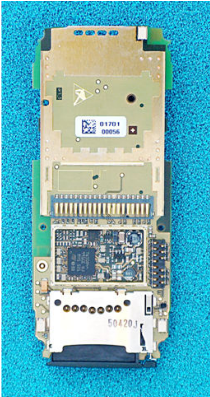
S75 PCB Front & Back Side Disassembly Step 4
