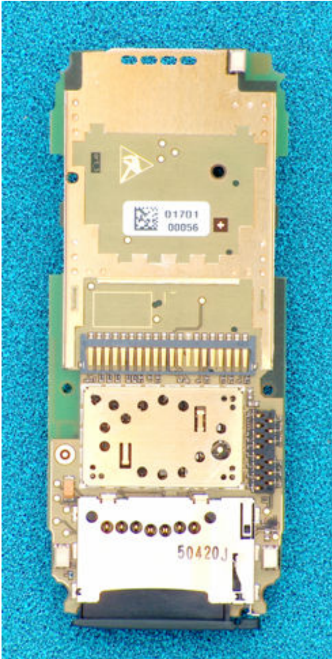
S75 PCB Front & Back Side Disassembly Step 3
