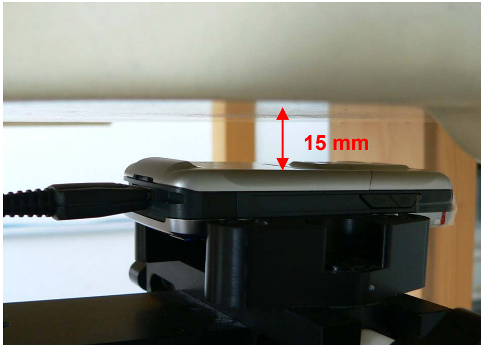
Fig. 34: Body worn configuration, GPRS (Class 10) with Data cable, antenna towards the phantom.
