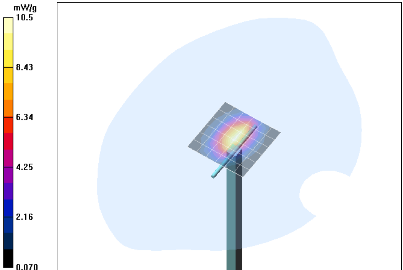
Fig. 11: Validation measurement 1900 MHz Head (July 27, 2005), coarse grid. Ambient Temperature: 22.0° C, Liquid Temperature: 21.5° C.
