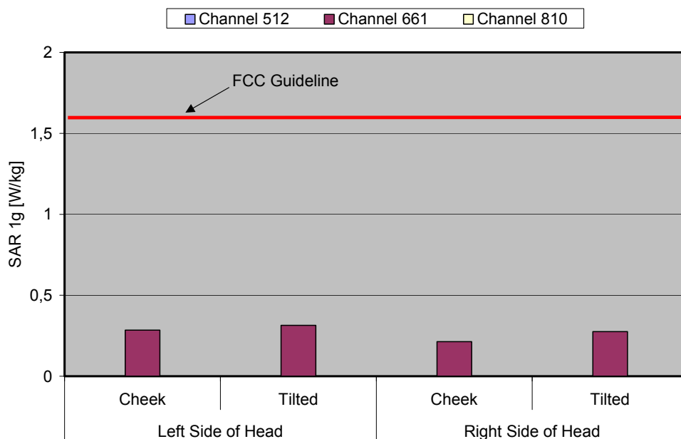
Fig. 9: The measured head phantom SAR values for the Siemens S75 with Flash for PCS 1900 in comparison to the FCC exposure limit.
