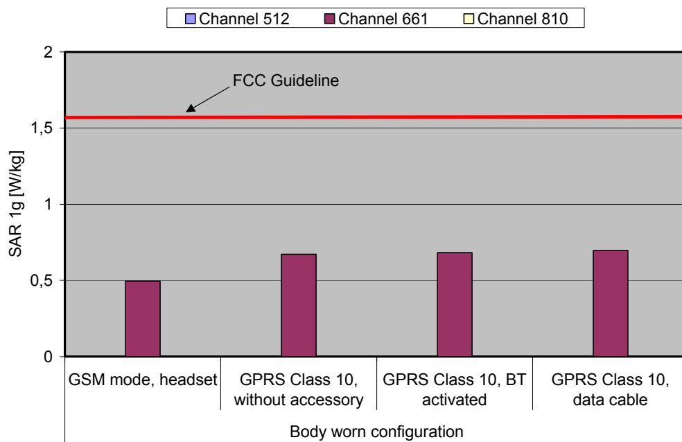
Fig. 10: The measured SAR values in body-worn configuration for the Siemens S75 for PCS 1900 in comparison to the FCC exposure limit.
