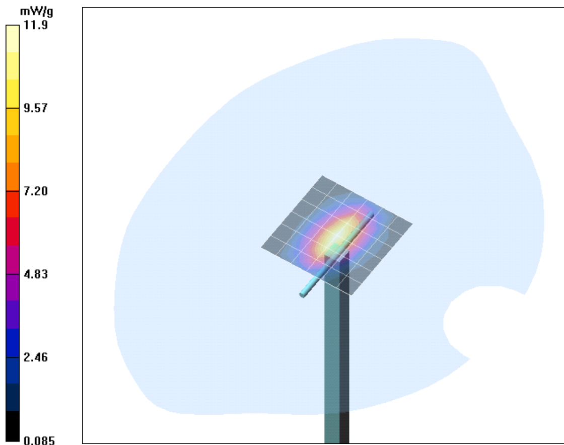
Fig. 12: Validation measurement 1900 MHz body (July 29, 2005), coarse grid. Ambient Temperature: 22.0° C, Liquid Temperature: 21.5° C.
