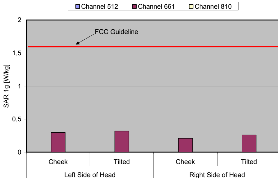
Fig. 8: The measured head phantom SAR values for the Siemens S75 for PCS 1900 in comparison to the FCC exposure limit.
