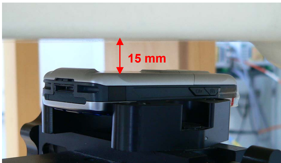
Fig. 33: Body worn configuration, GPRS (Class 10) without accessory and with Bluetooth respectively, antenna towards the phantom.
