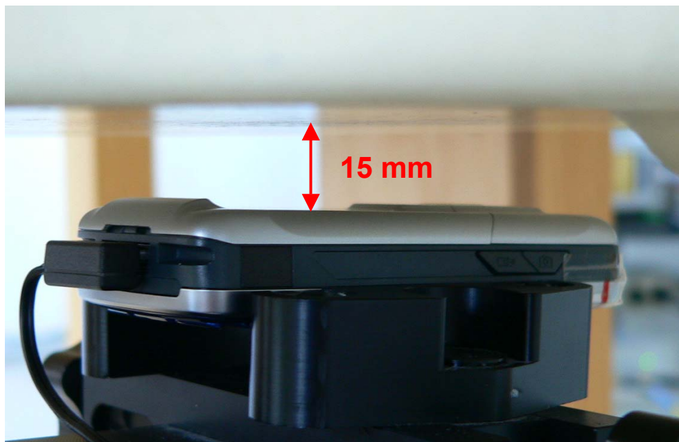
Fig. 32: Body worn configuration, GSM with headset, antenna towards the phantom.
