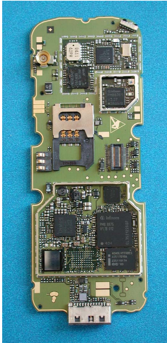
SK65 PCB Shields Removed
