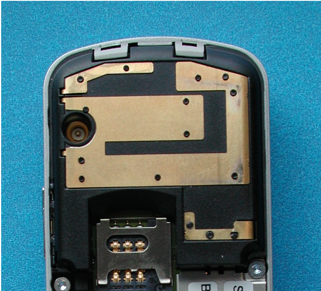
SK65 Tri-Band Antenna
