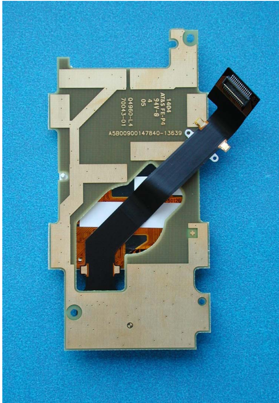
SK65 LCD Board Back View
