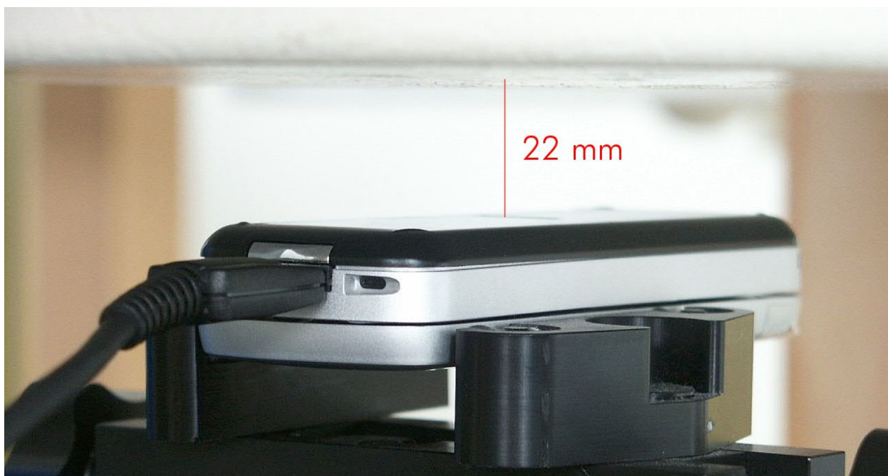
Fig. 23: Body worn configuration, GPRS mode (2 TX slot) with data cable, antenna towards the phantom.
