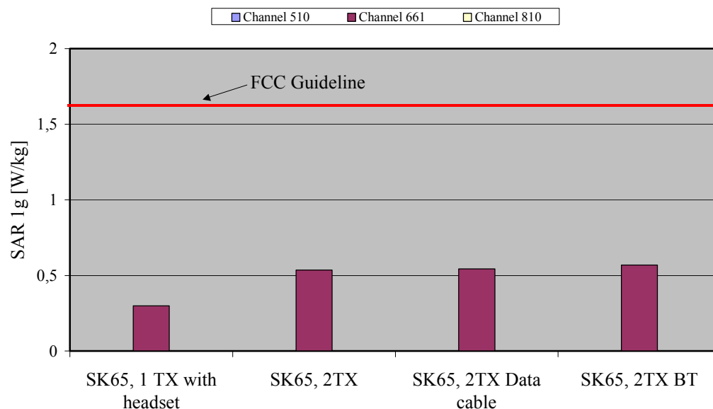
Fig. 9: The measured SAR values in body-worn configuration for the Siemens SK 65 for PCS 1900 (1 TX slot and 2TX slots, gap = 22 mm) in comparison to the FCC exposure limit.
