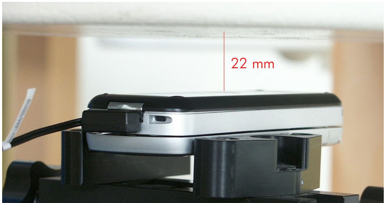
Fig. 22: Body worn configuration, GSM mode (1 TX ) with headset, antenna towards the phantom.
