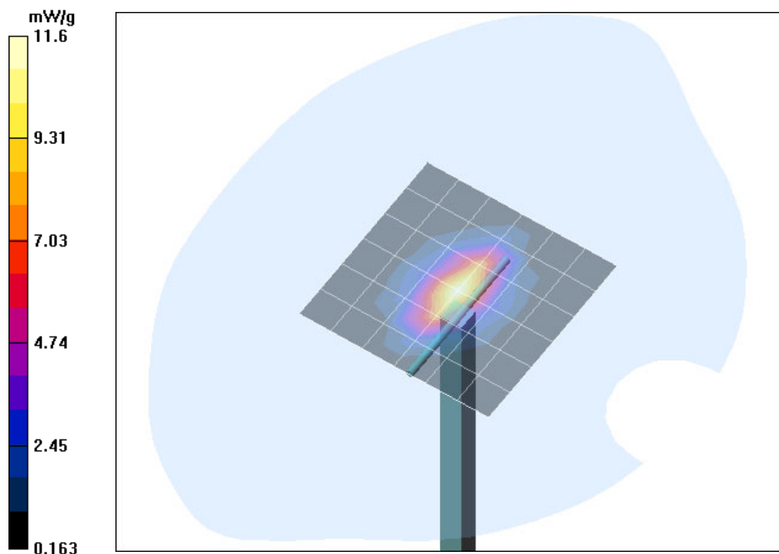
Fig. 11: Validation measurement 1900 MHz body (July 08, 2004), coarse grid. Ambient Temperature: 21.5° C, Liquid Temperature: 20.5° C.
