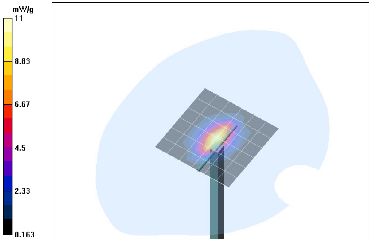
Fig. 10: Validation measurement 1900 MHz Head (July 06, 2004), coarse grid. Ambient Temperature: 20.8° C, Liquid Temperature: 20.3° C.
