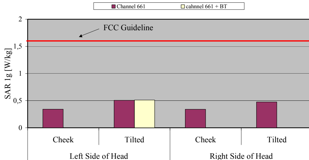
Fig. 8: The measured head phantom SAR values for the Siemens SK 65 for PCS 1900 in comparison to the FCC exposure limit.
