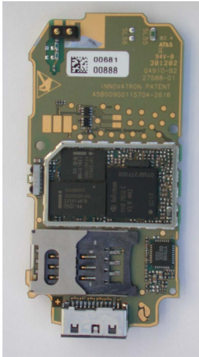
SL55 board without shielding, side2
