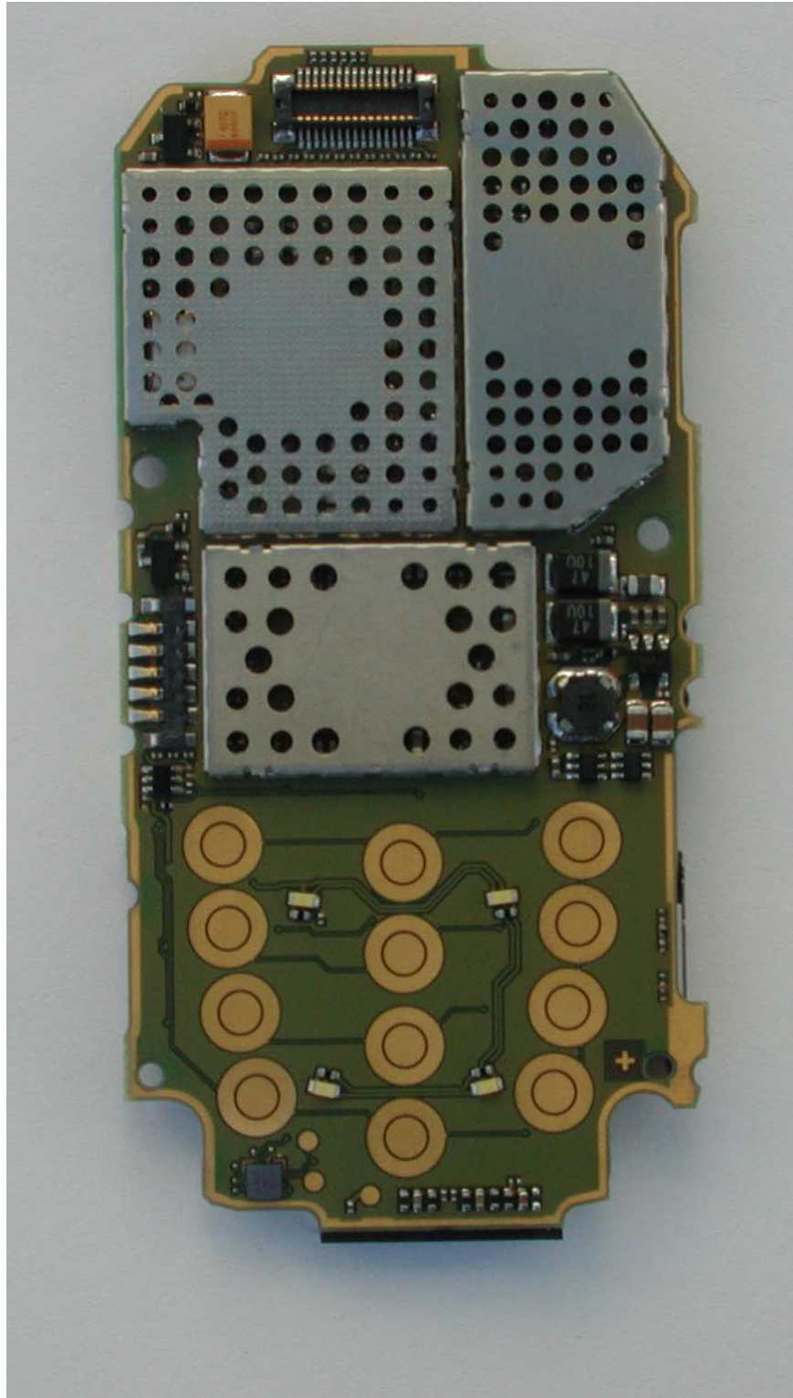
SL55 board with shielding, side1
