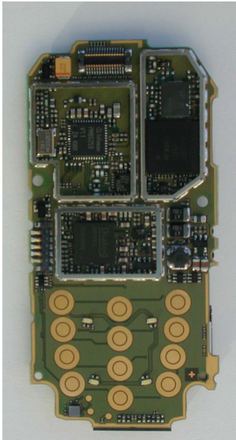
SL55 board without shielding, side1
