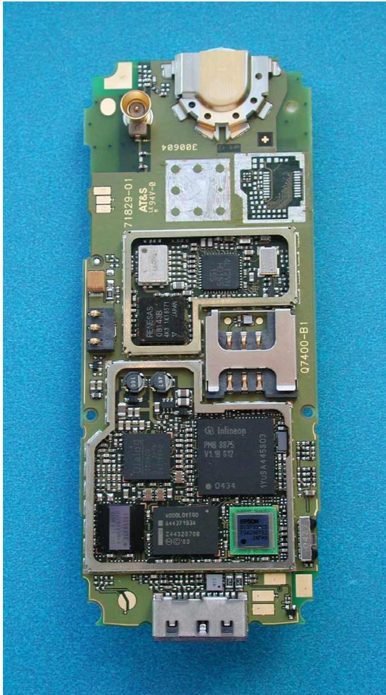
SP65 PCB Rear View Shields Removed
