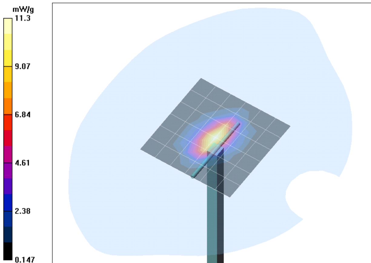
Fig. 11: Validation measurement 1900 MHz body (February 02, 2005), coarse grid. Ambient Temperature: 21.9° C, Liquid Temperature: 21.1° C.
