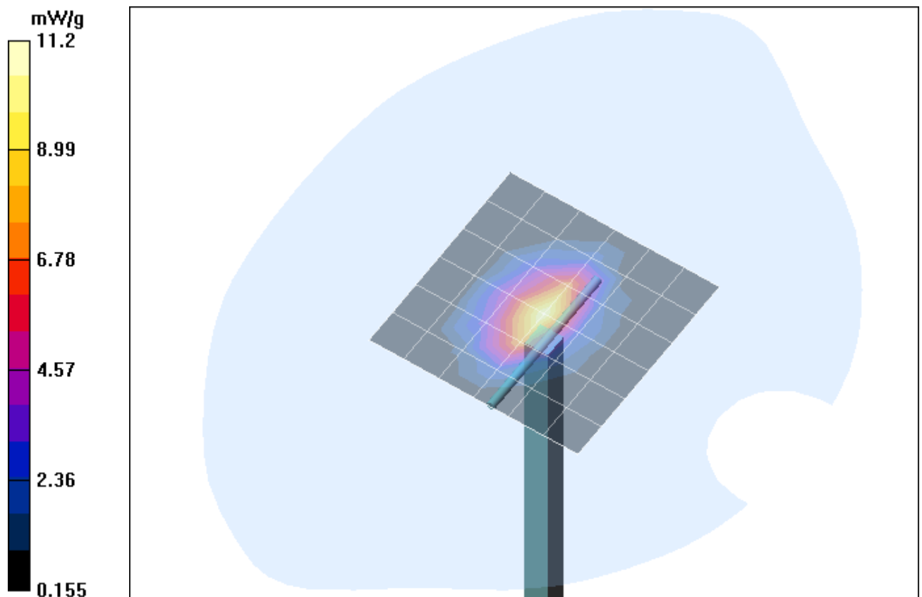
Fig. 10: Validation measurement 1900 MHz Head (January 31, 2005), coarse grid. Ambient Temperature: 21.8° C, Liquid Temperature: 20.9° C.
