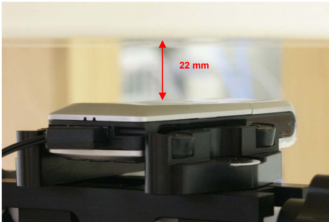
Fig. 20: Body worn configuration, GSM mode with headset, antenna towards the phantom, distance = 22 mm.
