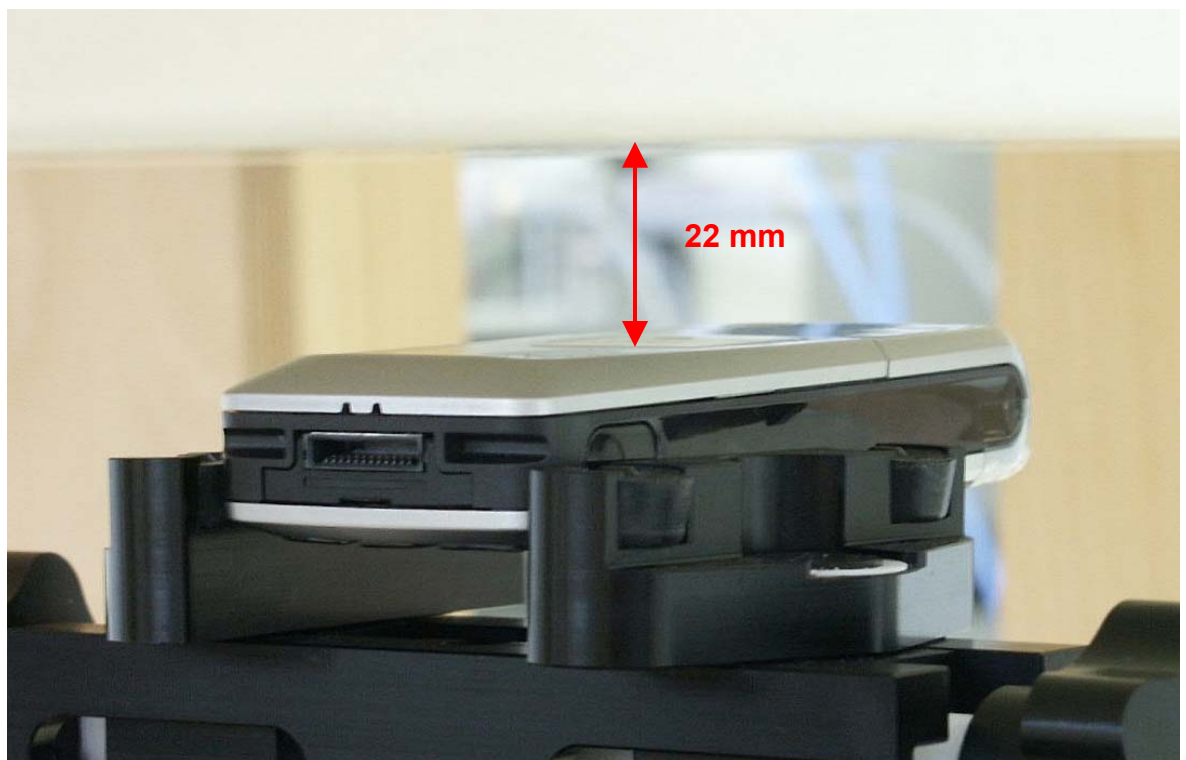
Fig. 21: Body worn configuration, GPRS mode (Class 10), antenna towards the phantom.
