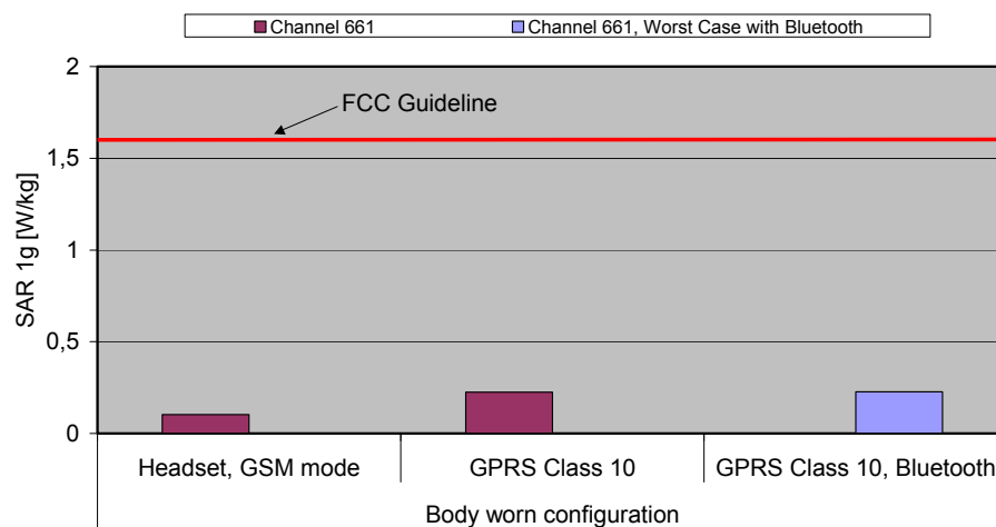
Fig. 9: The measured SAR values in body-worn configuration for the Siemens SP65 for PCS 1900 in comparison to the FCC exposure limit.
