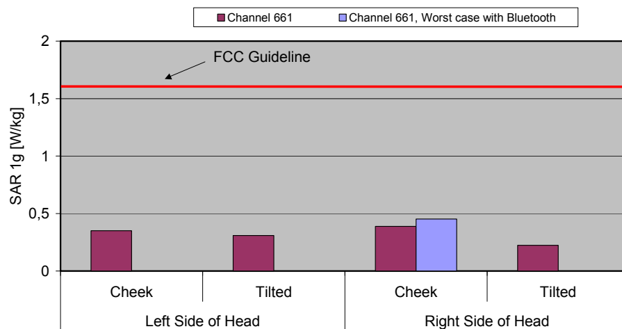
Fig. 8: The measured head phantom SAR values for the Siemens SP65 for PCS 1900 in comparison to the FCC exposure limit.
