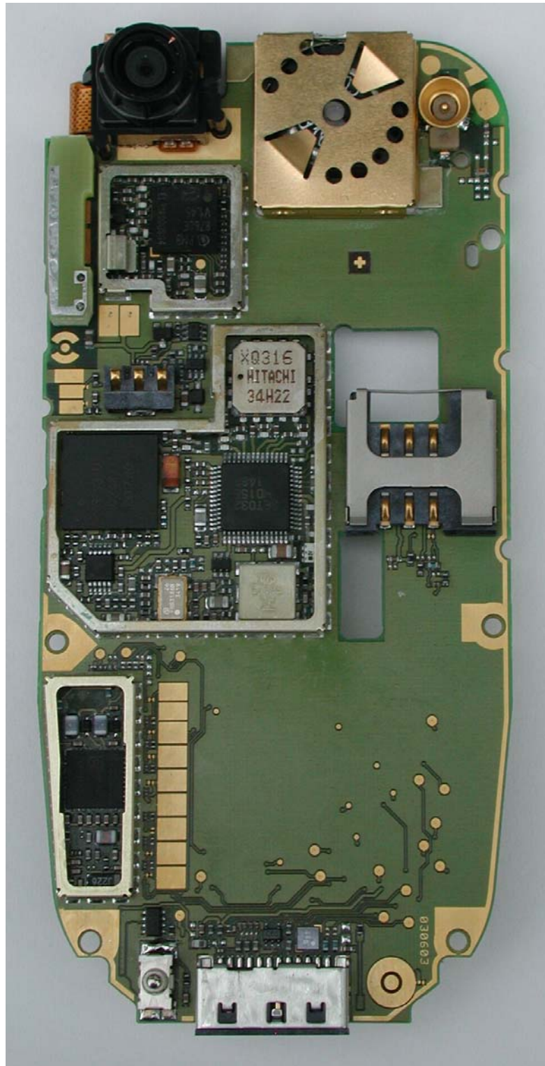
SX1 Main Board without Shielding (Side 2)
