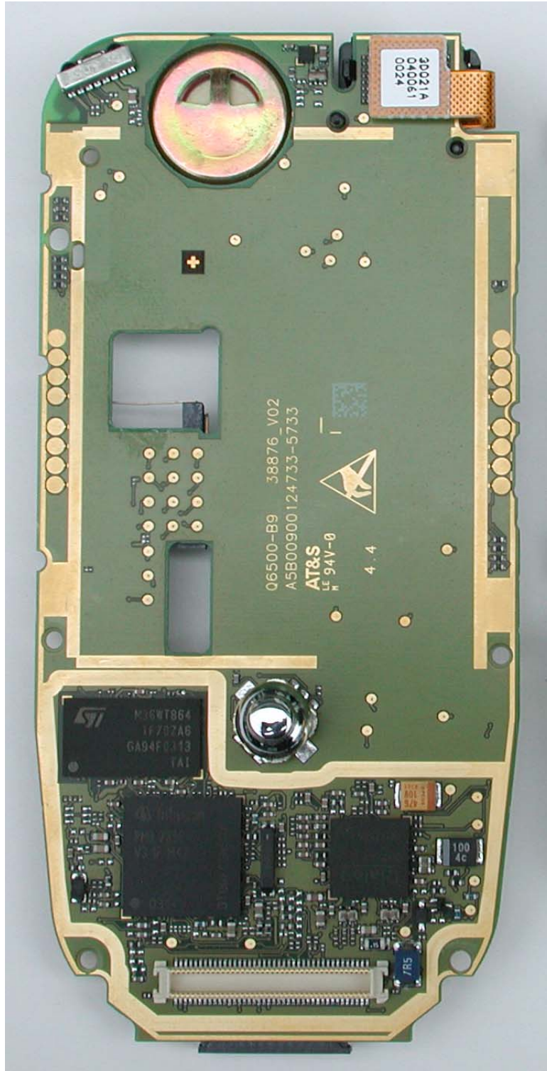
SX1 Main Board (Side 1)
