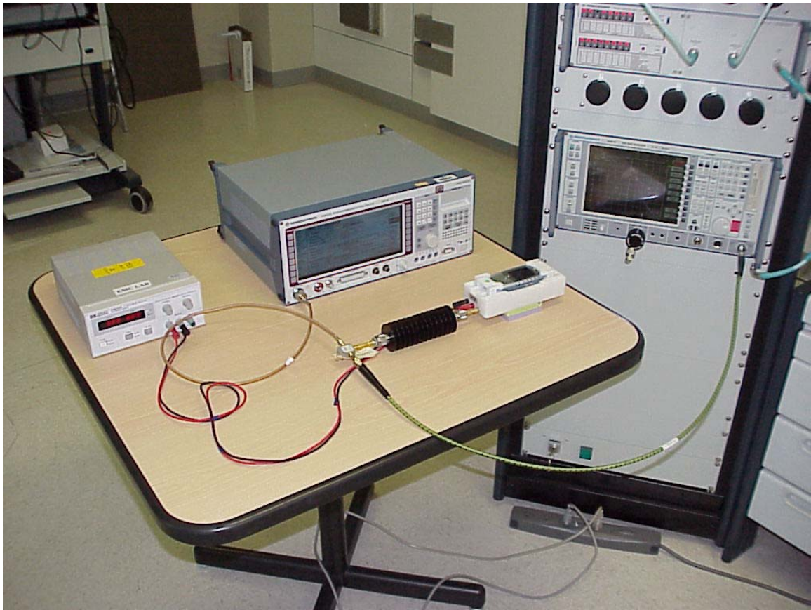
Test setup – conducted measurements GSM 1900
