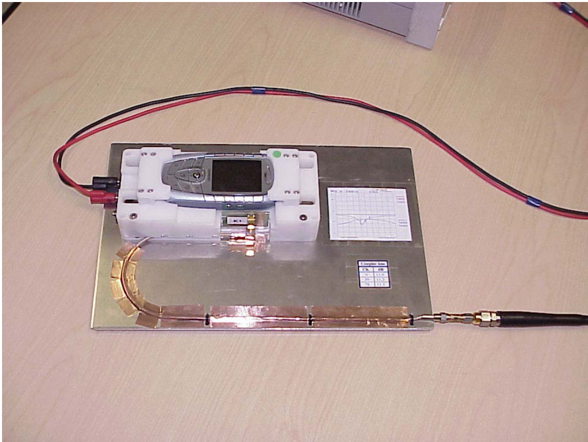
Test setup – conducted measurements Bluetooth
