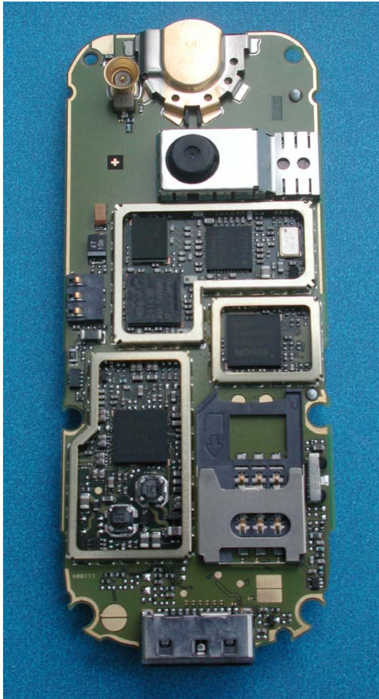
C65 PCB Back View Shields Removed
