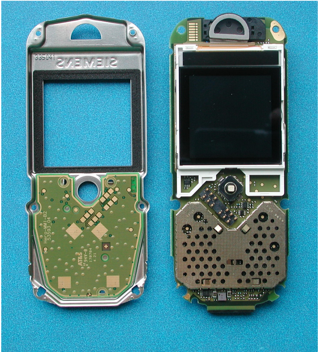
C65 Disassembly step 2
