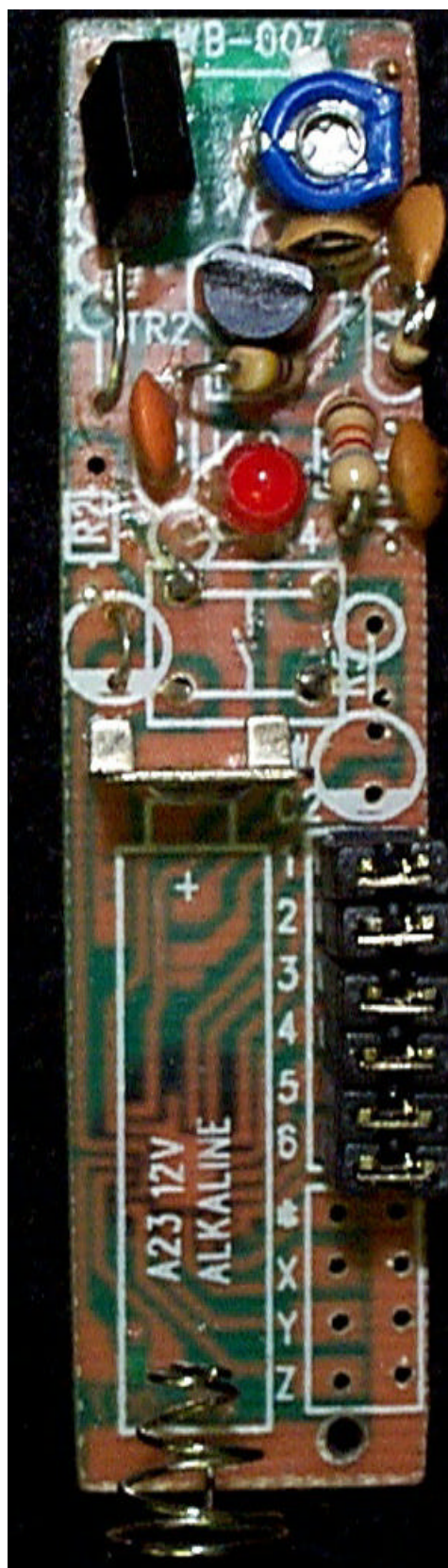
Photo 3. Internal View, Top Side
