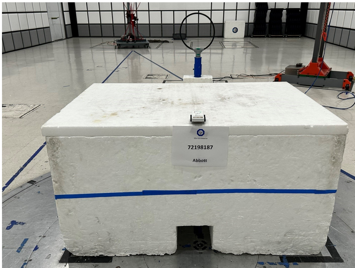
Radiated Emissions Test Setup (9kHz to 30MHz)
