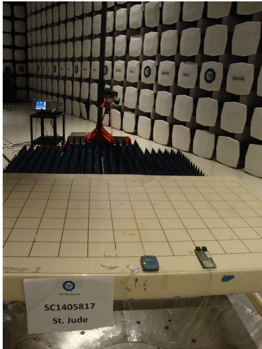
Figure 4(1GHz-18GHz Back Picture)
