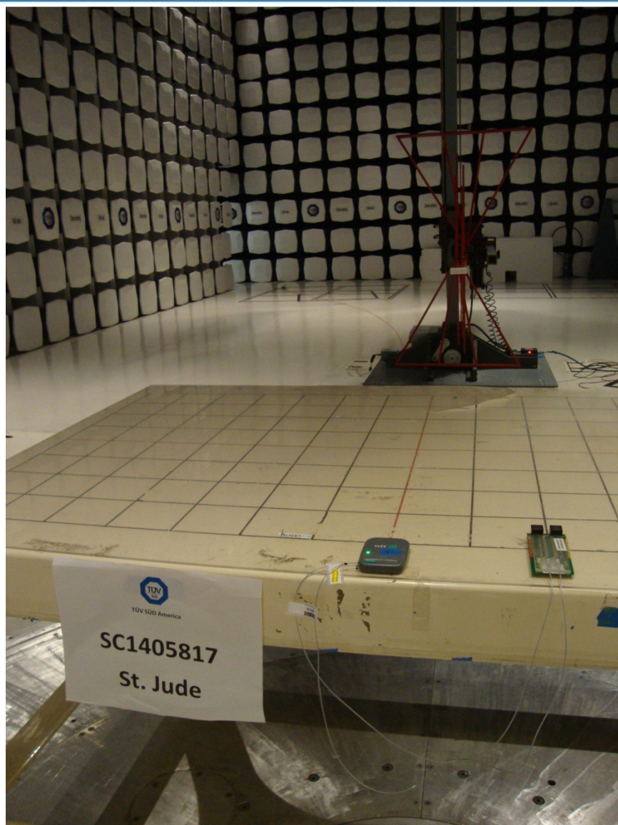
Figure 2(30MHz-1GHz Back Picture)
