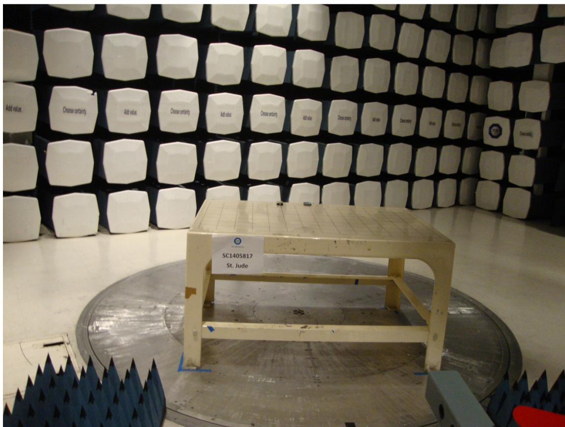
Figure 3(1GHz-18GHz Front Picture)
