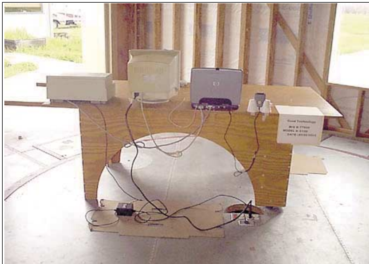
Radiated Emissions - Back View - USB Vertical
