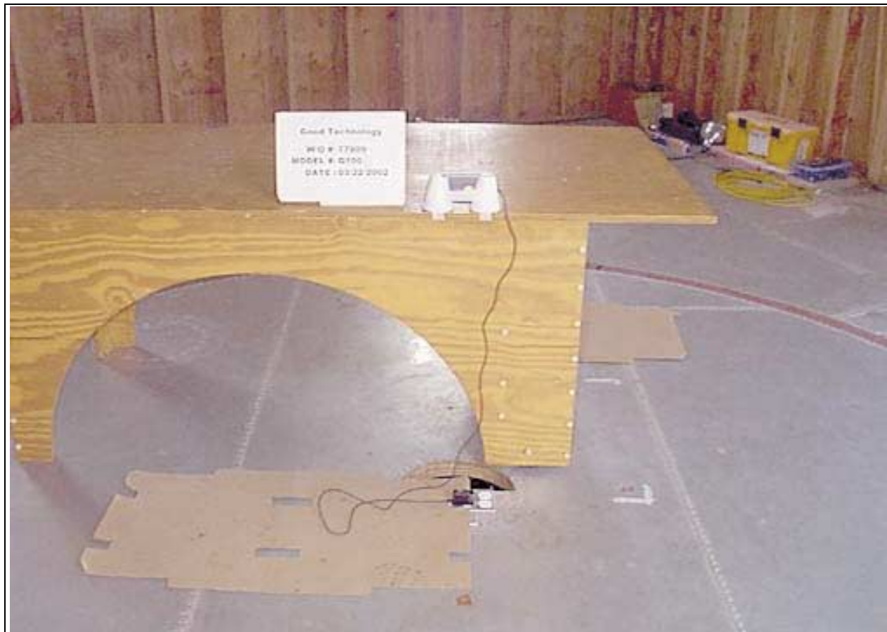
Radiated Emissions - Back View - AC Adapter Horizontal
