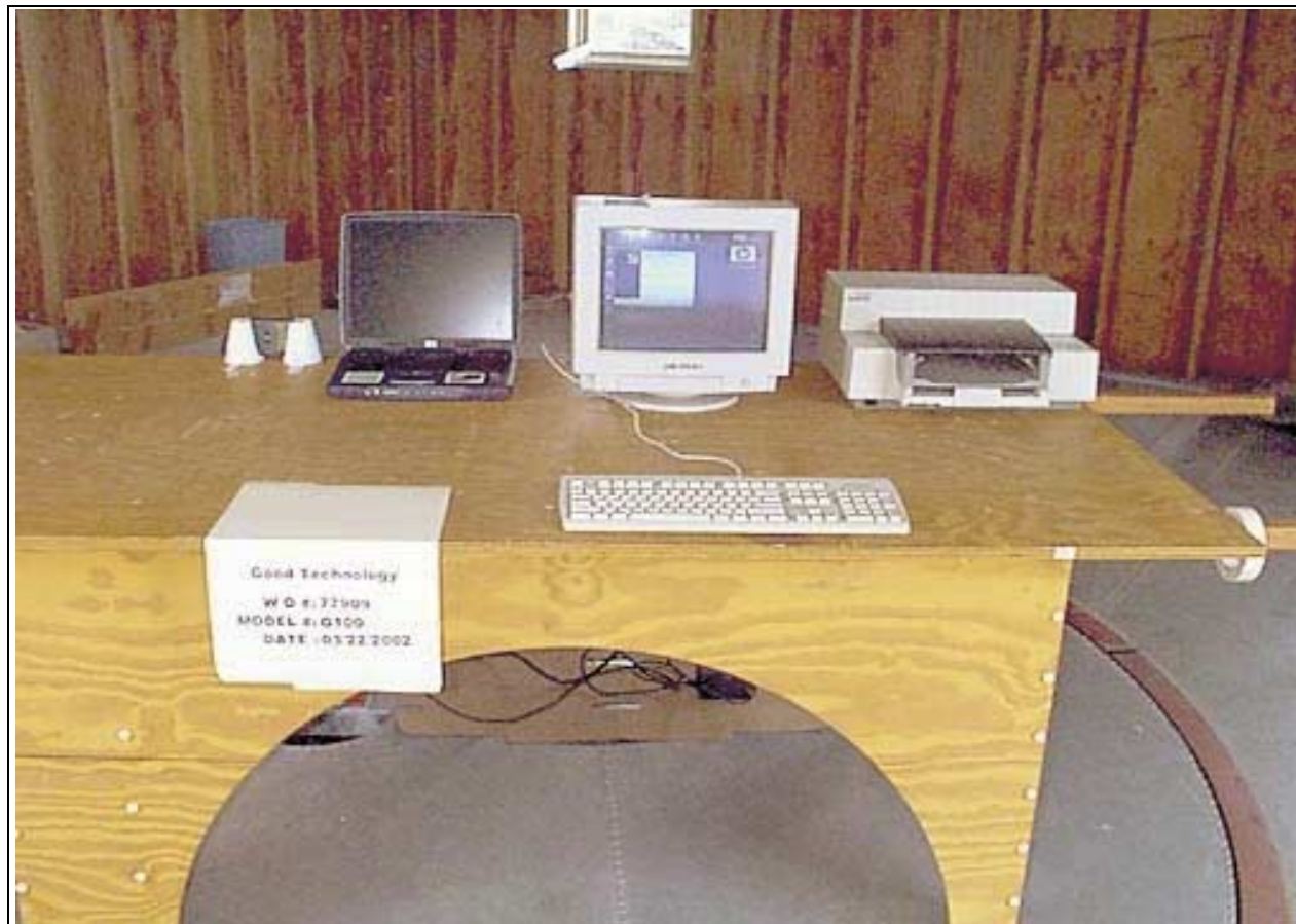
Radiated Emissions - Front View - USB Horizontal
