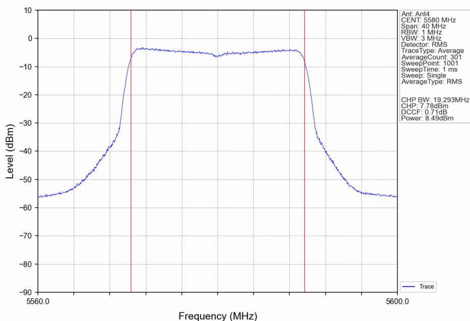
802.11ax(HEW20)_MCH_5580MHz_RU26_Right_Ant4_NTNV
