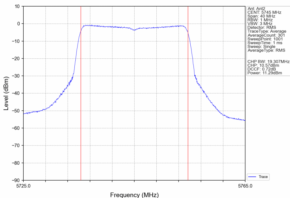
802.11ax(HEW20)_LCH_5745MHz_RU26_Right_Ant2_NTNV
