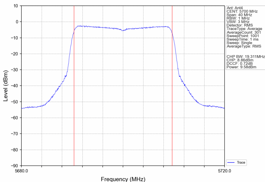
802.11ax(HEW20)_HCH_5700MHz_RU26_Mid_Ant4_NTNV
