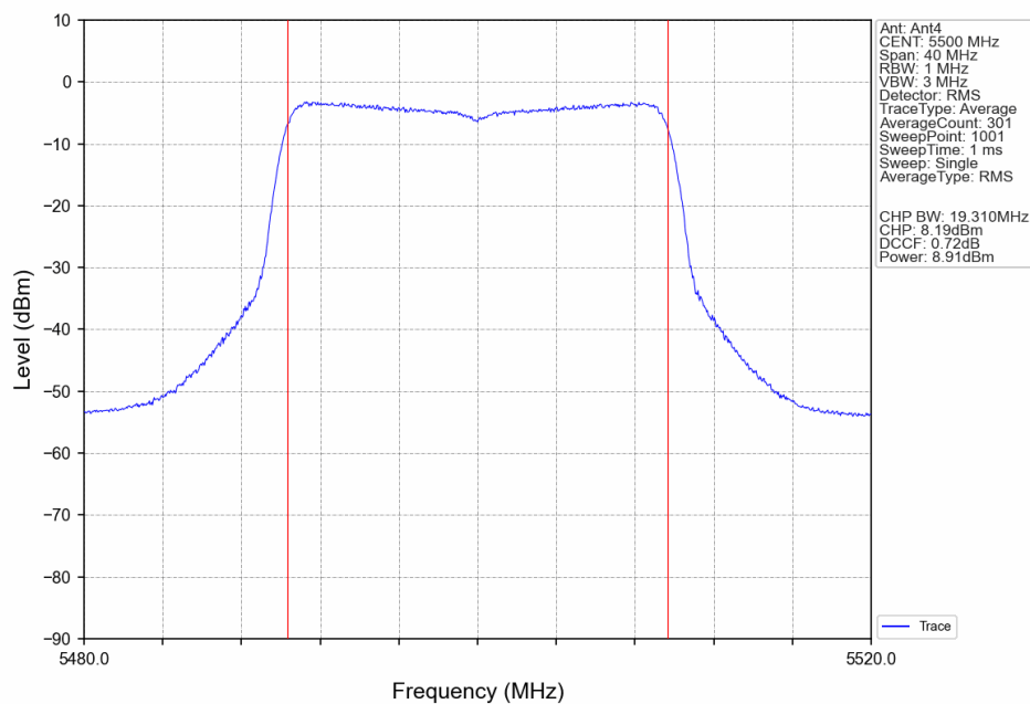
802.11ax(HEW20)_LCH_5500MHz_RU26_Right_Ant4_NTNV
