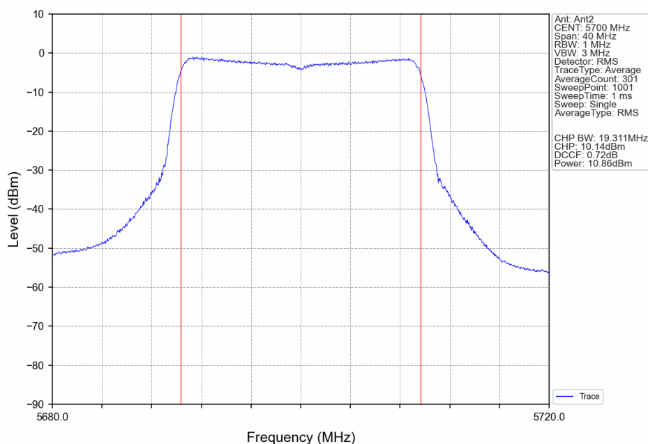
802.11ax(HEW20)_HCH_5700MHz_RU242_Left_Ant2_NTNV
