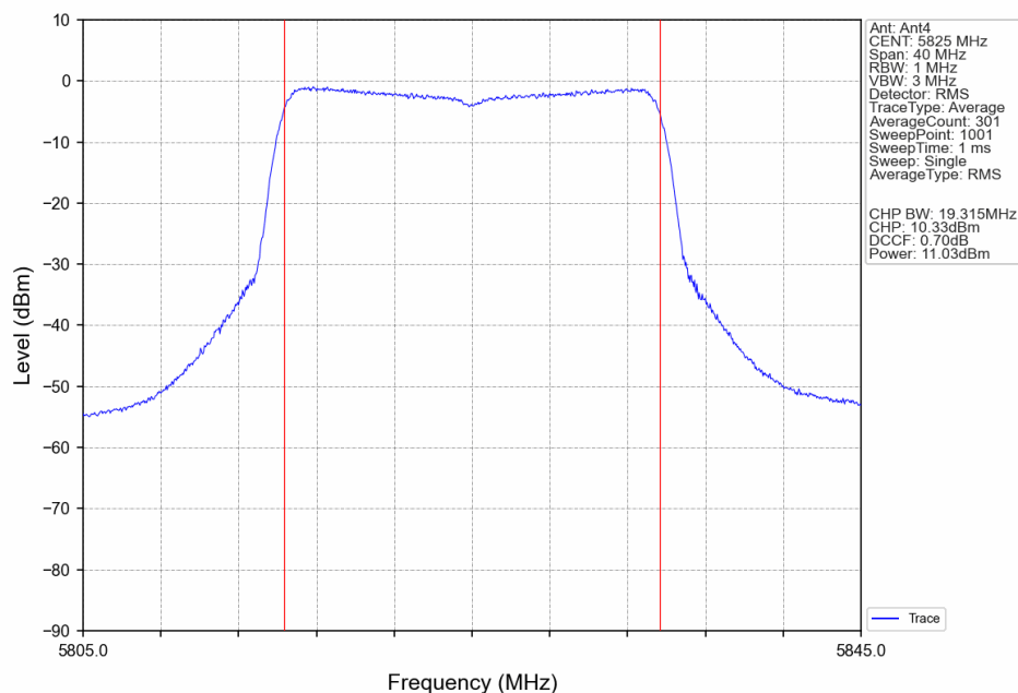
802.11ax(HEW20)_HCH_5825MHz_RU26_Mid_Ant4_NTNV
