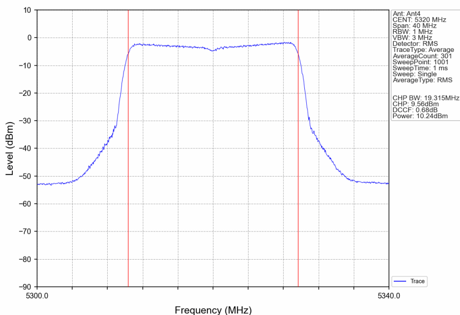
802.11ax(HEW20)_HCH_5320MHz_RU26_Right_Ant4_NTNV
