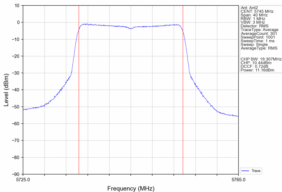
802.11ax(HEW20)_LCH_5745MHz_RU26_Left_Ant2_NTNV
