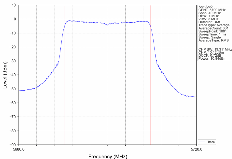
802.11ax(HEW20)_HCH_5700MHz_RU26_Right_Ant2_NTNV
