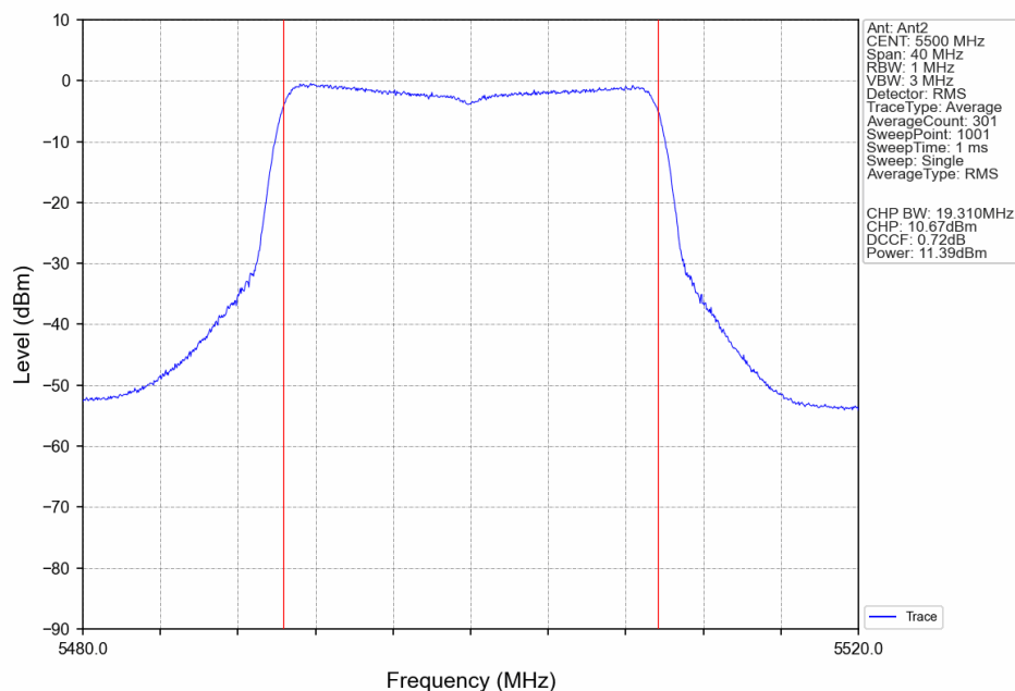
802.11ax(HEW20)_LCH_5500MHz_RU26_Mid_Ant2_NTNV
