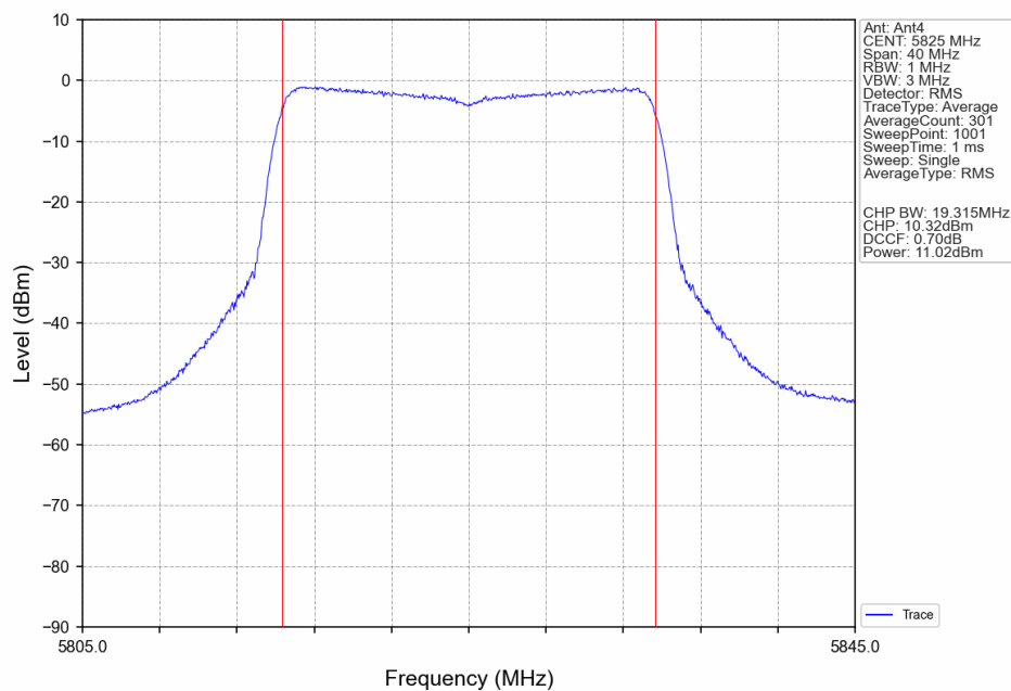
802.11ax(HEW20)_HCH_5825MHz_RU242_Left_Ant4_NTNV
