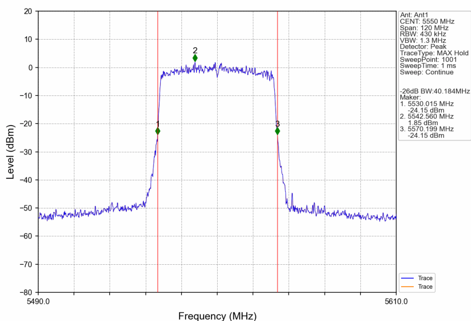
802.11ax(HEW40)_MCH_5550MHz_RU484_Left_Ant1_NTNV
