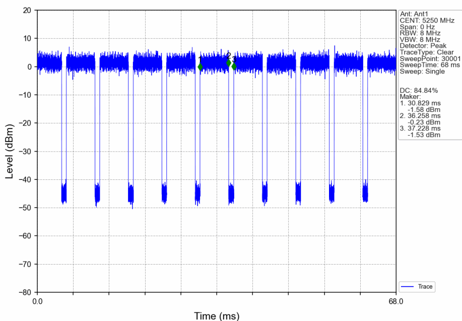
802.11ac(VHT160)_MCH_5250MHz_Ant1_NTNV
