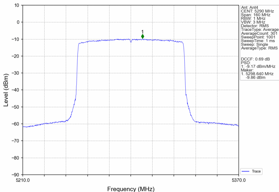
802.11ax(HEW80)_MCH_5290MHz_RU26_Mid_MIMO_NTNV
