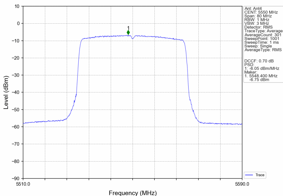
802.11ax(HEW40)_MCH_5550MHz_RU26_Right_Ant4_NTNV
