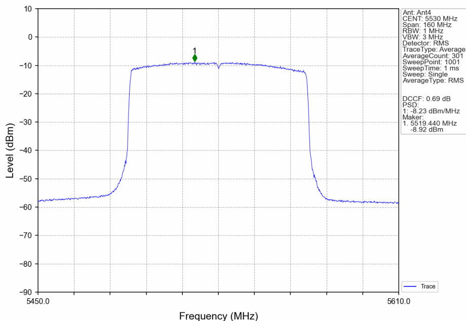
802.11ax(HEW80)_LCH_5530MHz_RU26_Mid_MIMO_NTNV
