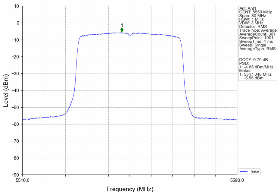
802.11ax(HEW40)_MCH_5550MHz_RU484_Left_Ant1_NTNV
