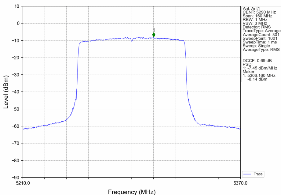
802.11ax(HEW80)_MCH_5290MHz_RU26_Mid_Ant1_NTNV
