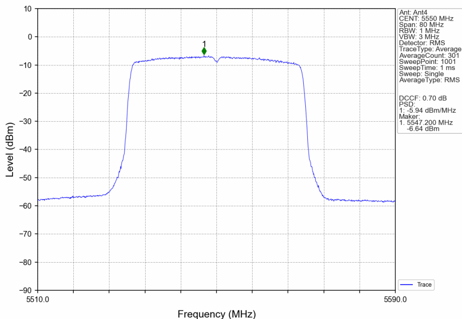
802.11ax(HEW40)_MCH_5550MHz_RU26_Mid_MIMO_NTNV
