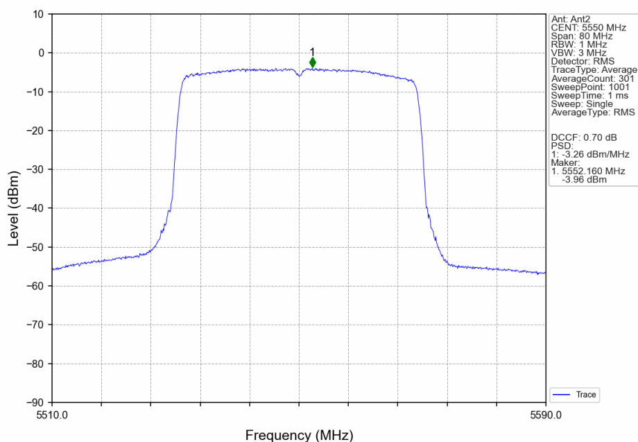
802.11ax(HEW40)_MCH_5550MHz_RU26_Right_Ant2_NTNV
