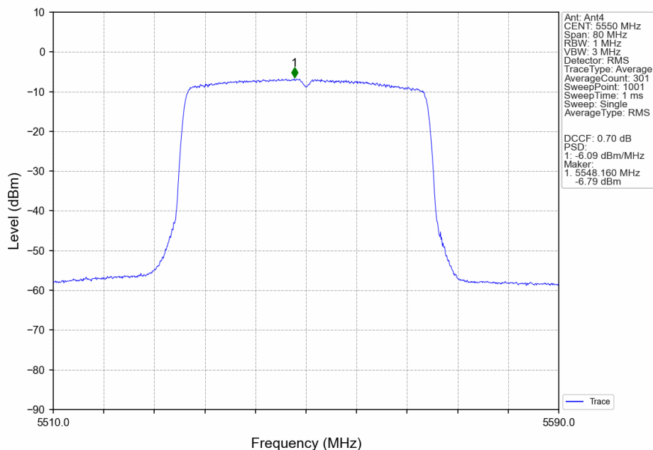
802.11ax(HEW40)_MCH_5550MHz_RU484_Left_MIMO_NTNV
