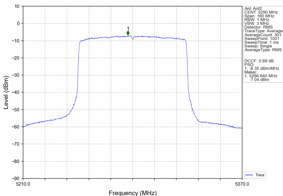
802.11ax(HEW80)_MCH_5290MHz_RU26_Right_Ant2_NTNV
