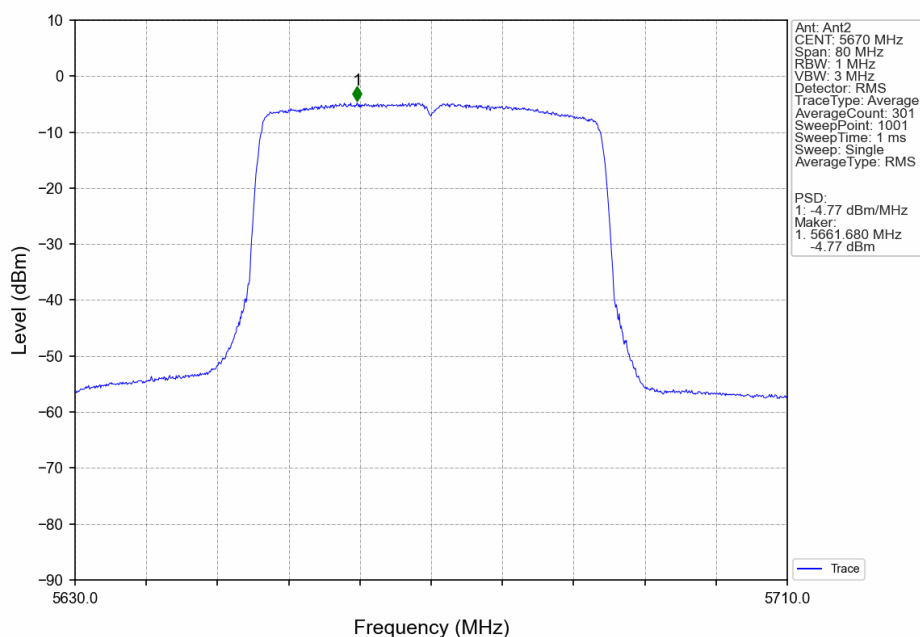
802.11ax(HEW40)_HCH_5670MHz_RU26_Right_Ant2_NTNV
