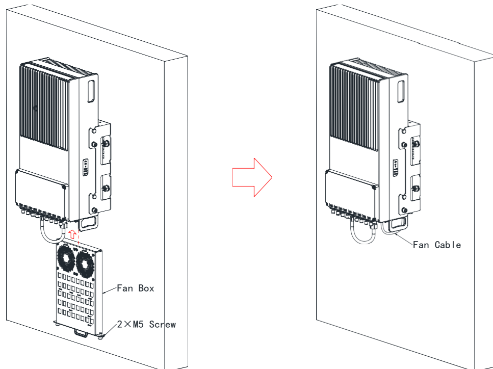
Figure 8 Fan Installation
