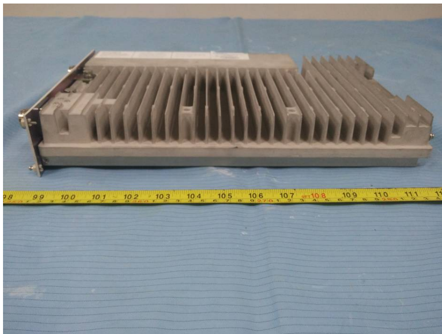
EUT (RF Unit) – Right View
