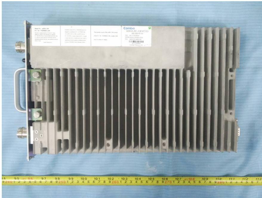
EUT (RF Unit) – Front View
