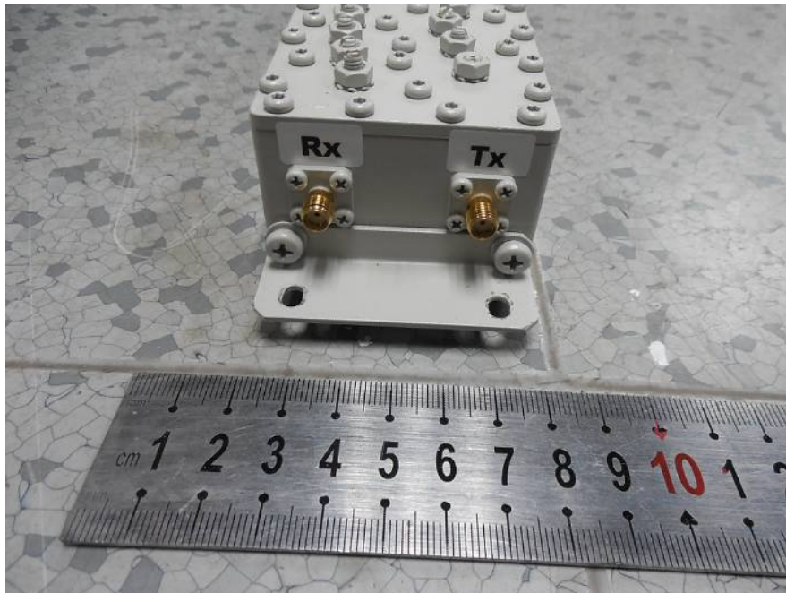
EUT –Duplexer back view
