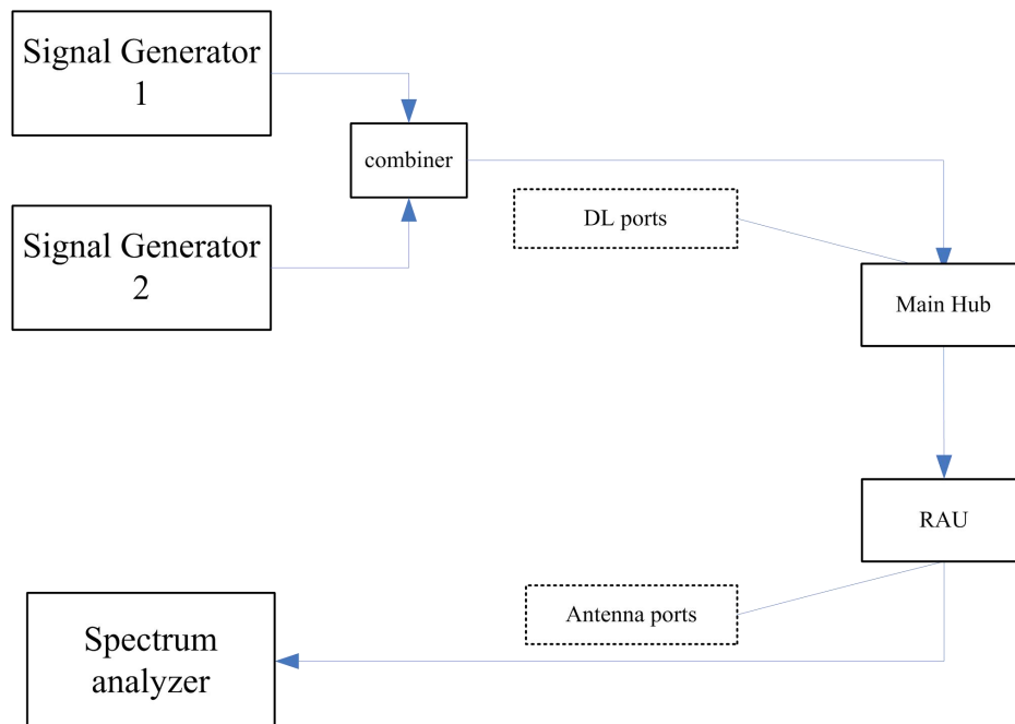
Figure 4: Downlink Intermodulation Configuration
