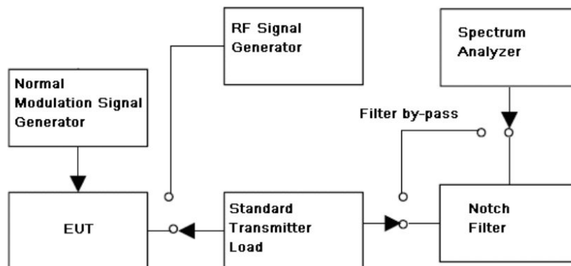
Figure 4: Downlink Intermodulation Configuration
