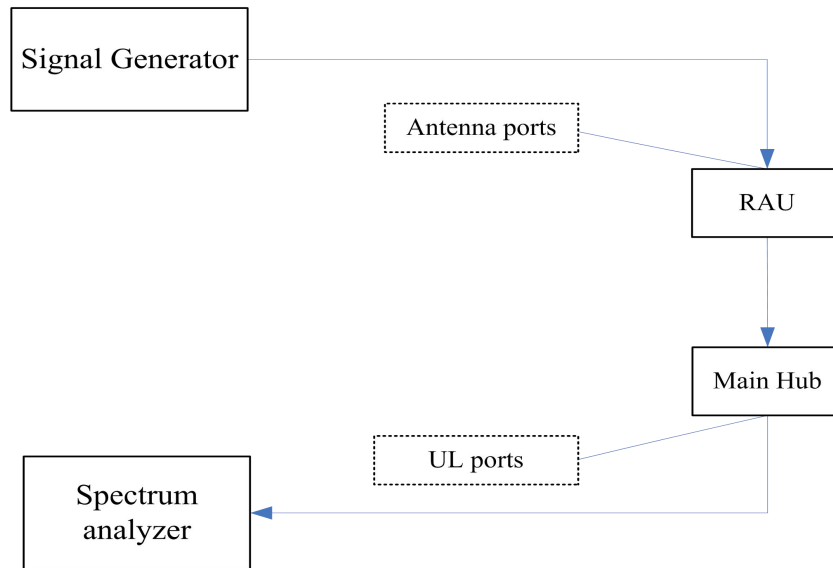
Figure 7: Uplink Out of Band Rejection Configuration
