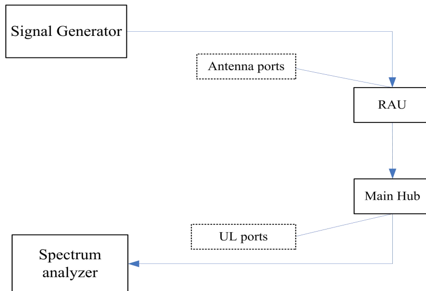
Figure 3: Uplink Band Edge Configuration
