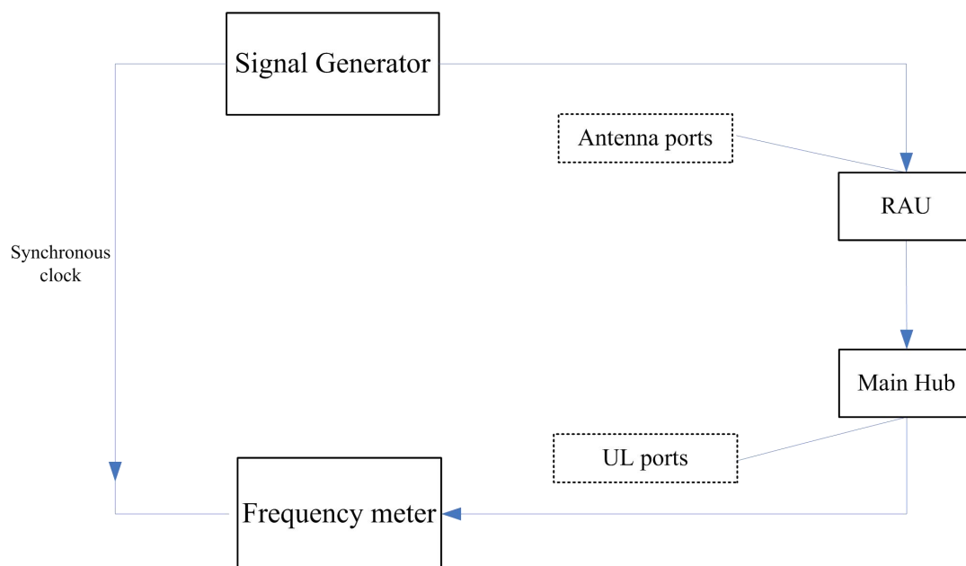
Figure 5: Uplink Frequency Stability Configuration
