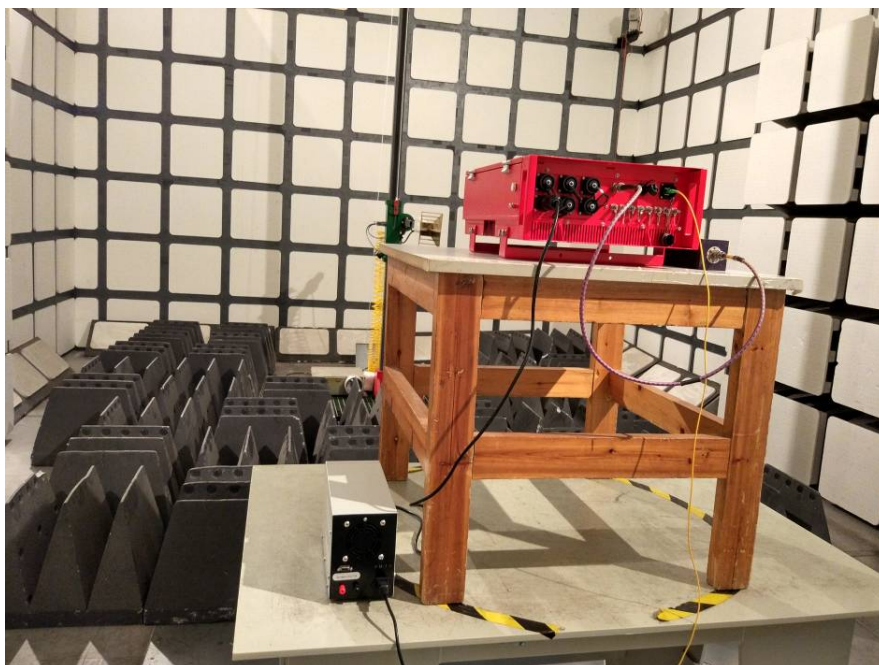
Transmitting Radiated Emissions Tested – Rear View (Above 1 GHz)
